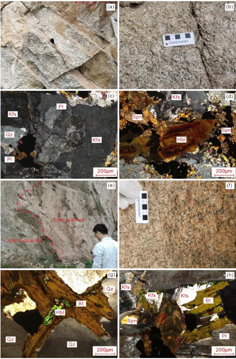
Figure 3: Representative field photographs and photomicrographs of the LP and XP in the western section of North Qinling Orogen. Kfs = K-feldspar, Pl = Plagioclase, Bt = biotite, Qz = Quartz, Hbl = Hornblende, Spn = Sphene.
