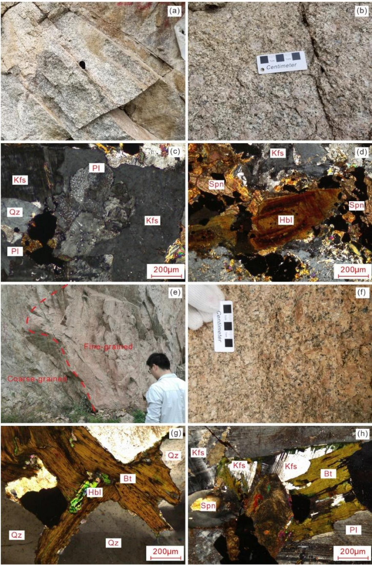
175 Figure 3: Representative field photographs and photomicrographs of the LP and XP in the western section of North Qinling Orogen. Kfs = K-feldspar, Pl = Plagioclase, Bt = biotite, Qz = Quartz, Hbl = Hornblende, Spn = Sphene.
