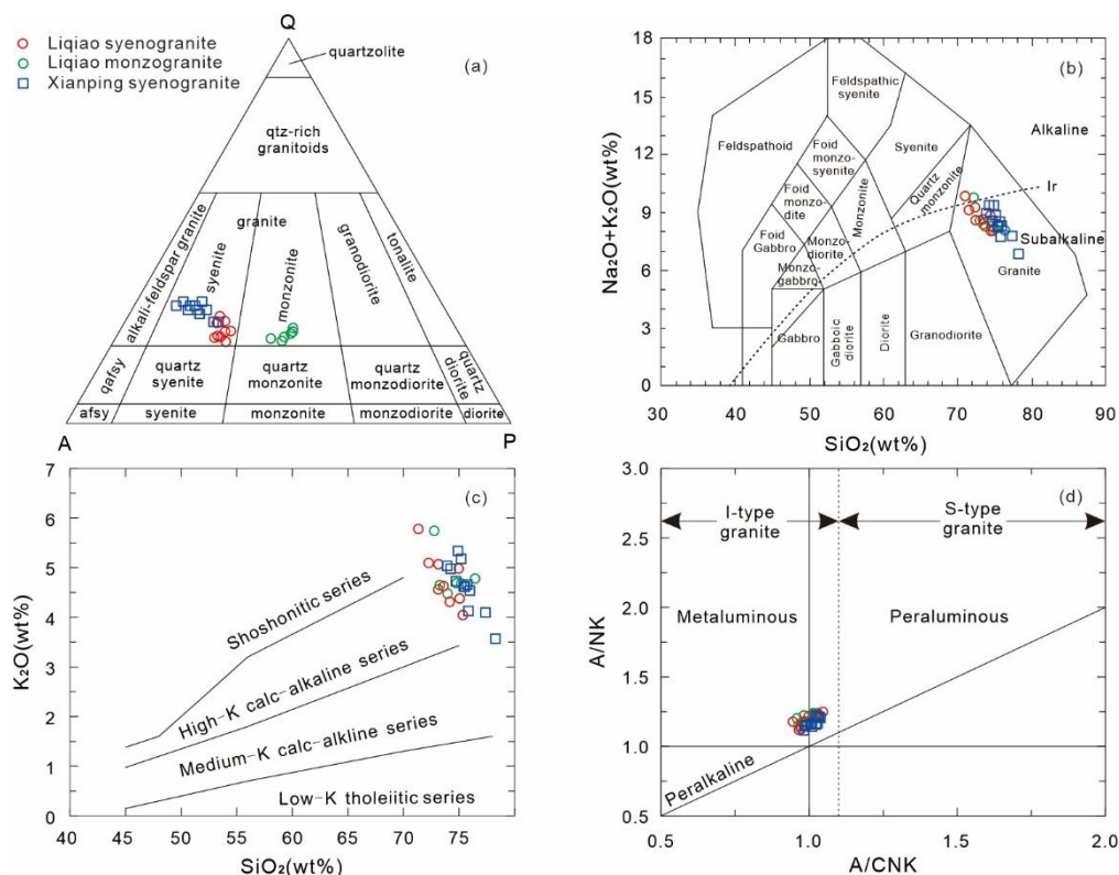
Figure 6: Geochemical plots for rocks of the LP and XP of the western section of North Qinling Orogen: (a) Q-A-P diagram (Streckeisen 1976); (b) TAS classification diagram (Middlemost 1994); (c) K_2O versus SiO_2 diagram (Peccerillo and Taylor, 1976); (d) A/CNK (molar Al_2O_3/[CaO+Na_2O+K_2O] ) versus A/NK (molar Al_2O_3/[Na_2O+K_2O] ) diagram (Maniar and Piccoli, 1989).
