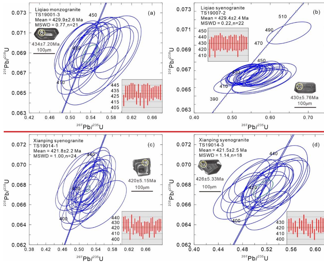
Figure 4: CL image of zircons and the U-Pb zircon concordia diagrams from the LP and XP in the western section of NQO.
