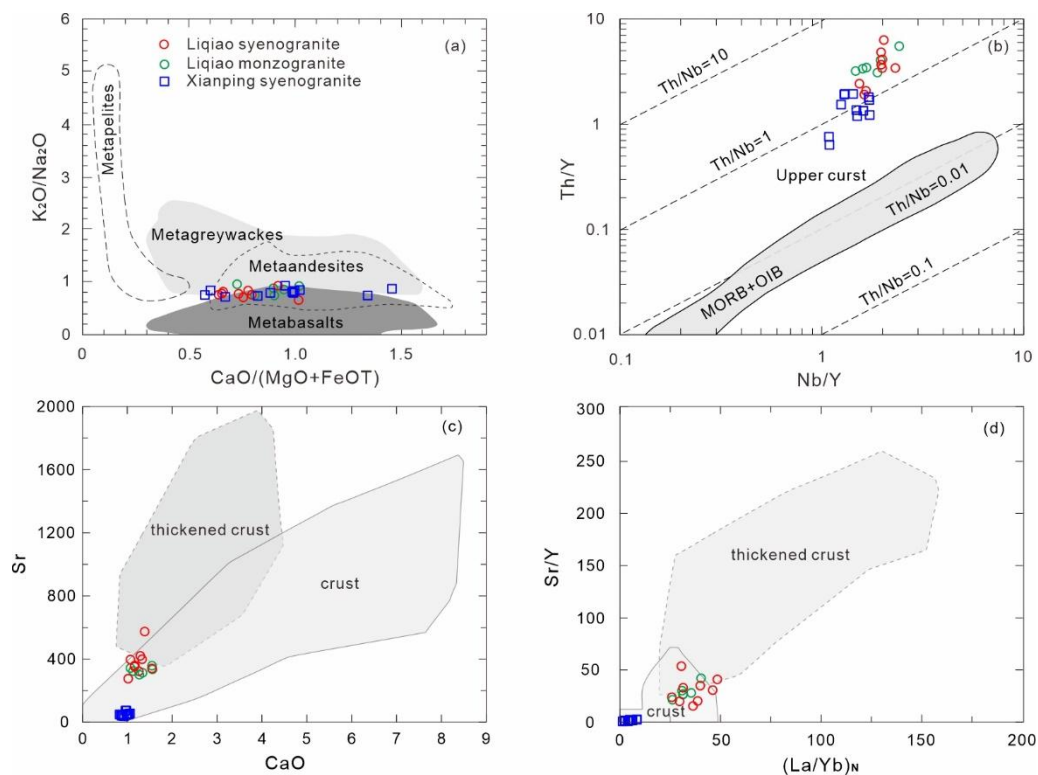
Figure 10: The source region diagrams of the LP and XP in the western section of North Qinling Orogen: (a) molar K_2O/Na_2O versus molar CaO/(MgO+FeO^I) (Altherr and Siebel 2002); (b) Nb/Y versus Th/Y (Boztuğ et al. 2007); (c) CaO versus Sr (He et al. 2011); (d) (La/Yb)_N versus Sr/Y (He et al. 2011).
