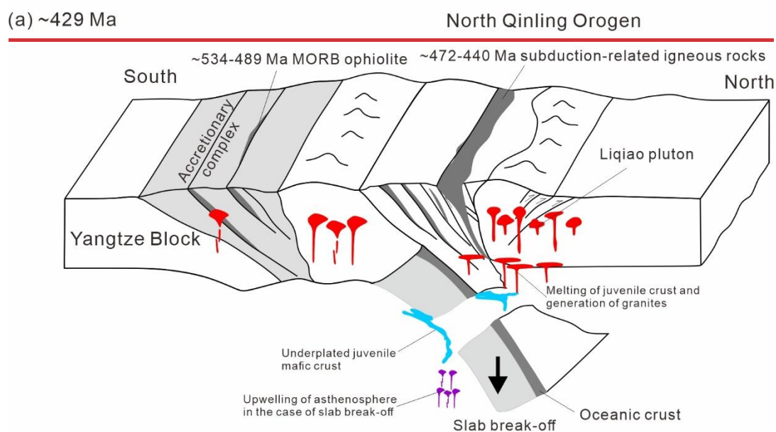
Figure 13: Schematics geodynamic and petrogenetic model illustrating the evolution of the western section of the NQO at ca. 429 Ma and 421 Ma, and the generation of the LP (a) and XP (b) during Late Silurian. MORB—mid-ocean ridge basalt.
