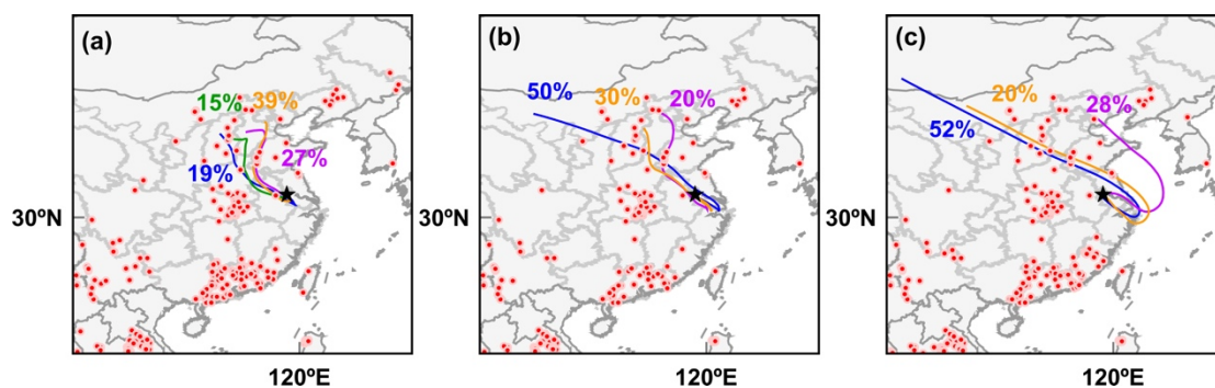
Figure S1. Three-day HYSPLIT back trajectories initiated over Nanjing with altitudes below 500 m, along with MODIS fire spots across three episodes with PM_{2.5} concentrations of (a) > 200 , (b) 100-200 , and (c) < 100 \mu g m^{-3} . The black star indicates the sampling site. MODIS active fire data can be accessed here: https://firms.modaps.eosdis.nasa.gov/download/list.php .
