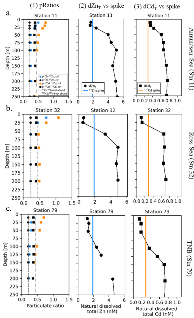
Figure S1. (1) Particulate ^{67}\text{Zn}: ^{68}\text{Zn} and ^{110}\text{Cd}: ^{114}\text{Cd} ratios measured in the \geq 3 \mu\text{m} fraction showing deviations from natural abundance ratios, (2) natural total dissolved Zn (dZn T ) compared to the concentration of ^{67}\text{Zn} spike added, and (3) natural total dissolved Cd (dCd T ) compared to the concentration of ^{110}\text{Cd} spike at a representative station from each group (a., Amundsen Sea, b. Ross Sea, c., Terra Nova Bay (TNB)). Deviation of surface sample ratios from natural abundance represents enrichment of the spiked tracer isotopes ^{67}\text{Zn} and ^{110}\text{Cd} in the particulate fraction, indicative of uptake from the dissolved fraction. Stn, station.
