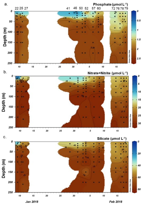
Fig. S6. Macronutrients measured within Terra Nova Bay. (a) phosphate, (b), sum of nitrate and nitrite, and (c) silicate in the upper 250m measured at all 13 Terra Nova Bay stations represented in color scale. Station numbers are given at the top of (a) and (I). Station data is presented in order of sampling date, from the earliest (station 22, early January) to the latest (station 79, late February).
