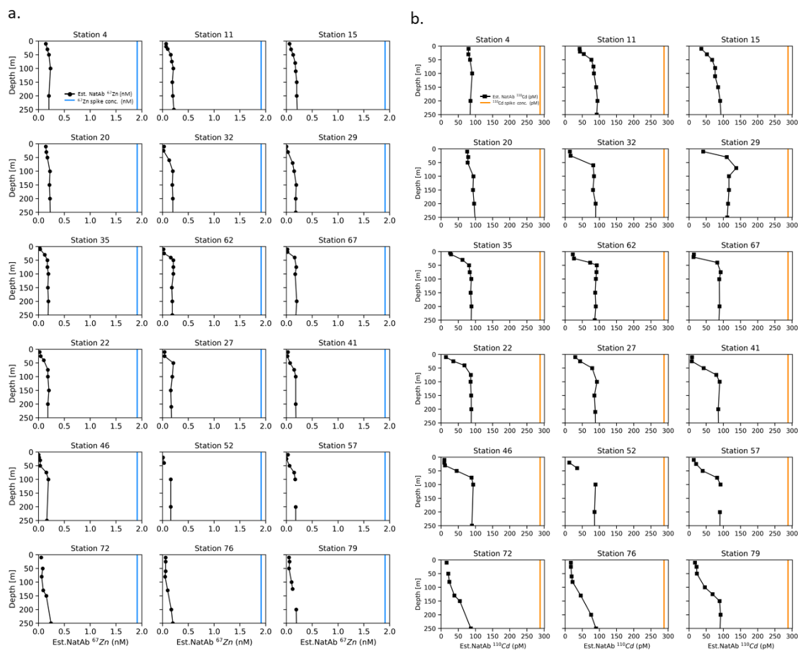
Figure S2. (a) The estimated natural abundance of ^{67}\text{Zn} and (b) the estimated natural abundance of ^{110}\text{Cd} in the upper 250m at each station calculated by multiplying total dissolved concentrations of Zn and Cd at each depth by the natural abundance of ^{67}\text{Zn} and ^{110}\text{Cd} (0.0410 and 0.1249, respectively; see Methods). Colored vertical lines denote the spiked concentration of ^{67}\text{Zn} (blue, 1.9 nM) and ^{110}\text{Cd} (orange, 288 pM). At each station, spikes were greater than the natural dissolved ^{67}\text{Zn} and ^{110}\text{Cd} at every depth.
