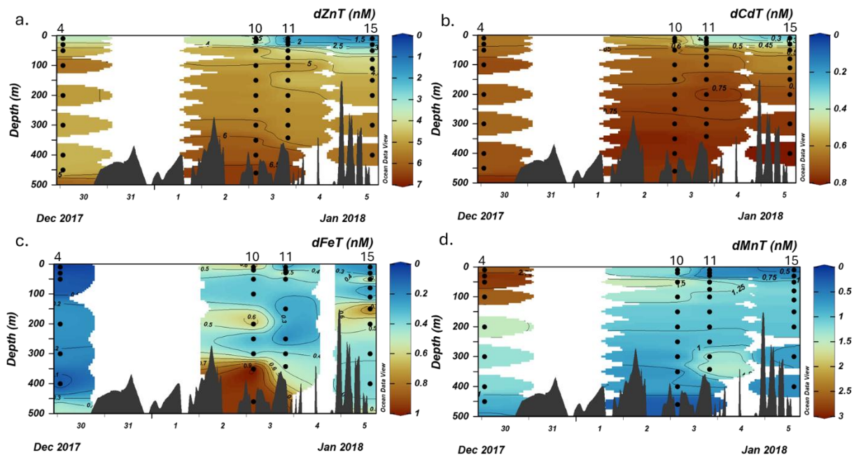
Figure S3. Total dissolved metal concentrations of (a) zinc, (b) cadmium, (c) iron, and (d) manganese measured in the upper 500 m in the Amundsen Sea represented in color scale.
