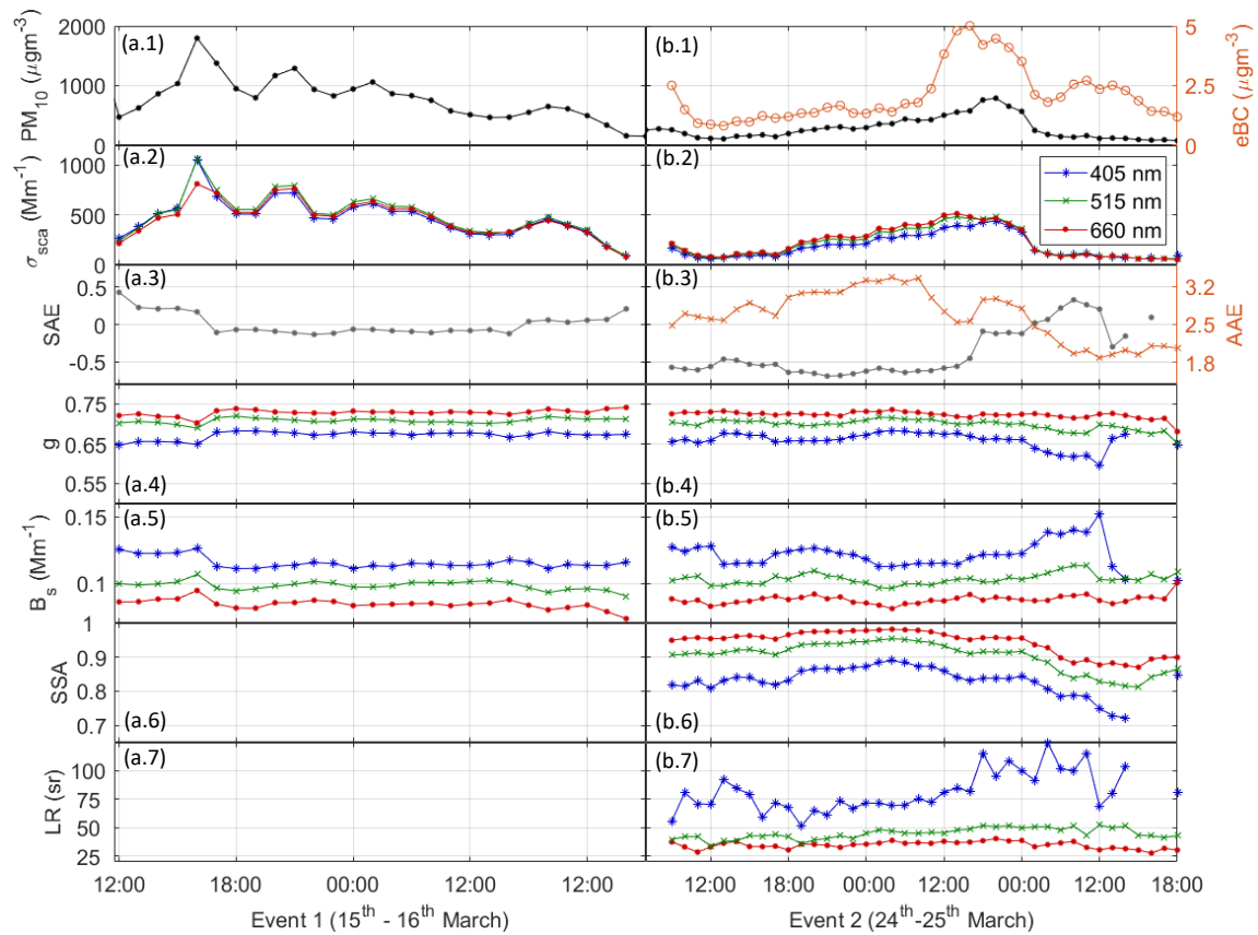
Figure 5. Time series of the PM 10 and eBC concentrations (a.1, b.1), \sigma_{\text{sca}} – scattering coefficient (a.2, b.2), SAE – scattering Angström exponent and AAE – absorption Angström exponent (a.3, b.3), g – asymmetry parameter (a.4, b.4), B_s – fraction of backscattered light (a.5, b.5), SSA – single scattering albedo (a.6, b.6) and LR – lidar ratio (a.7, b.7) for the extreme dust events of 15 th March (a) and 24 th March 2022 (b).
