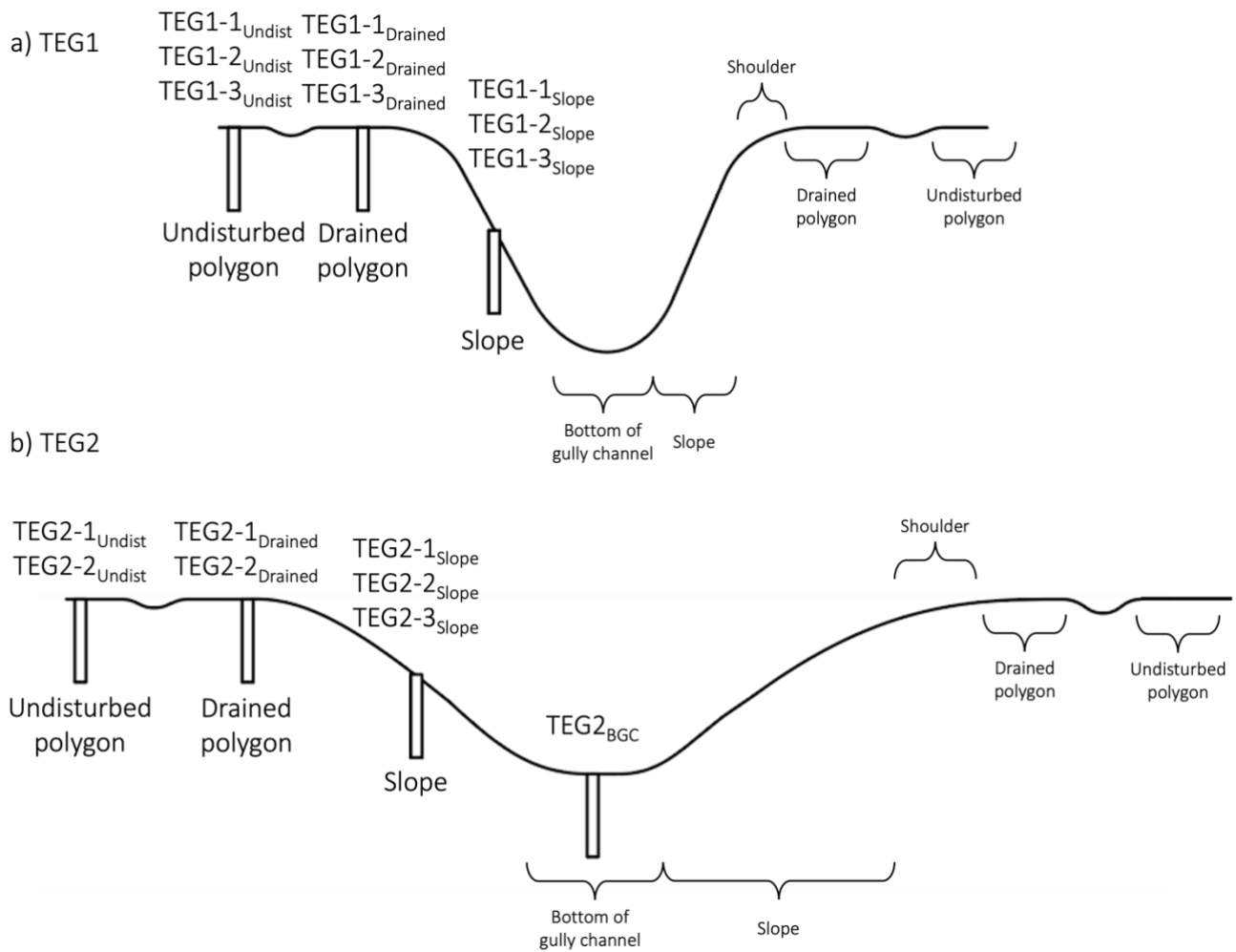
150 Figure 2. Conceptual cross-section of the two thermo-erosion gullies, TEG1 (a) and TEG2 (b), showing the sections of the TEGs where thaw front depth was probed (only one side is annotated, but for slopes and shoulders, both sides were probed), and the locations where we drilled into permafrost. While TEG1 was composed of three subsites, TEG2 had cores relatively close to one another. The locations of the cores are relative to the cross-section of the gullies, for their exact location see Figure 1. Figure not to scale.
