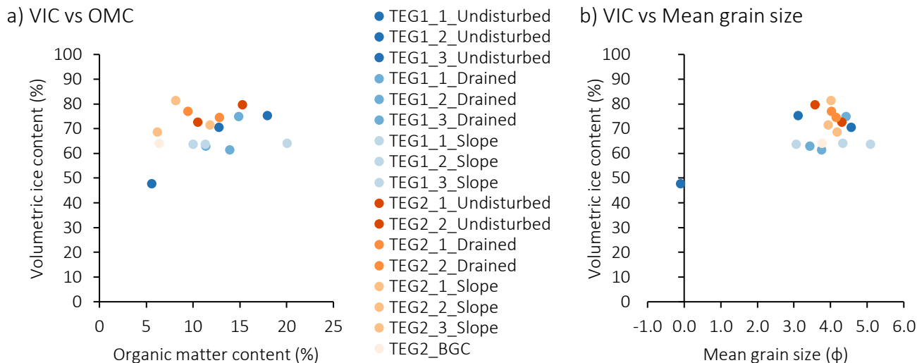
345 Figure 7. Volumetric ice content (VIC) against a) organic matter content (OMC) and b) mean grain size for each core of TEG1 and TEG2. Cores from TEG1 and TEG2 are in blue and orange shades, respectively. VIC, OMC, and mean grain size are weighted averages down to 1 m deep for each core.
