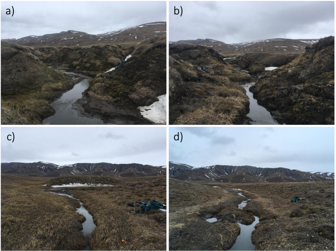
205 Figure 3. Thermo-erosion gullies 1 (TEG1, a-b) and 2 (TEG2, c-d). a) TEG1, near subsite TEG1-2, b) TEG1, near subsite TEG1-3. c) TEG2, near the transect where the cores were drilled, and d) TEG2, near TEG2_TFD2, about 400 m upstream of the cores. All pictures were taken on 24 June 2018 and point South-East. The backpack on the pictures is about 80 cm long.
