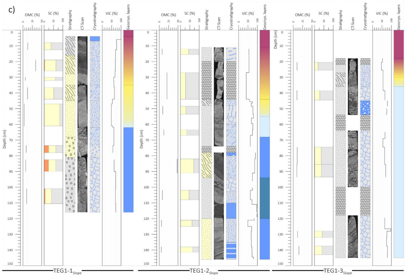
305 Figure 5. Organic matter content (OMC; %), soil composition (SC; %gravel, %sand, %silt), soil stratigraphy, CT-scan imagery, soil cryostratigraphy, volumetric ice content (VIC; %), and geocryological layers for the cores at TEG1. a) Cores in undisturbed polygons, b) cores in drained polygons, and c) cores in slopes of TEG1. While delineations were used to mark the transitions between the frozen part of the active layer, the transient layer, and the intermediate layer, color gradients were also used to denote the uncertainty in the limits between these layers. Refer to figure 6 for the legend.
