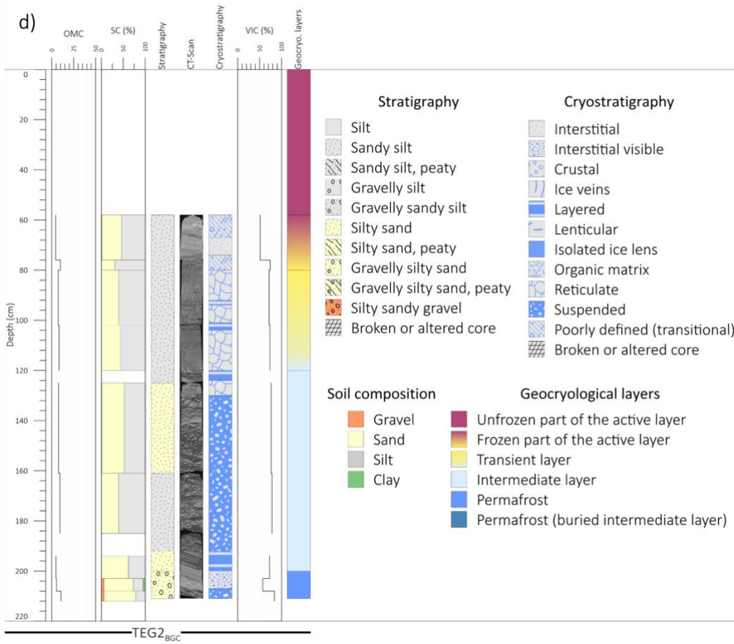
340 Figure 6. Organic matter content (OMC; %), soil composition (SC; %gravel, %sand, %silt), soil stratigraphy, CT-scan imagery, soil cryostratigraphy, volumetric ice content (VIC; %), and geocryological layers for the cores at TEG2. a) Cores in undisturbed polygons, b) cores in drained polygons, c) cores in slopes of TEG2, and d) core at the bottom of the gully channel of TEG2. While delineations were used to mark the transitions between the frozen part of the active layer, the transient layer, and the intermediate layer, color gradients were also used to denote the uncertainty in the limits between these layers.
