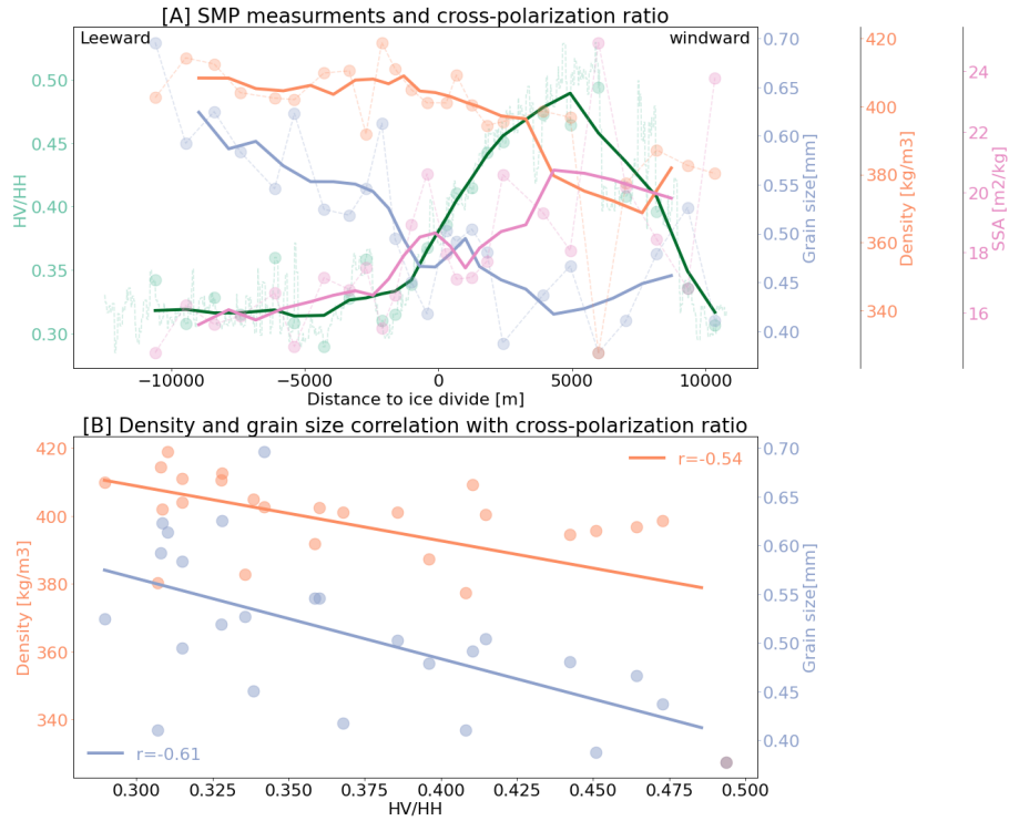
Figure 9. A) SMP measurements compared to the cross-polarization ratio across LIR in a east to west profile across the LIR. SMP measurements include the average optically equivalent grain diameter, density and SSA of the first meter of snow. The points are the actual measurements and the solid lines are running means with a 4 point window for the SMP measurements and a 80 pixel running mean for the Sentinel-1 cross-polarization ratio. The location of the SMP measurements is shown in Fig. 4 H. B) shows the correlation between the the cross-polarization ratio and the optically equivalent grain diameter (blue) and the density (orange) measured by the SMP.
