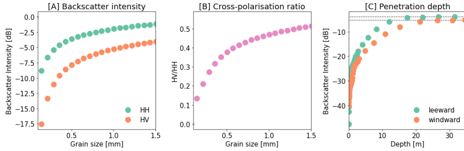
Figure 8. Synthetic backscatter intensity modelled with SMRT. A) shows the modelled \sigma_{HH} and \sigma_{HV} intensity with increasing optically equivalent grain diameter. B) shows the \sigma_{HV}/\sigma_{HH} with increasing optically equivalent grain diameter. C) shows the increase in \sigma_{HH} when including deeper layers on the windward and leeward side of LIR. The dotted lines in C) represent the Backscatter intensity of the complete snowpack, to highlight at which point the Backscatter intensity is no longer increasing.
