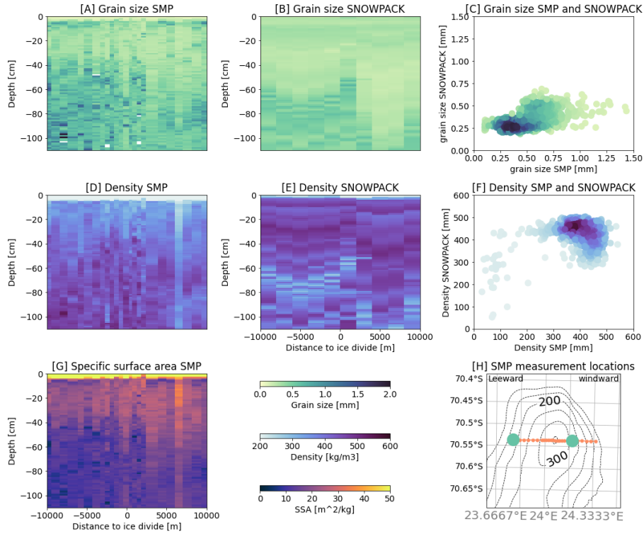
Figure 4. SMP measured optically equivalent grain diameter (A), density (D) and specific surface area (SSA) (G) at LIR as well as SNOWPACK modelled optically equivalent grain diameter (B) and density (E). The third column shows how the results compare between SMP and SNOWPACK, with panel (C) showing optically equivalent grain diameter and (F) density. (H) shows the location of the SMP measurements taken across LIR (orange dots) as well as the locations of the AWS (green dots).
