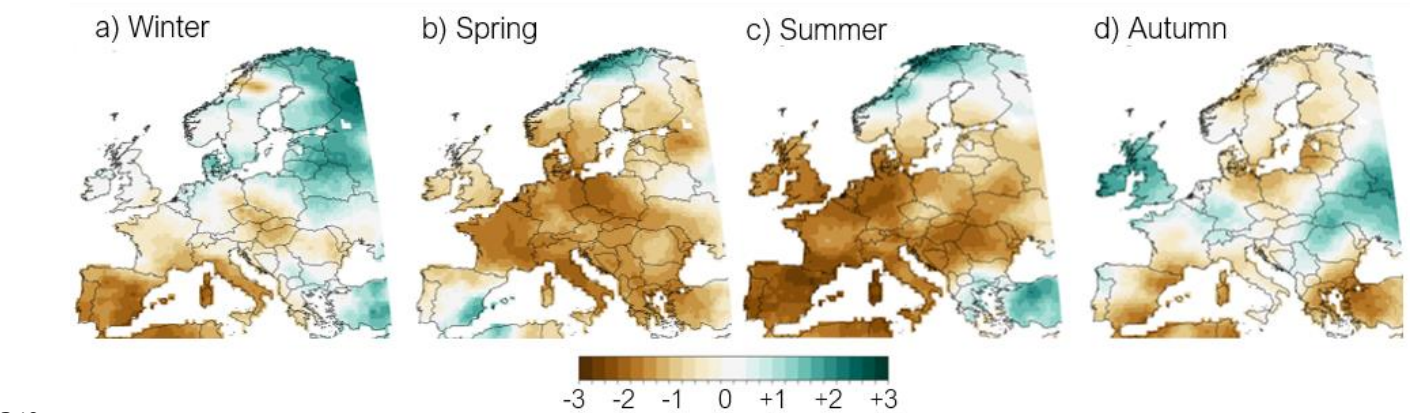
340 Figure 2: Seasonal evolution of the Standardized Potential Evapotranspiration Index for 3-month accumulation (SPEI-3) for 2022; a) Winter (SPEI-3 February); b) Spring (SPEI-3 May); c) Summer (SPEI-3 August) and d) Autumn (SPEI-3 November).
