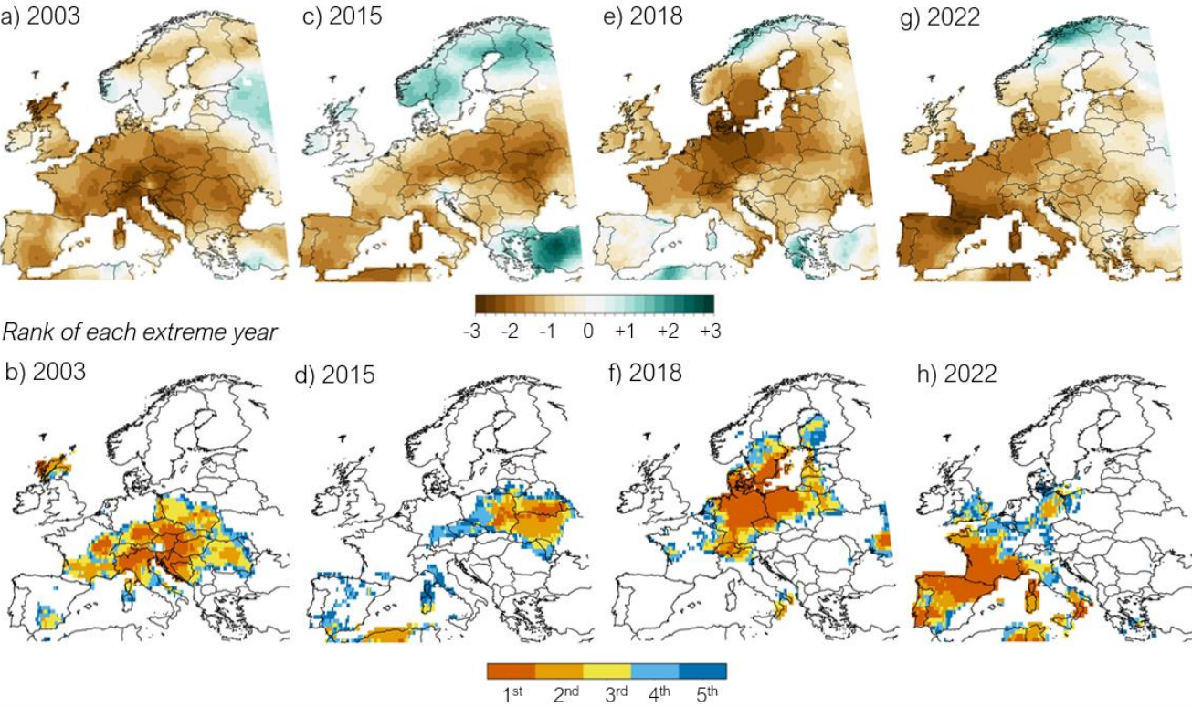
Figure 3: Comparison of the SPEI6 for September of the main Europe-wide droughts since 2000: Namely, 2003, 2015, 2018, and 2022 (top row) and their associated ranking (bottom row). The period analysed is 1950–2022. A rank of one signifies that SPEI6 September for a given year (i.e. 2003, 2015, 2018 or 2022) is record-breaking, i.e. the lowest value during the analysed period.
