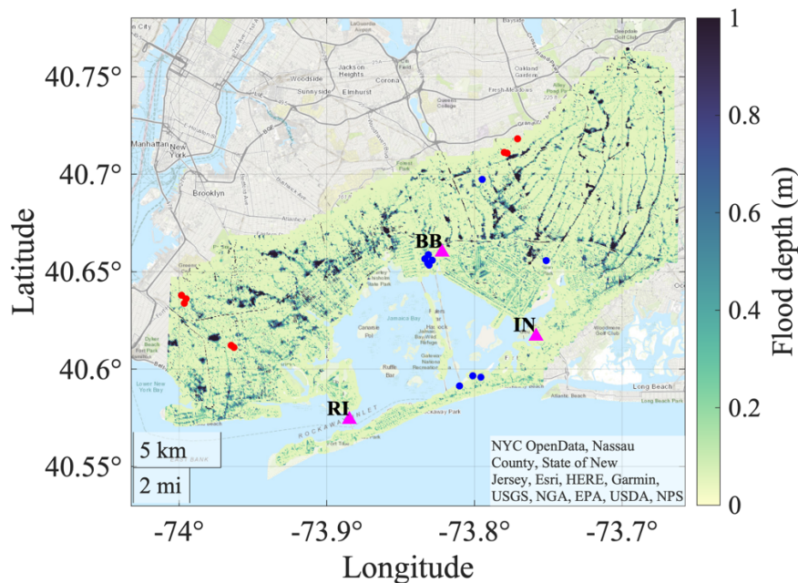
Figure 6 Flood depth above ground level (model with no drainage), red circles, blue circles and purple triangles show HWMs from Ida, HWMs from September 29 th storm, and tide gauge locations, respectively. Tide gage locations Bergen Basin (BB), Rockaway (RI), and Inwood (IN) are shown. (topographic base map from MATLAB, hosted by Esri®)
