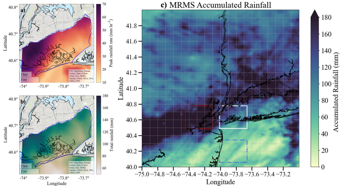
Figure 3. a) Maximum hourly rain intensity for Ida, b) Total accumulated rain during Aug 29, 2021, to Sep 02, 2021, for Ida. (watershed boundary is shown with blue dots, and topographic base maps are from MATLAB, hosted by Esri®), c) Ida total rain is shown as color shading (temporally accumulated rainfall over the 5-days simulation time). The white box shows the Jamaica Bay domain, whereas the red box (dot line) shows the rain that would fall over the domain if the rain were displaced eastward (worst case scenario), and the blue box (dash-dot line) shows what rain would fall over the domain for a displacement northward (best case scenario).
