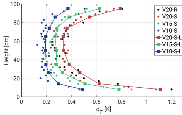
Figure 5. Standard deviation \sigma_{T'} with respect to the position of the sensor. Short time series (3 min) are denoted by circles, squares represent longer measurements (19 min). Decreasing \Delta T shifts left \sigma_{T'} values reducing the temperature fluctuations at all positions.
