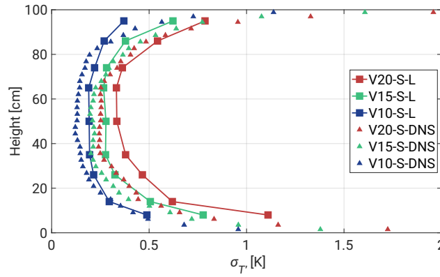
Figure 11. Standard deviation \sigma_{T'} with respect to the height of the chamber. The chart analogous to Fig. 5 but including only 19 min segments (squares) and the DNS (triangles).
