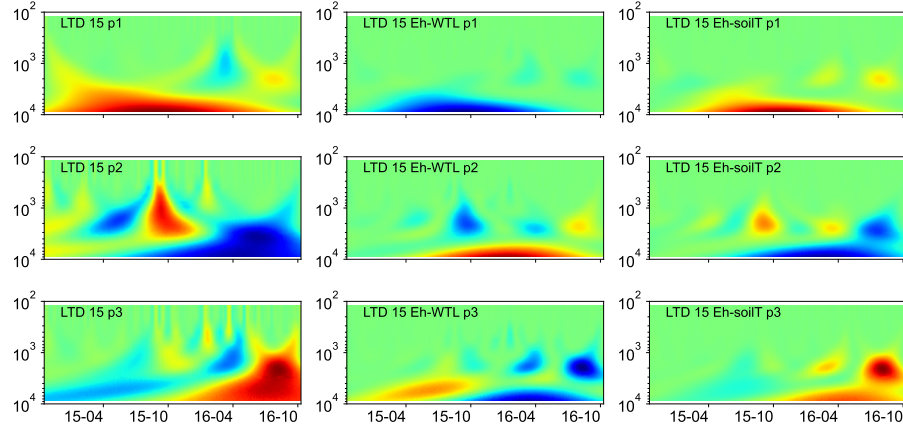
Figure 5. Left-Left: Wavelet coherence between Mexican hat wave and E_h at the ME-LTD plot ;(15 cm depth); center-centre: interaction between E_h and WTL wavelets; right-right: interaction between E_h and soil temperature wavelets at the LTD plot ;(15 cm depth). 3-Top to bottom: three probes plotted separately (p1 ... p3). Note logarithmic, inverted scale (hours) on y-axis, dates as YY-MM on x-axis.
