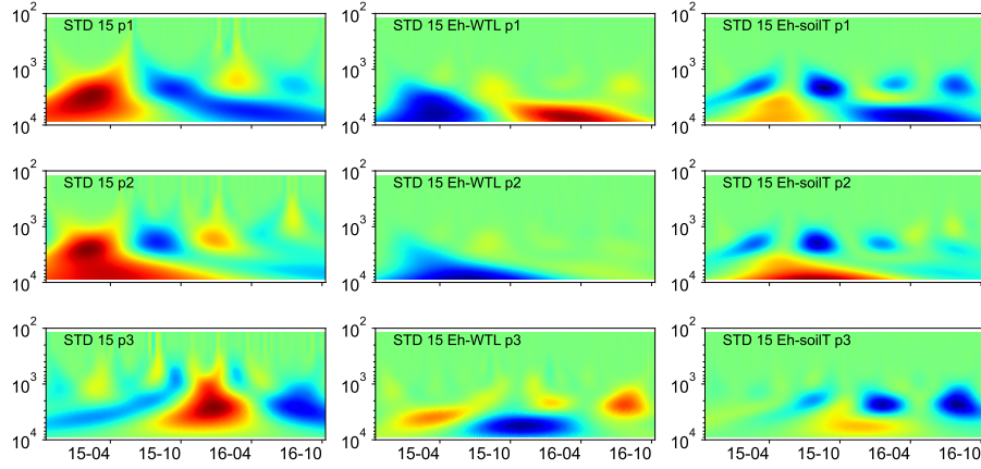
Figure 7. Left-Left: Wavelet coherence between Mexican hat wave and E_h at the ME-STD plot (15 cm depth); center-centre: interaction between E_h and WTL wavelets; right-right: interaction between E_h and soil temperature wavelets at the ME-STD plot (15 cm depth). 3-Top to bottom: three probes plotted separately (p1 . . . p3). Note logarithmic, inverted scale (hours) on y-axis, dates as YY-MM on x-axis.
