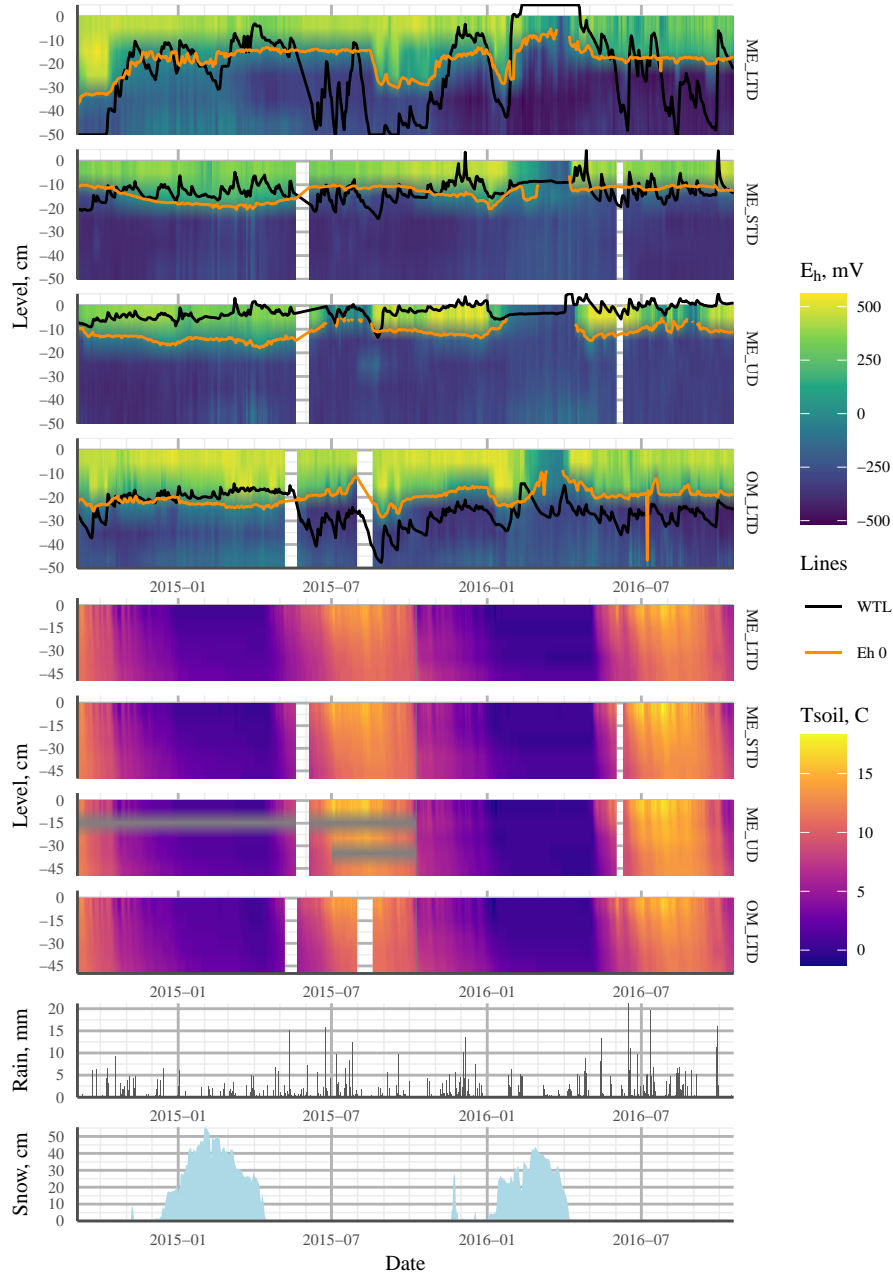
Figure 3. Heat maps showing mean values (mean of three profiles per treatment) interpolated from the 5-45 cm depth profiles of E_h (four topmost plots; four topmost plots: ME LTD, ME STD, ME UD, OM LTD; WTL and the E_h 0 isopotential shown as solid black and orange lines, respectively) and soil temperature (four middle plots; four middle plots: ME LTD, ME STD, ME UD, OM LTD), with WTL and the 0 isopotential shown as solid black and orange lines over the plots, respectively. The two plots at the bottom show Bottom two plots: daily rainfall (mm) and snow pack thickness (cm) at the peatland over the study period. ME = mesotrophic sedge fen; OM = ombrotrophic bog; UD = undrained; STD = short-term (~ 15 years) drainage; LTD = long-term (~ 55 years) drainage.
