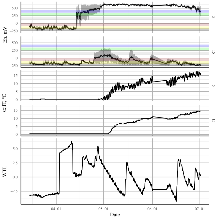
Figure 12. Redox potential ( E_h ) and soil temperature (soilT) at 5 and 15 cm depth, and water table level (WTL) at the undrained (UD) plot in Spring 2016. Solid black line in E_h : mean of 3-three profiles, shaded area: S-E-Standard Error. Horizontal coloured bars represent approximate theoretical E_h values of transition between different TEAs, from top to bottom: O_2 , NO_3^- , Mn^{4+} , Fe^{3+} , SO_4^{2-} , CO_2
