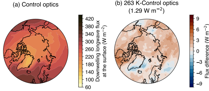
Figure 5. (a) The 1 year ensemble mean downwelling longwave flux at the surface from the B1850_UVnudge1980 control run. Flux differences in the 1 year ensemble averages between (b) the 263 K and control optics runs from B1850_UVnudge1980. Stippling indicates the differences are statistically significant at the 95 % confidence level. False discovery rate was controlled for using Wilks (2016). The colormaps are generated based on work by Crameri et al. (2020).
