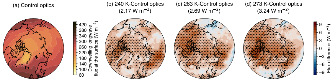
Figure 3. (a) The 1 year ensemble mean downwelling longwave flux at the surface from the F1850_UVnudge1980 control run. Flux differences in the 1 year ensemble averages between (b) the 240 K and control optics runs, (c) the 263 K and control optics runs, and (d) the 273 K and control optics runs from F1850_UVnudge1980. In parentheses above the (b), (c), and (d) plots is the spatial average of the flux differences over 60–90° N. Stippling indicates the differences are statistically significant at the 95 % confidence level. False discovery rate was controlled for using Wilks (2016). The colormaps are generated based on work by Crameri et al. (2020).
