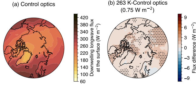
Figure 4. (a) The 39 year ensemble mean downwelling longwave flux at the surface from the F1850_UVnudge1980–2018 control run. Flux differences in the 39 year ensemble averages between (b) the 263 K and control optics runs from F1850_UVnudge1980–2018. In parentheses above the (b) plot is the spatial average of the flux differences over 60–90° N. Stippling indicates the differences are statistically significant at the 95 % confidence level. False discovery rate was controlled for using Wilks (2016). The colormaps are generated based on work by Crameri et al. (2020).
