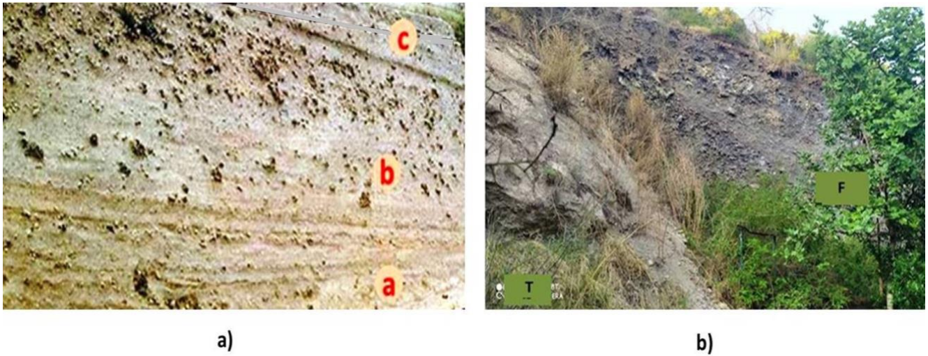
739 740 Fig. 17 – a) Flow units in the phreatomagmatic Pyroclastic flows, b) Deposit of the final scoria 741 flow (F) in the western depression of the phreatomagmatic Tuff cone (T).
