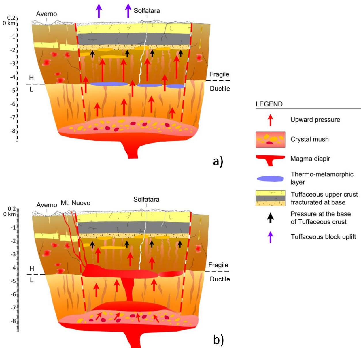
Fig. 16 – Schematic cross sections of the hydrothermal and magmatic systems underlying the Campi Flegrei resurgent block in the 1538 AD, showing:
