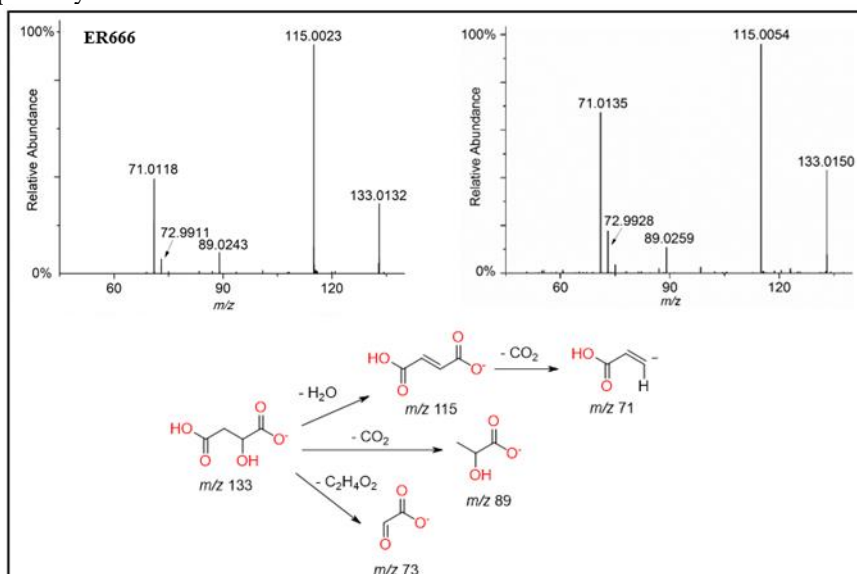
5 Figure 9. ESI(-) product ion mass spectra of malic acid (MW 134) eluting at RT = 0.82 min, registered for the ER666 non-acidified seed aerosol sample (left) and standard compound (right) along with a proposed fragmentation pathway.
