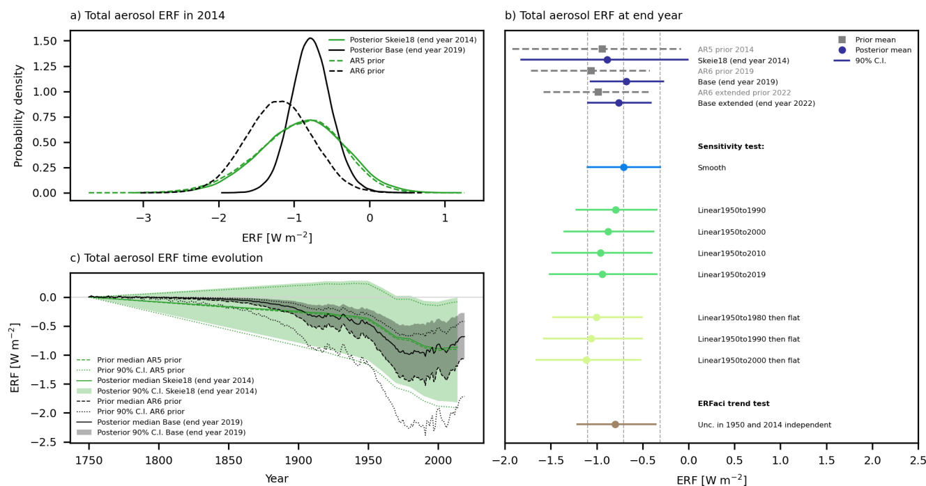
205 Figure 3. Same as Fig. 2, but for aerosol ERF. The underlying numbers for b) is presented in Table S4.
