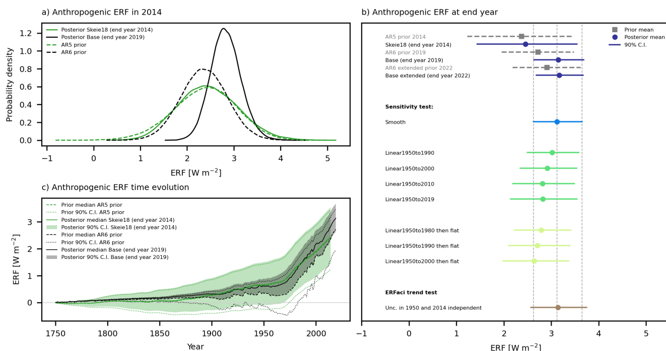
190 Figure 2: Prior and posterior distributions of anthropogenic ERF. In a) the probability density function of the prior (dashed line) and posterior (solid line) ERF in 2014 for “Base” using AR6 prior (black) and “Skeie18” using AR5 prior (green). In b) the posterior 90% C.I. is indicated by a solid line and the posterior mean as a dot and the prior 90% C.I. is indicated by a dashed line and the prior mean as a square. The results are shown for the end year in the analysis. In c) the prior and posterior time evolutions of the anthropogenic ERF are shown for “Skeie18” and “Base”. The underlying numbers for b) are presented in Table S3.
