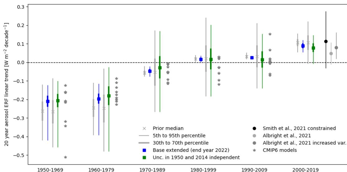
395 Figure 5: The 20-year aerosol ERF linear trend for six different periods. The posterior aerosol ERF trends are shown for “ Base extended ” (blue) and the test with independent uncertainties in 1950 and 2014 (green) with corresponding prior distribution plotted in gray to the left of the posterior. The median (crosses for prior and squares for posterior), 30th to 70th percentile and 5th to 95th percentiles are shown. For the five first time periods, the linear trend in the ERF diagnosed from 9 CMIP6 models in Smith et al. (2021b) are shown as stars and the linear trends are calculated on smoothed time series of ERF. For the last period (2000 to 2019) the mean, 5th and 95th percentiles presented in Quaas et al. (2022) from Albright et al. (2021) and Smith et al. (2021b) are shown.
