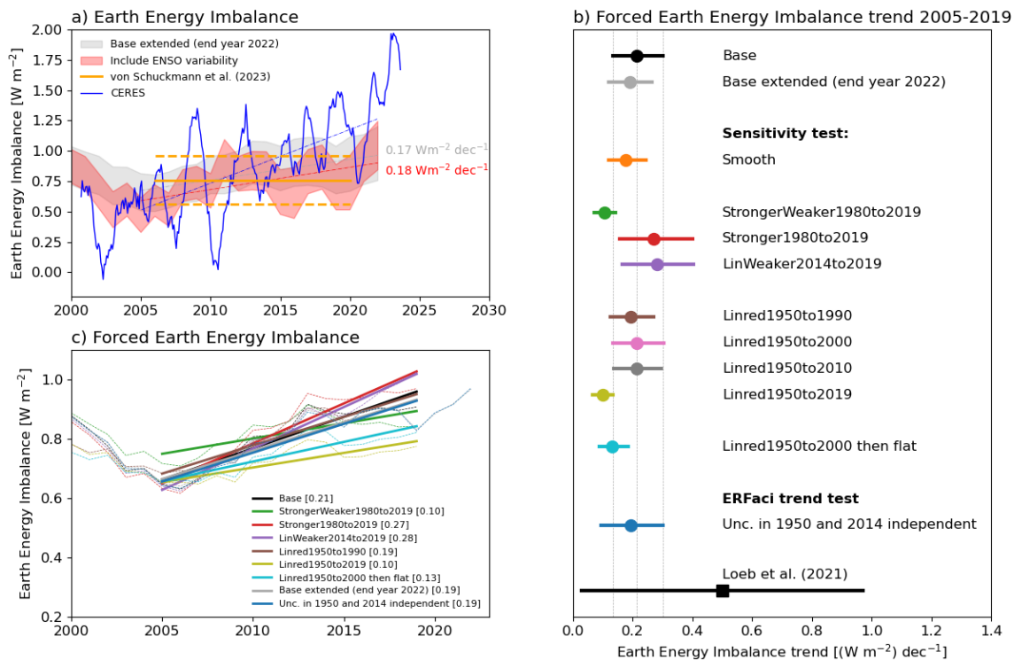
455 Figure 6: Posterior Earth Energy Imbalance and Earth Energy Imbalance trend. In a) the gray shading shows the 5 to 95 percentile of the posteriori EEI for the forced temperature response, while the red shading shows the posteriori EEI including ENSO variability for “Base extended”. The gray and red dashed line indicate the least squares linear fit for the posterior median of EEI without and with ENSO variability included for the period 2005 to 2022 and the trend over this period are indicated in the plot. The orange lines are the EEI from von Schuckmann et al. (2023) of 0.76 W m -2 (solid line) ± 0.2 W m -2 (dashed lines) for the 90% confidence interval for the period 2006 to 2020. CERES data are shown as a 12-month running mean in blue (Loeb et al., 460
