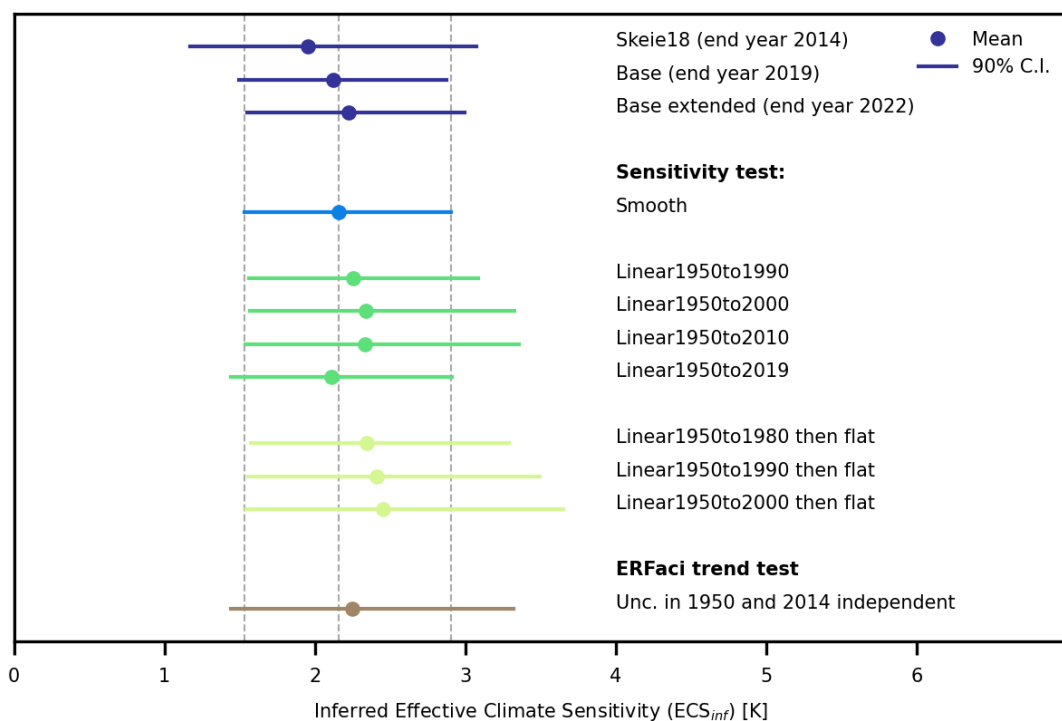
165 Figure 1: Posterior inferred effective climate sensitivity ( ECS_{inf} ) for the different analyses and sensitivity tests. The 5 th to 95 th percentiles ranges are indicated by a solid line and the mean values as a dot. The vertical lines indicate the posterior mean value and the 90% C.I. for “Smooth”, as it is used as a starting point for the “Linear” sensitivity tests shown. The posterior mean, median and 5 th and 95 th percentiles are presented in Table S1 and description of all estimations in Table A3. For AR5 we use the best estimate of 2xCO 2 radiative forcing from AR5, while for AR6 we use the 2xCO 2 ERF corresponding to the posteriori estimate of the historical CO 2 ERF for the conversion from climate sensitivity parameter to ECS_{inf} (see Appendix A). 170
