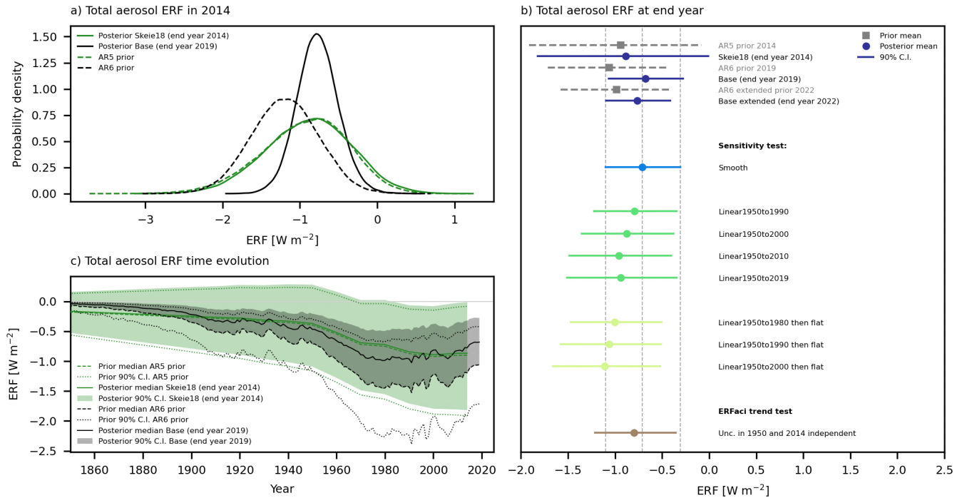
210 Figure 3. Same as Fig. 2, but for aerosol ERF. The underlying numbers for b) are presented in Table S4.
