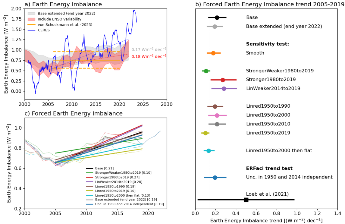
Figure 7: Posterior Earth Energy Imbalance and Earth Energy Imbalance trend. In a) the gray shading shows the 5 to 95 percentile of the posteriori EEI for the forced temperature response, while the red shading shows the posteriori EEI including ENSO variability for “Base extended”. The gray and red dashed line indicate the least squares linear fit for the posterior median of EEI without and with ENSO variability included for the period 2005 to 2022 and the trend over this period are indicated in the plot. The orange lines are the EEI from von Schuckmann et al. (2023) of 0.76 \text{ W m}^{-2} (solid line) \pm 0.2 \text{ W m}^{-2} (dashed lines) for the 90% confidence interval for the period 2006 to 2020. CERES data are shown as a 12-month running mean in blue (Loeb et al., 2018a) (include data for January 2024) and the least squares linear fit from 2005 to 2022 (dashed blue line). In b) the posteriori forced EEI trend over the period 2005 to 2019 are shown as 5 th to 95 th percentile as solid line and median value as a dot. At the bottom the mid-2005 to mid-2019 estimates for the trend for the net CERES TOA energy flux of 0.50 \pm 0.47 \text{ W m}^{-2} \text{ decade}^{-1} (90% confidence interval) from Loeb et al. (2021) are indicated with a black square and the solid line. In c) the posteriori median of the forced EEI from 2000 and onwards are shown for selected sensitivity tests as annual values (dashed lines) and the linear trend from between 2005 to 2019 as solid line. The trends in EEI over this period are indicated in the legend as \text{W m}^{-2} \text{ decade}^{-1} .
