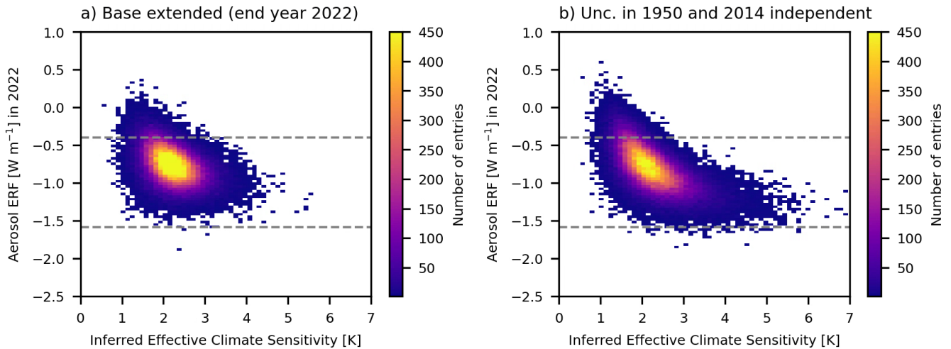
Figure 4: The joint posterior distribution of aerosol ERF in 2022 and posterior ECS inf . In a) for “Base extended” and in b) where the aerosol ERF aci uncertainties in 1950 and 2014 are treated independently. The 5 th and 95 th percentile in the aerosol ERF prior for 2022 are shown as horizontal dashed lines.
