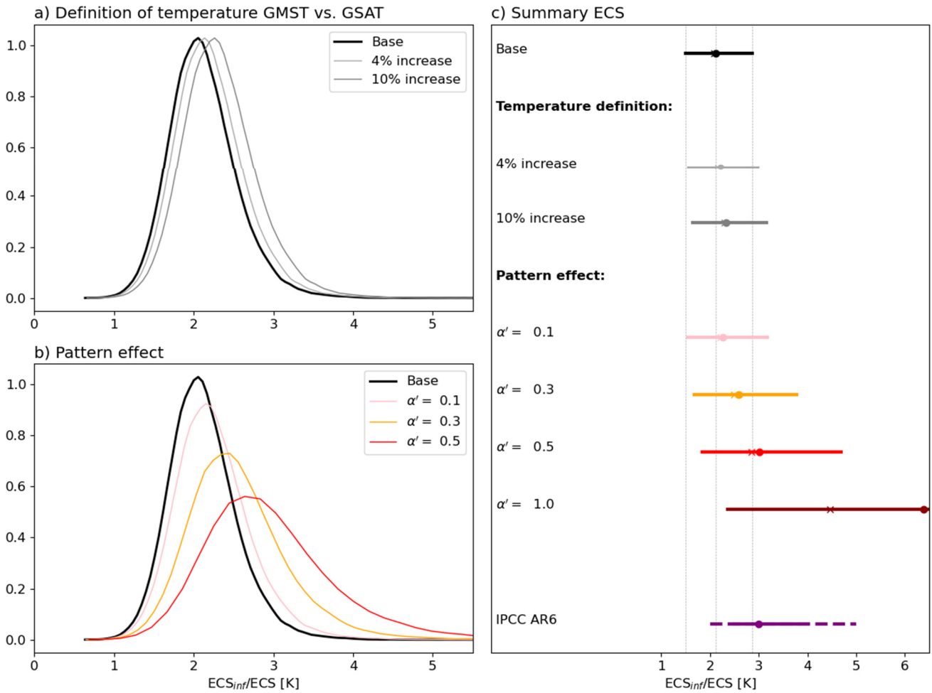
305 Figure 5: Illustrations of reasons for differences between observational estimates of ECS_{inf} and Effective Climate Sensitivity (ECS) as diagnosed from climate models. In a) the influence on ECS by different definitions of temperature is illustrated. The ECS_{inf} estimated in “Base”, based on observations of GMST, are enhanced by 4% and 10% as changes in GMST are larger than GSAT in climate models. In b) different assumptions of the “Pattern Effect” are added to the ECS_{inf} estimate from “Base”. The different values for \alpha' is given in the legend. For “Base” \alpha'=0 . In c) the results are summarized by the mean value (filled circle), median value (x) and 5 th to 95 th percentile range as solid line. Also indicated is the assessed best estimate of Equilibrium Climate Sensitivity from IPCC AR6 (filled circle) and the very likely (solid line) and likely (dashed line) uncertainty range. 310
