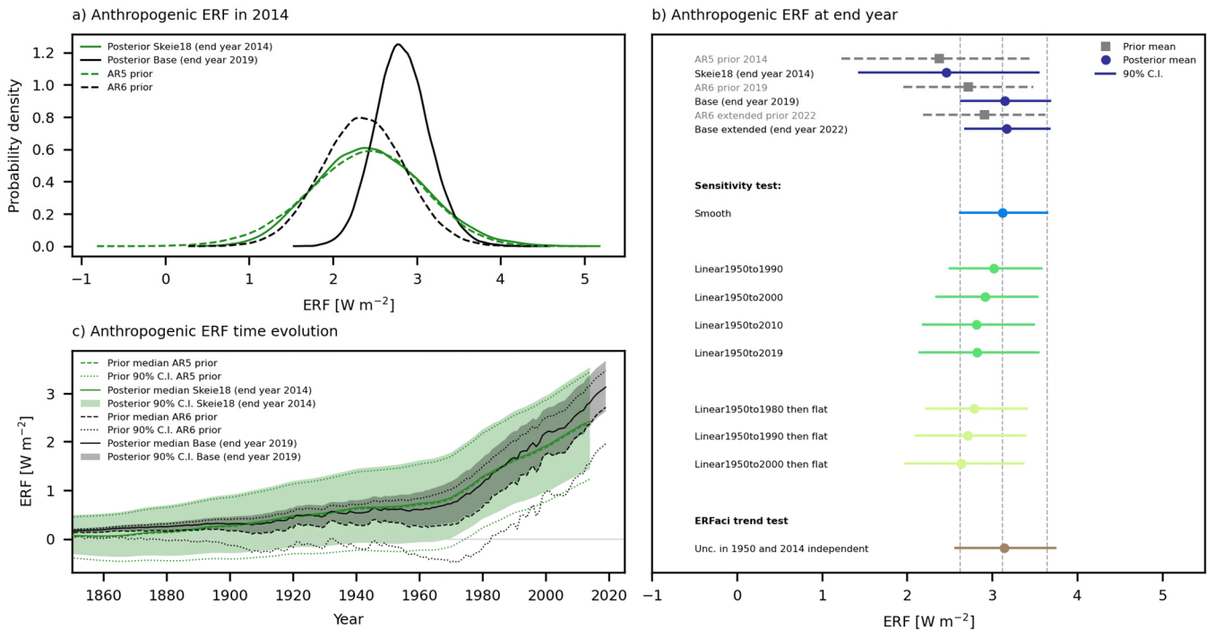
195 Figure 2: Prior and posterior distributions of anthropogenic ERF. In a) the probability density function of the prior (dashed line) and posterior (solid line) ERF in 2014 for “Base” using AR6 prior (black) and “Skeie18” using AR5 prior (green). In b) the posterior 90% C.I. is indicated by a solid line and the posterior mean as a dot and the prior 90% C.I. is indicated by a dashed line and the prior mean as a square. The results are shown for the end year in the analysis. In c) the prior and posterior time evolutions of the anthropogenic ERF are shown for “Skeie18” and “Base”. The underlying numbers for b) are presented in Table S3.
