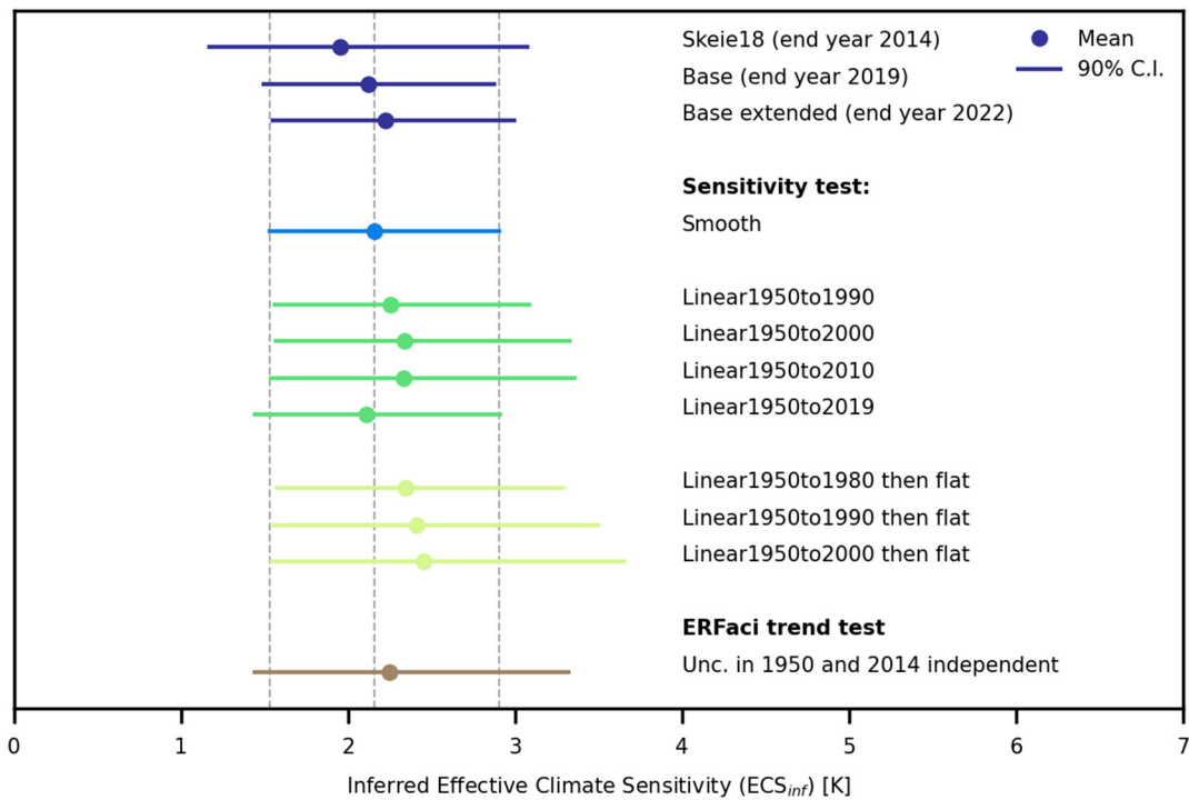
170 Figure 1: Posterior inferred effective climate sensitivity ( ECS_{inf} ) for the different analyses and sensitivity tests. The 5 th to 95 th percentiles ranges are indicated by a solid line and the mean values as a dot. The vertical lines indicate the posterior mean value and the 90% C.I. for “Smooth”, as it is used as a starting point for the “Linear” sensitivity tests shown. The posterior mean, median and 5 th and 95 th percentiles are presented in Table S1 and description of all estimations in Table A3. For AR5 we use the best estimate of 2xCO 2 radiative forcing from AR5, while for AR6 we use the 2xCO 2 ERF corresponding to the posteriori estimate of the historical CO 2 ERF for the conversion from climate sensitivity parameter to ECS_{inf} (see Appendix A).
