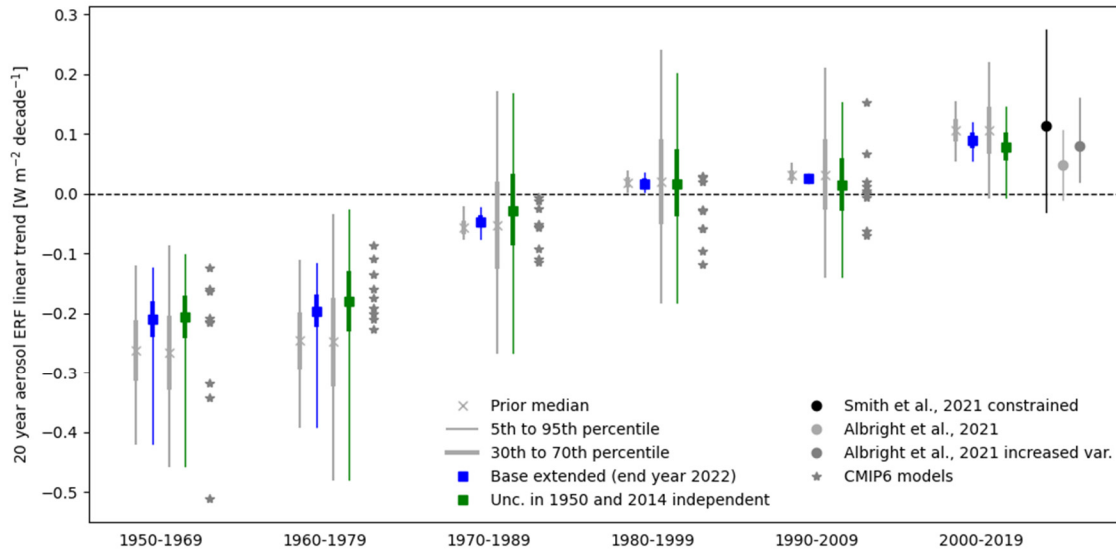
415 Figure 6: The 20-year aerosol ERF linear trend for six different periods. The posterior aerosol ERF trends are shown for “Base extended” (blue) and the test with independent uncertainties in 1950 and 2014 (green) with corresponding prior distribution plotted in gray to the left of the posterior. The median (crosses for prior and squares for posterior), 30th to 70th percentile and 5th to 95th percentiles are shown. For the five first time periods, the linear trend in the ERF diagnosed from 9 CMIP6 models in Smith et al. (2021b) are shown as stars and the linear trends are calculated on smoothed time series of ERF. For the last period (2000 to 2019) the mean, 5th and 95th percentiles presented in Quaas et al. (2022) from Albright et al. (2021) and Smith et al. (2021b) are shown.
