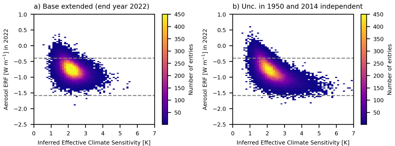
Figure 4: The joint posterior distribution of aerosol ERF in 2022 and posterior ECS_{inf} . In a) for “ Base extended ” and in b) where the aerosol ERFaci uncertainties in 1950 and 2014 are treated independently. The 5 th and 95 th percentile in the aerosol ERF prior for 2022 are shown as horizontal dashed lines.
