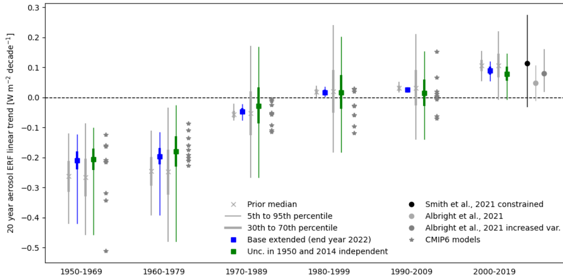
420 Figure 56: The 20-year aerosol ERF linear trend for six different periods. The posterior aerosol ERF trends are shown for “ Base extended ” (blue) and the test with independent uncertainties in 1950 and 2014 (green) with corresponding prior distribution plotted in gray to the left of the posterior. The median (crosses for prior and squares for posterior), 30th to 70th percentile and 5 th to 95 th percentiles are shown. For the five first time periods, the linear trend in the ERF diagnosed from 9 CMIP6 models in Smith et al. (2021b) are shown as stars and the linear trends are calculated on smoothed time series of ERF. For the last period (2000 to 2019) the mean, 5 th and 95 th percentiles presented in Quaas et al. (2022) from Albright et al. (2021) and Smith et al. (2021b) are shown.
