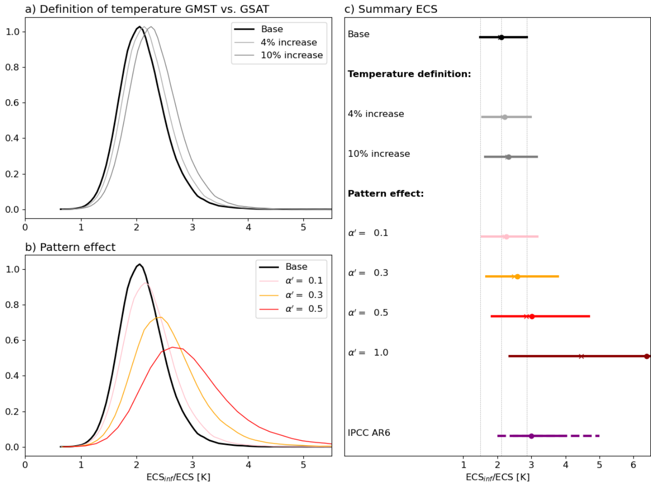
310 Figure 45: Illustrations of reasons for differences between observational estimates of ECS_{inf} and Effective Climate Sensitivity (ECS) as diagnosed from climate models. In a) the influence on ECS by different definitions of temperature is illustrated. The ECS_{inf} estimated in “Base”, based on observations of GMST, are enhanced by 4% and 10% as changes in GMST are larger than GSAT in climate models. In b) different assumptions of the “Pattern Effect” are added to the ECS_{inf} estimate from “Base”. The different values for \alpha' is given in the legend. For “Base” \alpha'=0 . In c) the results are summarized by the mean value (filled circle), median value (x) and 5 th to 95 th percentile range as solid line. Also indicated is the assessed best estimate of Equilibrium Climate Sensitivity from IPCC AR6 (filled circle) and the very likely (solid line) and likely (dashed line) uncertainty range. 315
