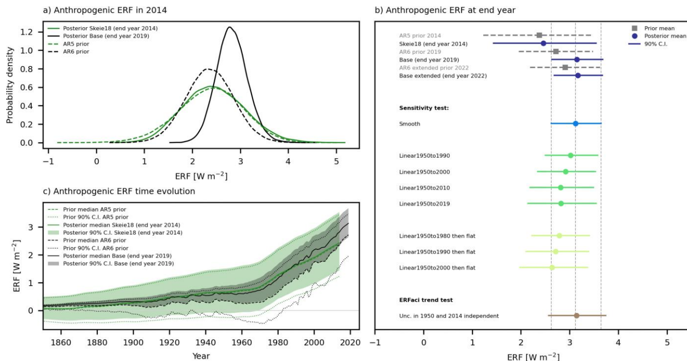
Figure 2: Prior and posterior distributions of anthropogenic ERF. In a) the probability density function of the prior (dashed line) and posterior (solid line) ERF in 2014 for “Base” using AR6 prior (black) and “Skeie18” using AR5 prior (green). In b) the posterior 90% C.I. is indicated by a solid line and the posterior mean as a dot and the prior 90% C.I. is indicated by a dashed line and the prior mean as a square. The results are shown for the end year in the analysis. In c) the prior and posterior time evolutions of the anthropogenic ERF are shown for “Skeie18” and “Base”. The underlying numbers for b) are presented in Table S3.
