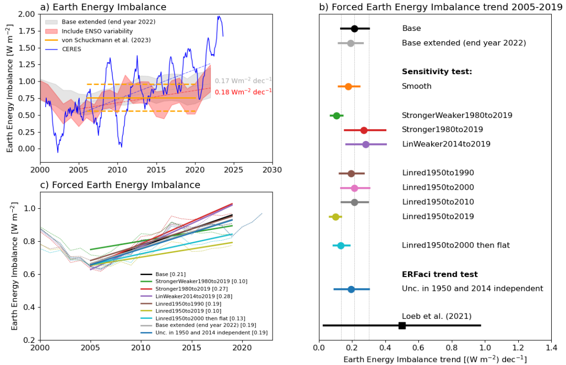
485 Figure 67: Posterior Earth Energy Imbalance and Earth Energy Imbalance trend. In a) the gray shading shows the 5 to 95 490 percentile of the posteriori EEI for the forced temperature response, while the red shading shows the posteriori EEI including ENSO variability for “ Base extended ”. The gray and red dashed line indicate the least squares linear fit for the posterior median of EEI without and with ENSO variability included for the period 2005 to 2022 and the trend over this period are indicated in the plot. The orange lines are the EEI from von Schuckmann et al. (2023) of 0.76 \text{ W m}^{-2} (solid line) \pm 0.2 \text{ W m}^{-2} (dashed lines) for the 90% confidence interval for the period 2006 to 2020. CERES data are shown as a 12-month running mean in blue (Loeb et al., 2018a) (include data for January 2024) and the least squares linear fit from 2005 to 2022 (dashed blue line). In b) the posteriori forced EEI trend over the period 2005 to 2019 are shown as 5 th to 95 th percentile as solid line and median value as a dot. At the bottom the mid-2005 to mid-2019 estimates for the trend for the net CERES TOA energy flux of 0.50 \pm 0.47 \text{ W m}^{-2} \text{ decade}^{-1} (90% 495 confidence interval) from Loeb et al. (2021) are indicated with a black square and the solid line. In c) the posteriori median of the forced EEI from 2000 and onwards are shown for selected sensitivity tests as annual values (dashed lines) and the linear trend from between 2005 to 2019 as solid line. The trends in EEI over this period are indicated in the legend as \text{W m}^{-2} \text{ decade}^{-1} .
