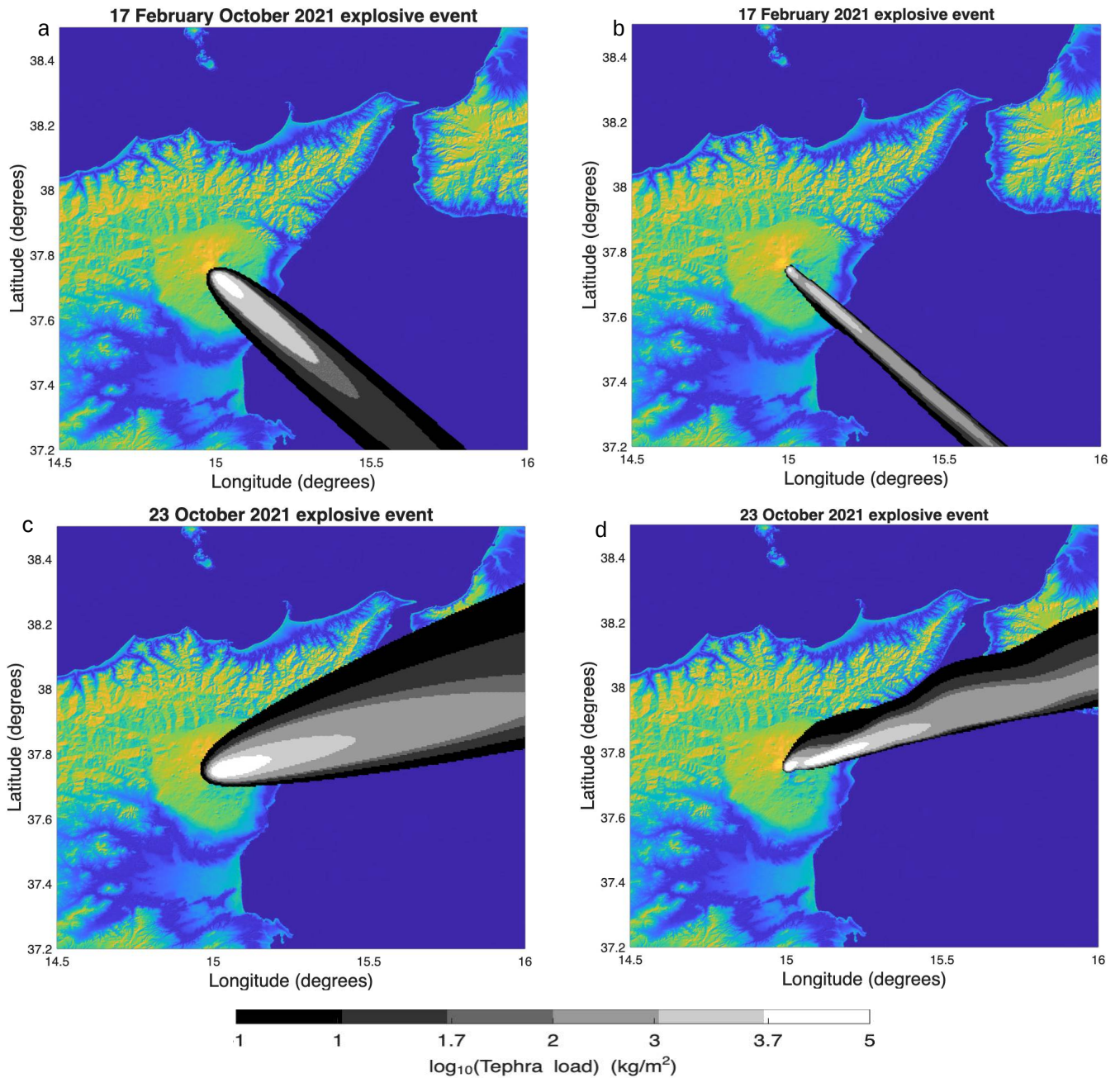
Figure 2: Maps of tephra load ( \text{kg/m}^2 ) for the Etna lava fountain event of 17 February 2021 (a-b)) and of 23 October 2021 (c-d)), using the Tephra2 (a-c)) and Fall3D (b-d)) models. Tephra deposition is plotted as uniform iso-mass contour lines in grayscale, ranging from black for values lower than 10 \text{ kg/m}^2 to light white for values greater than 5 \cdot 10^3 \text{ kg/m}^2 . The colour scale is the same in all panels.
