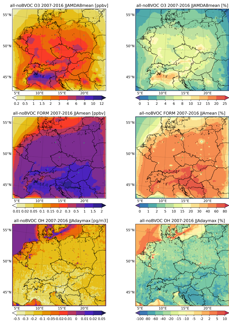
Figure 5. The average JJA impact of all BVOC emissions on the maximum daily 8hour ozone (MDA8; upper row), daily mean formaldehyde and daily max hydroxyl radical near surface concentrations in ppbv for O 3 and HCHO (FORM in figure titles) and in pgm -3 (10 -6 μgm -3 ) for OH. Left columns shows the absolute impact, the right shows the relative contribution in %
