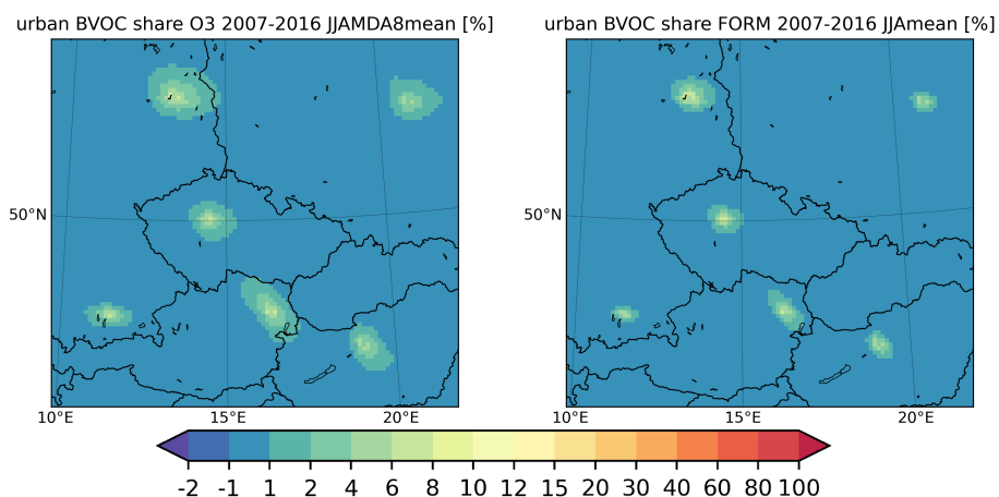
Figure 15. The relative share of the impact of urban BVOC emissions in the total impact in % for the MDA8 ozone (left) and daily mean HCHO (right) averaged over 2007-2016 JJA. The plot is zoomed to the cities analyzed.
