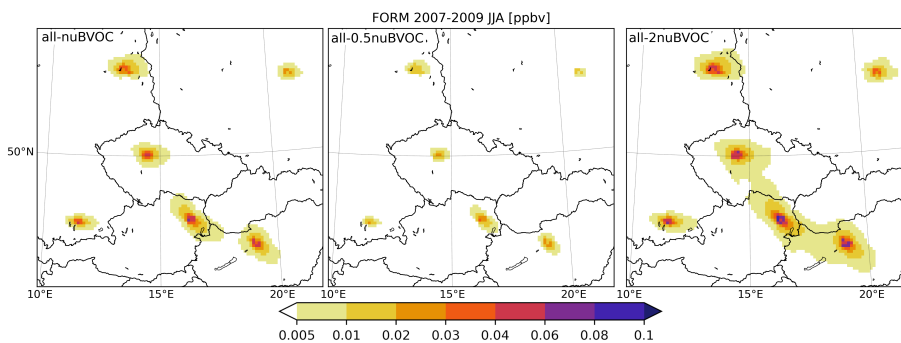
Figure 20. Same as Fig. 19 but for formaldehyde.
