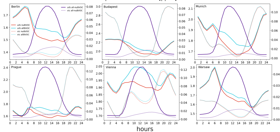
Diurnal variation of FORM and the impact of urbanBVOC [ppbv] for selected cities and their vicinities
