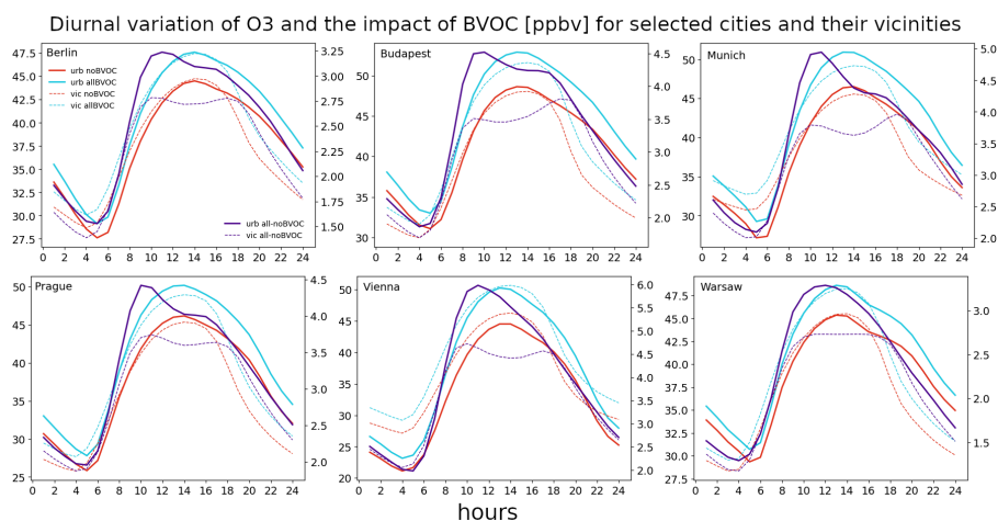
Figure 7. The diurnal cycle of near surface O_3 for 6 city centres (bold) and their vicinities (dashed) for the "noBVOC" (red) and "allBVOC" (cyan). The right y-axis corresponds to the impact of BVOC emissions (allBVOC-noBVOC; violet). Cities are Berlin, Budapest, Munich, Prague, Vienna and Warsaw. Units in ppbv.
