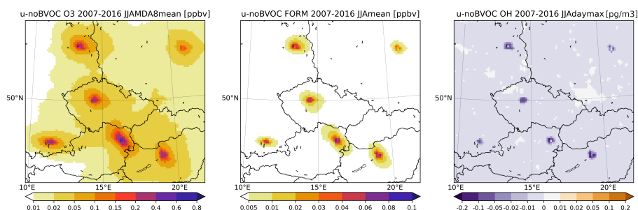
Figure 11. The impact of urban BVOC emissions (calculated alternatively as uBVOC-noBVOC) on the MDA8 ozone (left), daily mean FORM (middle) and maximum daily OH (right) averaged over 2007-2016 JJA. The plot is zoomed to the cities analyzed. Units are ppbv for ozone and FORM, and \text{pgm}^{-3} ( 10^{-6} \mu\text{gm}^{-3} ) for OH.
