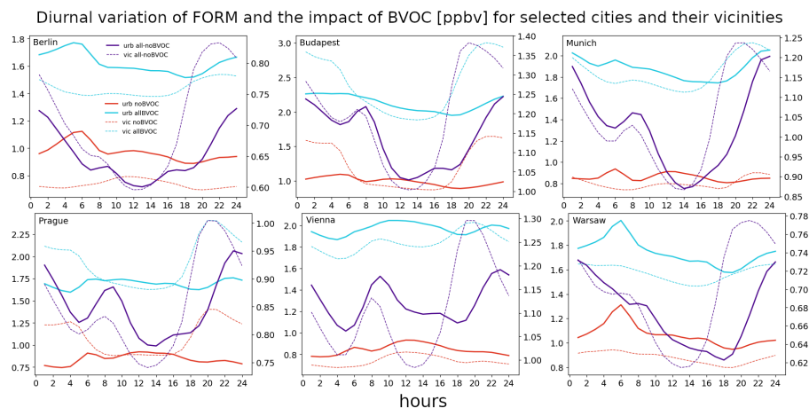
Figure 8. Same as Fig. 7 but for formaldehyde.
