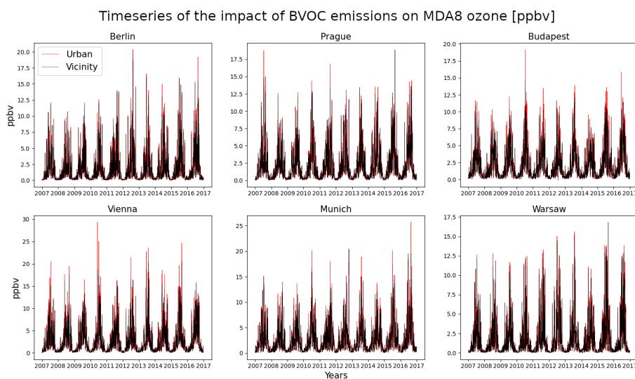
Figure 6. The 2007-2016 timeseries of the BVOC impact of MDA8 ozone for the centres and vicinities of 6 selected cities in ppbv
