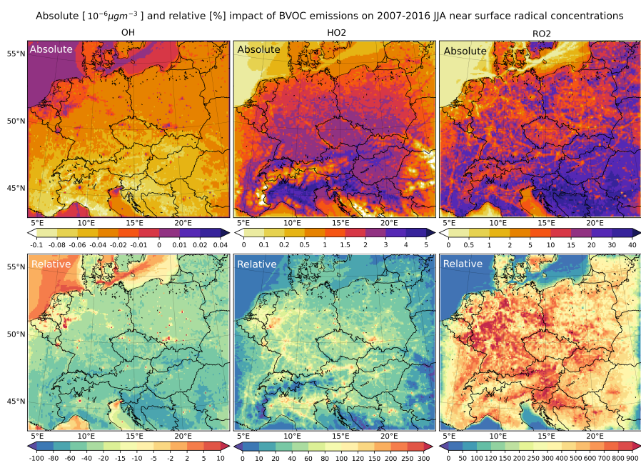
Figure 16. The absolute (top) and relative (bottom) impact of all BVOC emissions on the near surface concentrations of OH (left), HO 2 (middle) and RO 2 (right) averaged over 2007-2016 JJA. Units are \text{pgm}^{-3} ( 10^{-6}\mu\text{gm}^{-3} ) or % for the relative impact.
