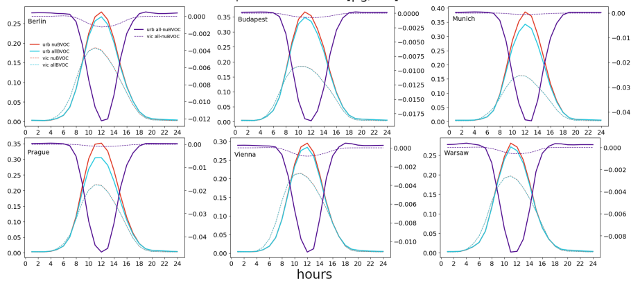
Diurnal variation of OH and the impact of urbanBVOC [pg/m3] for selected cities and their vicinities
