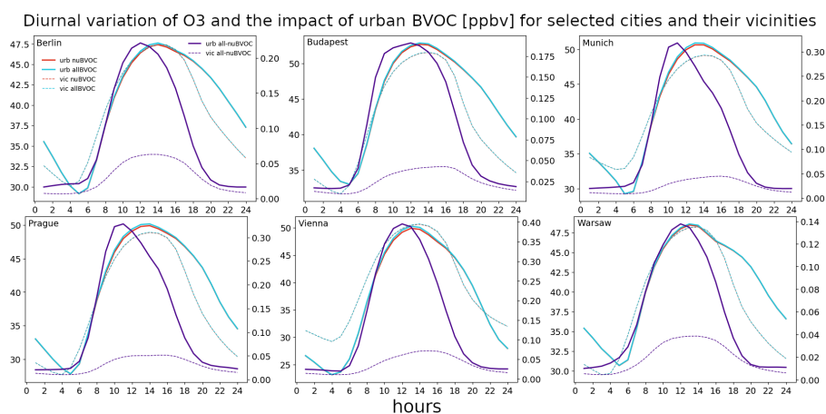
Figure 12. The diurnal cycle of near surface \text{O}_3 for 6 city centres (bold) and their vicinities (dashed) for the "nuBVOC" (red) and "allBVOC" case (cyan). The right y-axis corresponds to the impact of urban BVOC emissions (allBVOC-nuBVOC; violet). Cities are Berlin, Budapest, Munich, Prague, Vienna and Warsaw. Units in ppbv.
