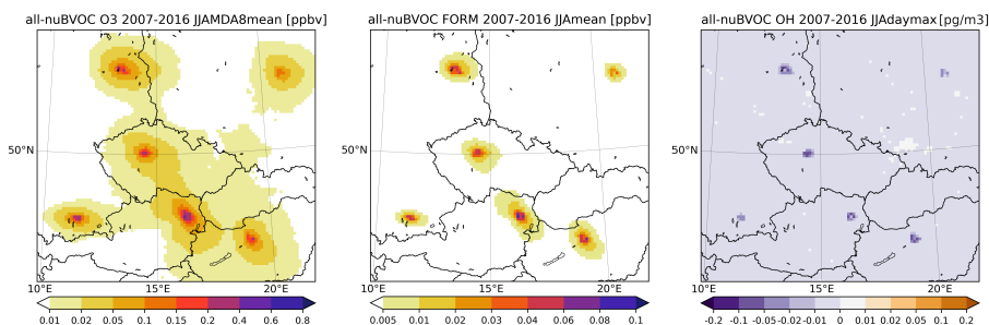
Figure 10. The impact of urban BVOC emissions (calculated as allBVOC-nuBVOC) on the MDA8 ozone (left), daily mean HCHO (middle) and maximum daily OH (right) averaged over 2007-2016 JJA. The plot is zoomed to the cities analyzed. Units are ppbv for ozone and FORM, and \text{pgm}^{-3} ( 10^{-6} \mu\text{gm}^{-3} ) for OH.
