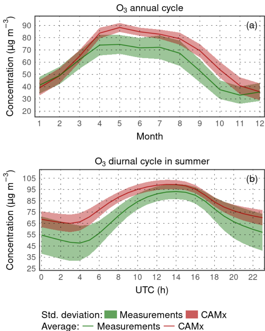
Figure 3. Comparison of modelled surface ozone concentrations with rural background stations for the annual cycle of the average monthly means (a) and average JJA diurnal cycle (b) in \mu\text{g m}^{-3} .
