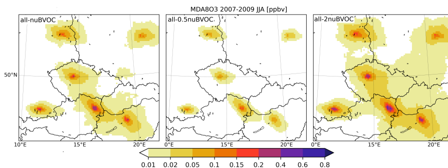
Figure 19. The sensitivity of MDA8 ozone on the amount of urban BVOC emissions in ppbv for the default situation (allBVOC-nuBVOC; left), and the modified urban fraction of the BVOC emissions (allBVOC-0.5nuBVOC; middle and allBVOC-2nuBVOC; right) averaged over 2007-2009 JJA. The plot is zoomed to the cities analyzed.
