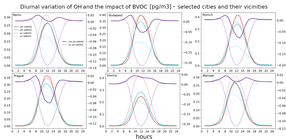
Figure 9. Same as Fig. 7 but for OH and in \text{pgm}^{-3} ( 10^{-6} \mu\text{gm}^{-3} ).
