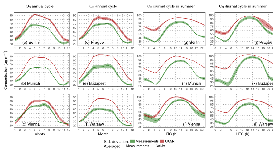
Figure 4. Comparison of modelled surface ozone concentrations with urban background stations from six selected city for the annual cycle of the average monthly means (a-f) and average JJA diurnal cycle (g-l) in \mu\text{g m}^{-3} .
