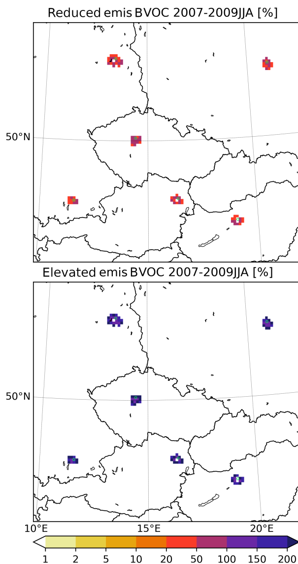
Figure 18. The urban BVOC emission used in the 0.5nuBVOC (top) and 2nuBVOC (bottom) experiments relative to the default urban emission fluxes seen in Fig. 1. Units in %.
