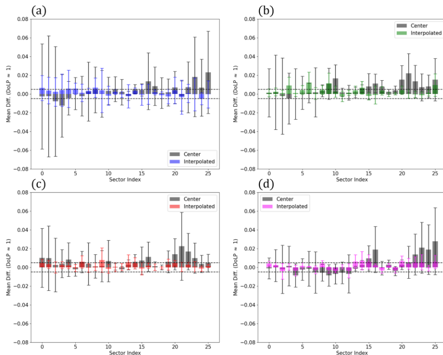
Figure 8: Graphs indicating the degree of linear polarization calibration performance of the center FOV calibration matrix (grey) applied across all sectors in the 26-Sector scan (See figure-Figure 2 ) and the performance of matrices generated from paraboloid fitting of the calibration matrix (colored by spectral band, or in order of blue, green, red, and near-infrared referred to also as a, b, c, d here). Bar heights indicate the mean absolute difference of only the fully polarized data (DoLP ≈ approximately 1) as compared to the result from each sector's independent calibration matrix. Error bars indicate the standard deviation of same. Dotted lines indicate a \pm 0.5 uncertainty.
