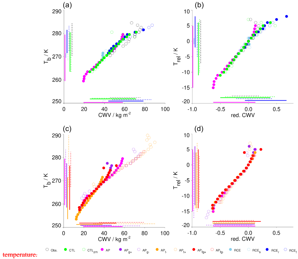
Figure 5. Precipitation onset curves. In (a) and (c) an open or filled circle marks the average CWV at which precipitation rates reach 2 \text{ mm h}^{-1} for each bulk temperature T_b ( y -axis). Lines along the axes mark the range covered by the respective 2 \text{ mm h}^{-1} isoline of a simulation. (b) and (d) repeat (a) and (c) in the phase space of reduced CWV and relative temperature T_{\text{rel}} = T_b - T_m .
