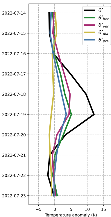
Figure 12. Same as Fig. 5, but the \theta' decomposition terms are now depicted as deviations from their long-term averages.
