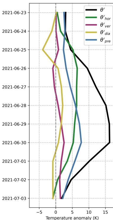
Figure 10. Same as Fig. 2, but the \theta' decomposition terms are now depicted as deviations from their long-term averages.
