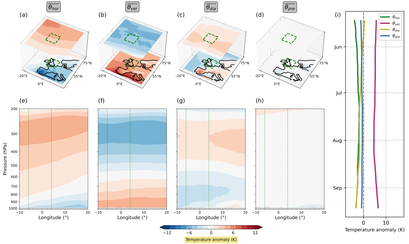
Figure 8. Long-term average (2010-2022) of the \theta' decomposition for the UK region. Panels (a) to (h) depict the long-term averages during that time of the year the UK heat wave happened (16 to 20 July). Panel (i) shows the evolution of the near-surface \theta' decomposition during the summer season, averaged over the UK heat wave region. The 3D plots in panels (a) to (d) are analogous to those in Fig. 5b–p) and the vertical cross-sections in panels (e) to (h) are analogous to those in Fig. 6b–e.
