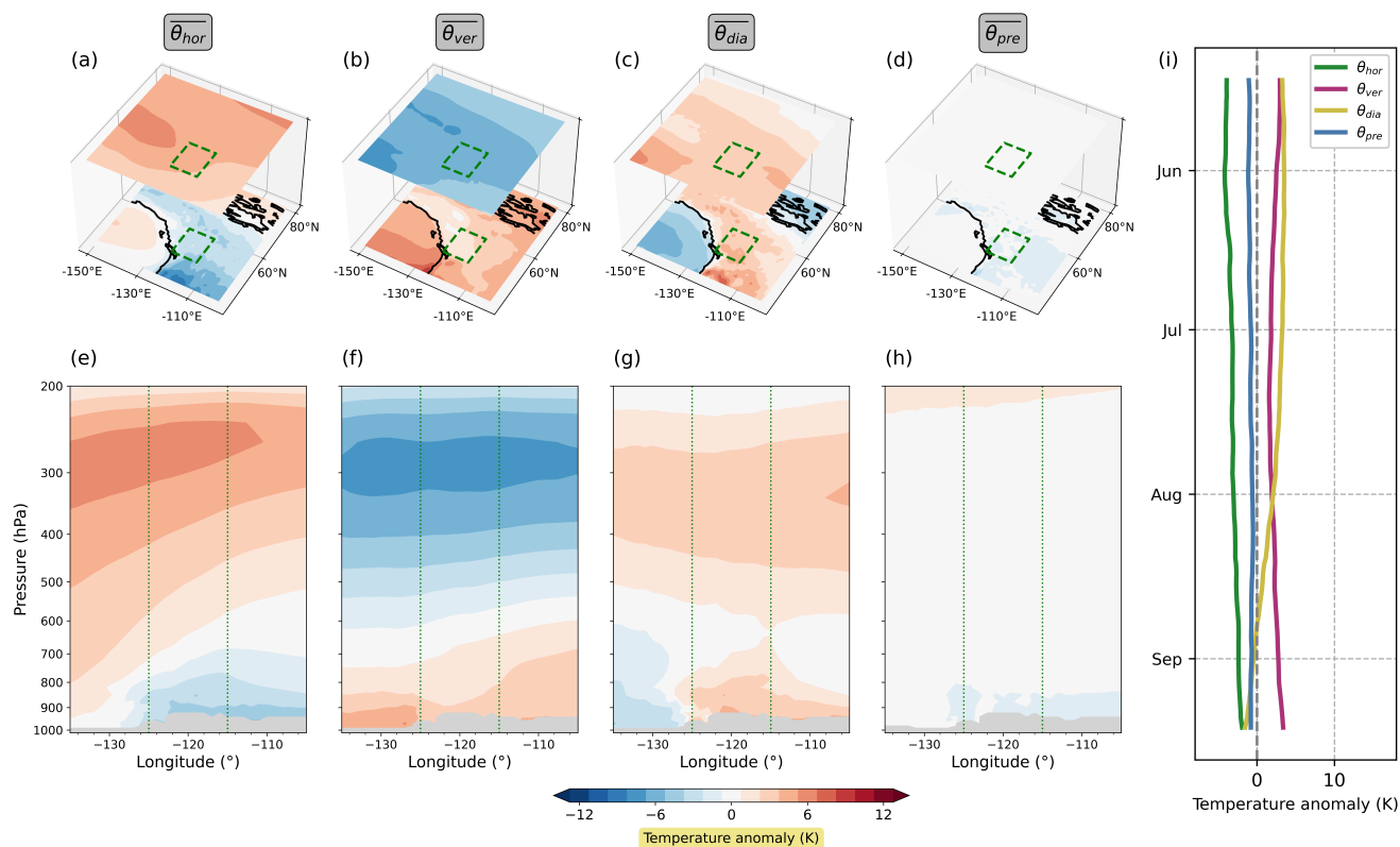
Figure 7. Long-term average (2010-2022) of the \theta' decomposition for the Pacific Northwest. Panels (a) to (h) depict the long-term averages during that time of the year the Pacific Northwest heat wave happened (27 June to 1 July). Panel (i) shows the evolution of the near-surface \theta' decomposition during the summer season, averaged over the Pacific Northwest heat wave region. The 3D plots in panels (a) to (d) are analogous to those in Fig. 2b–p) and the vertical cross-sections in panels (e) to (h) are analogous to those in Fig. 3b–e.
