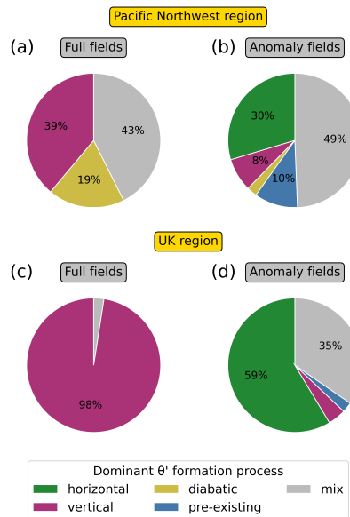
Figure 15. Pie charts displaying the relative frequency of the dominant near-surface \theta' formation processes for hot days during summer in (a)–(b) the Pacific Northwest region and (c)–(d) the UK region. A single process is considered dominant if it contributes at least 1.5 times as much as the second-placed term. If no single process is identified as dominant, the day is counted as "mix". The pie charts are based on area mean values. In (a) and (c) the pie charts are based on the \theta' decomposition in terms of full fields, whereas in (b) and (d) the pie charts are based on the \theta' decomposition in terms of anomaly fields.
