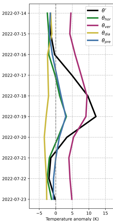
Figure 5. Evolution of the potential temperature anomaly \theta' and its decomposition into contributions from horizontal transport, vertical transport, diabatic heating, and pre-existing anomaly during the UK heat wave. The time series have been obtained by averaging the different terms over the lowest 50 hPa above the surface within the UK heat wave region (6°W–4°E, 49–59°N).
