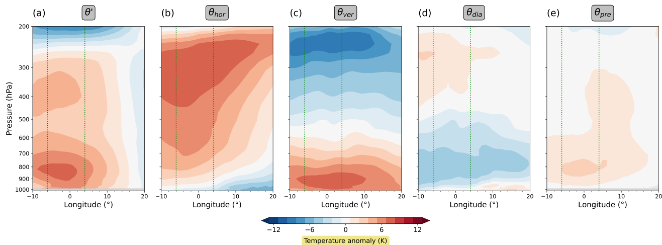
Figure 6. Five-day mean (16 July–20 July 2022) vertical cross-sections showing the \theta' decomposition during the UK heat wave. Fields are latitudinally averaged between 49–59°N. The panels show (a) the potential temperature anomaly \theta' , (b) the contribution from horizontal transport, (c) the contribution from vertical transport, (d) the contribution from diabatic heating, and (e) the contribution from the pre-existing anomaly. The two green vertical lines in each panel indicate the longitudinal extent of the UK heat wave region.
