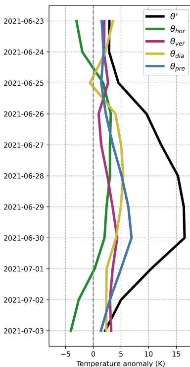
Figure 2. Evolution of the near-surface potential temperature anomaly \theta' and its decomposition into contributions from horizontal transport, vertical transport, diabatic heating, and pre-existing anomaly during the Pacific Northwest heat wave. The time series have been obtained by averaging the different terms over the lowest 50 hPa above the surface within the Pacific Northwest heat wave region.
