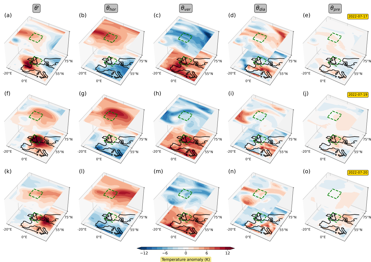
Figure 4. Illustration of the 3D structure of \theta' and its contributions from horizontal transport, vertical transport, diabatic heating, and pre-existing anomaly for three selected dates (17 July, 19 July, and 20 July 2022). The upper layer depicts fields averaged between 300 – 400 hPa, and the lower layer depicts fields near the surface. The green rectangle indicates the UK heat wave region.
