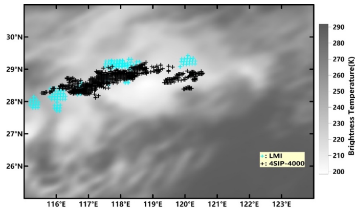
225 Figure 4. The simulated and observed lightning locations during the storm. The shaded field indicates brightness temperature. The simulated results are from the 4SIP-4000 experiment.
