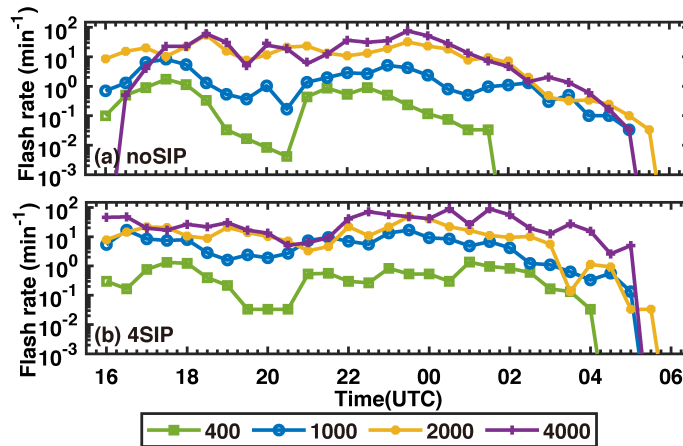
480 Figure 17. Time evolution of the flash rate for the noSIP experiment and 4SIP experiment.
