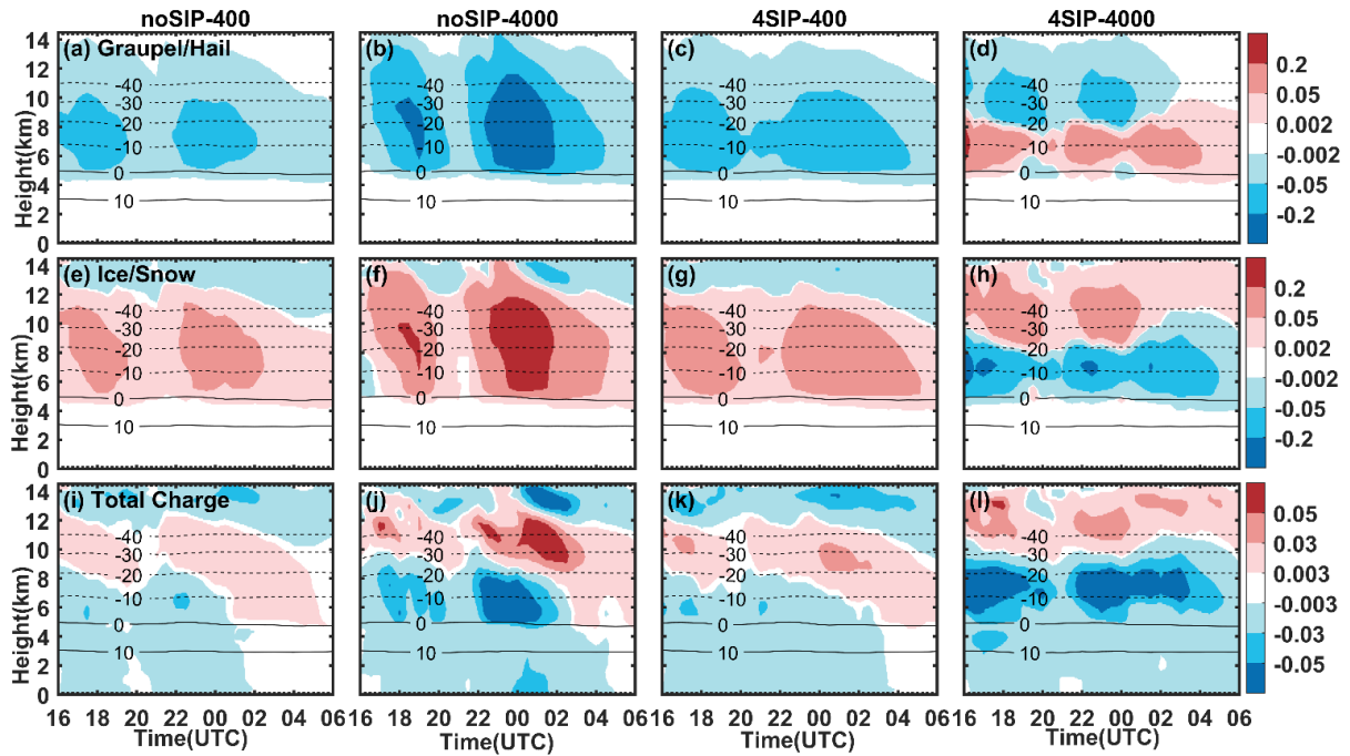
435 Figure 14. Time-height evolution of mean charge carried by graupel/hail (a-d) and ice/snow (e-h) particles as well as mean total space charge (i-l) (unit is nC m^{-3} ) for four sensitivity experiments. The first to fourth columns represent the results from noSIP-400, noSIP-4000, 4SIP-400 and 4SIP-4000 experiment, respectively.
