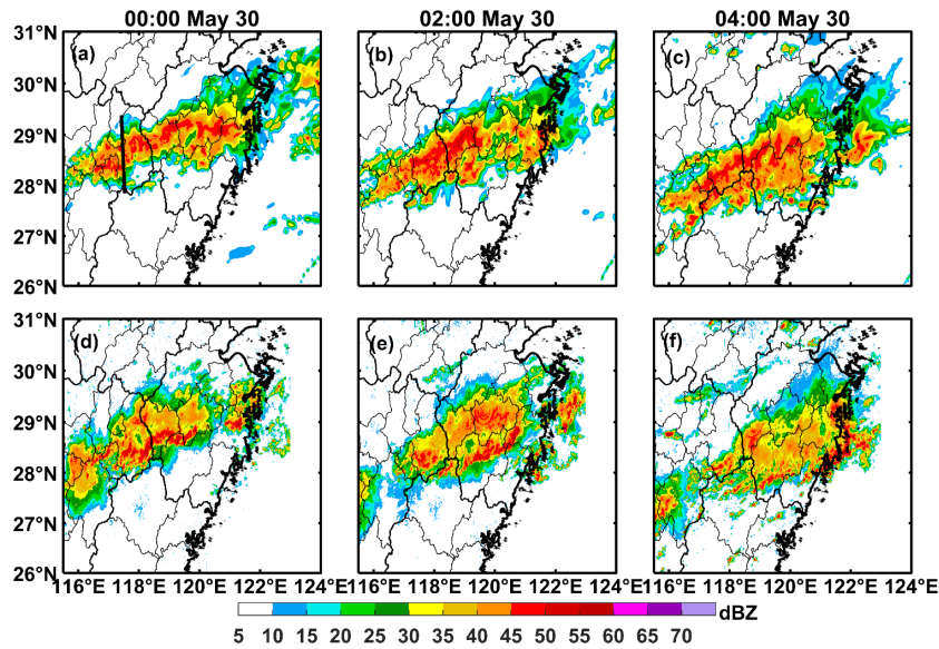
215 Figure 3. The (a-c) simulated and (d-f) observed radar reflectivity at 00:00, 02:00, and 04:00 on 30th May. The vertical black line in (a) shows the cross-section used in the subsequent investigation. The simulated results are from the 4SIP-4000 experiment.
