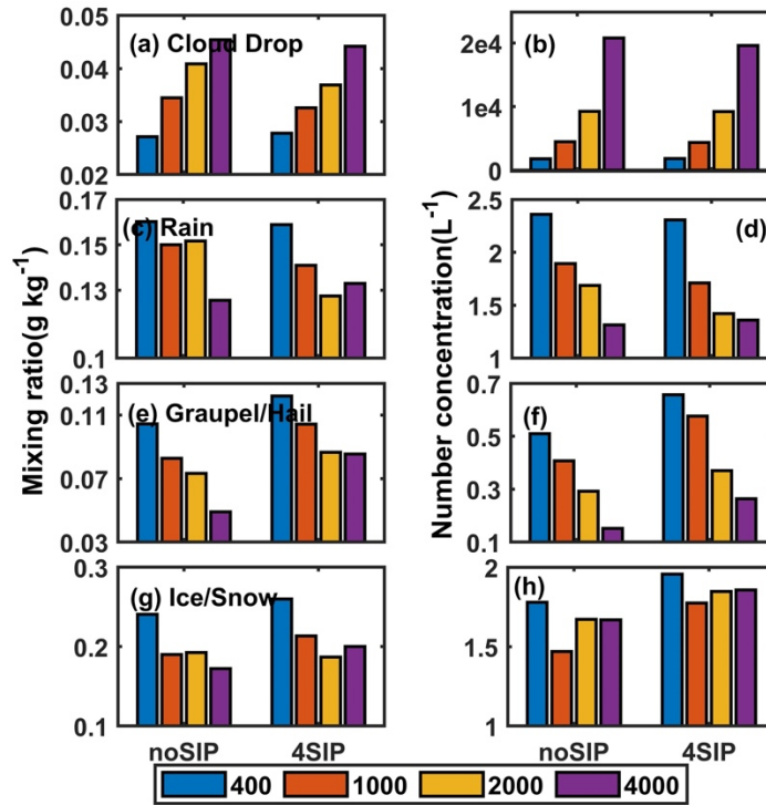
305 Figure 8. The time-domain-averaged mixing ratios (a, c, e, g) and number concentrations (b, d, f, h) of (a, b) cloud drop, (c, d) rain, (e, f) graupel/hail and (g, h) ice/snow from 8 sensitivity experiments.
