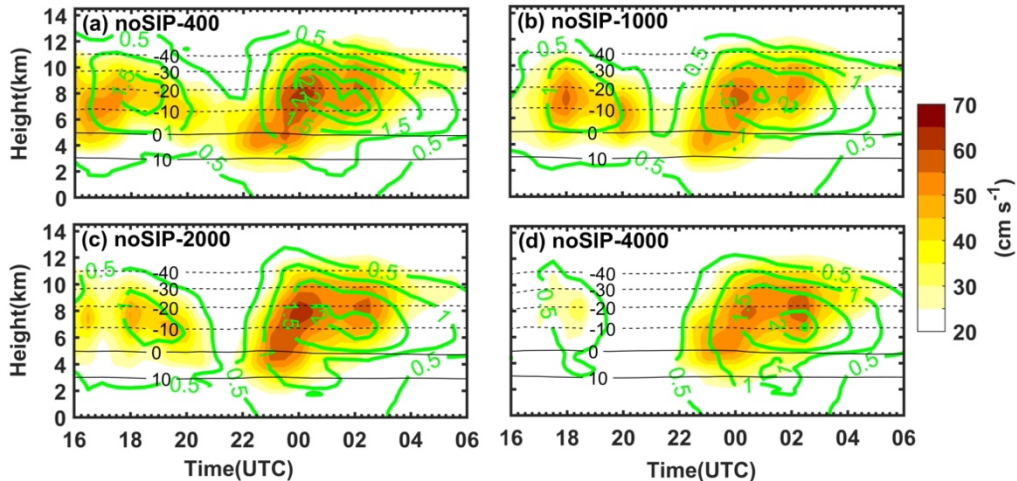
310 Figure 9. Time-height evolution of mean vertical wind velocity (cm/s, shaded) of (a) noSIP-400, (b)noSIP-1000, (c)noSIP-2000, (d)noSIP-4000. Green contour lines show all hydrometeors mixing ratio of 0.5, 1.0, 1.5, 2.0 and 2.2 g/kg.
