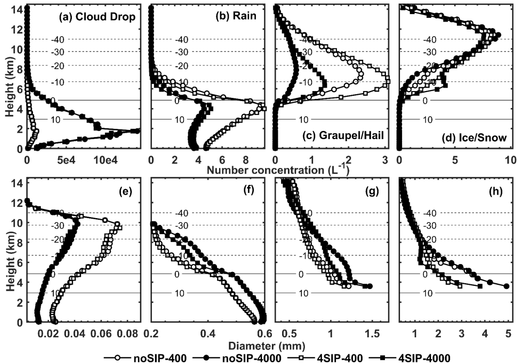
280 Figure 7. The vertical profiles of mean concentration (upper row) and mean diameter (lower row) of (a, e) cloud drop, (b, f) rain, (c, g) graupel/hail and (d, h) ice/snow from noSIP-400, noSIP-4000, 4SIP-400 and 4SIP-4000 experiment.
