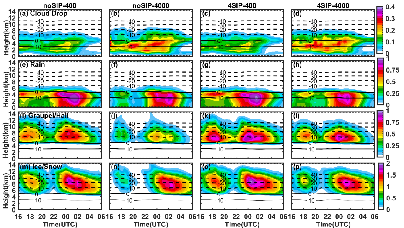
260 Figure 6. Time-height evolution of the mean mixing ratio (unit is g/kg) of four particles for four sensitivity experiments. (a-d) cloud drop, (e-h) rain, (i-l) graupel/hail, (m-p) ice/snow. The first to fourth columns represent the results from noSIP-400, noSIP-4000, 4SIP-400 and 4SIP-4000, respectively.
