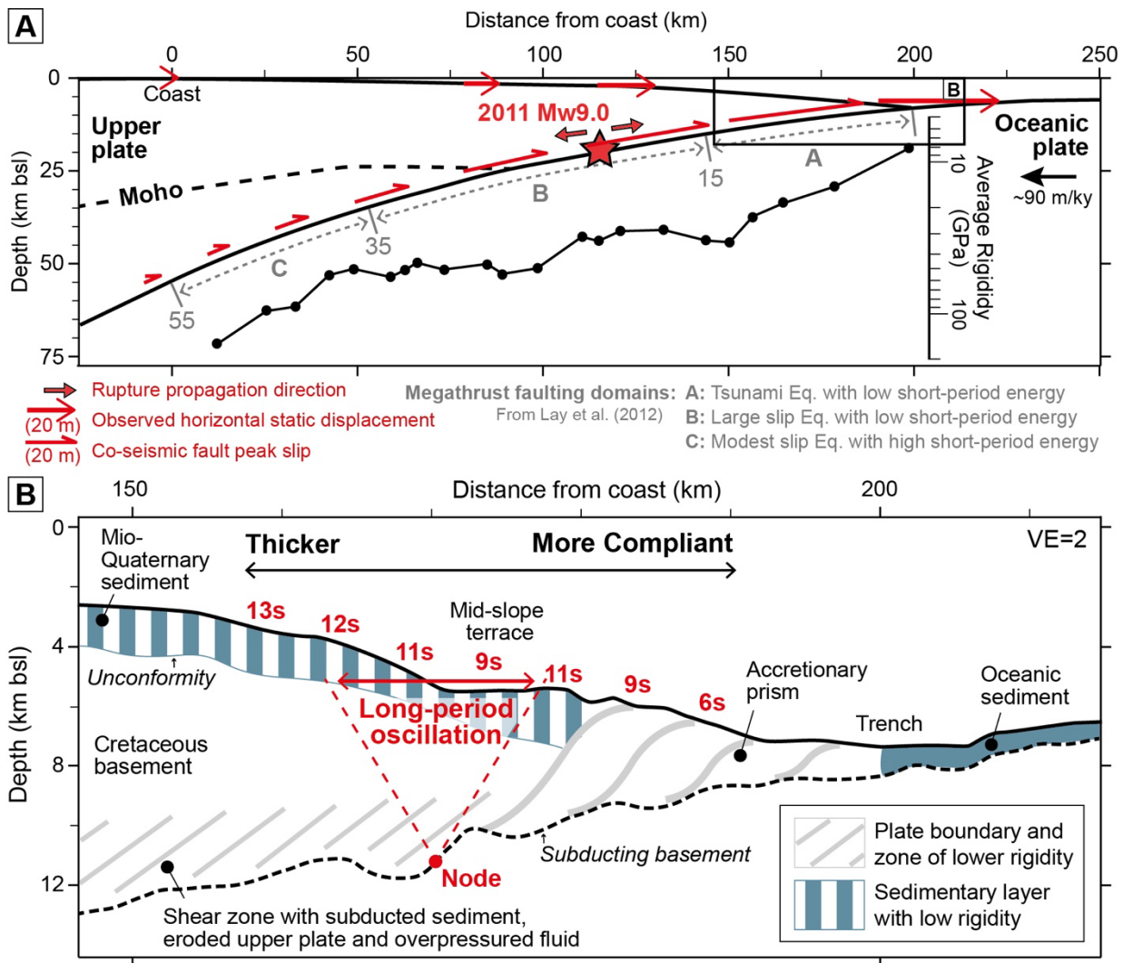
95 Figure 1: Profile across the Japan active margin at the 2011 Mw9.0 Tohoku-Oki megathrust rupture. A. Schematic cross section showing hypocenter and rupture initiation (red start) and megathrust domains A, B and C modified from Lay et al. (2012). Mean values of rigidity in depth bins from seismic-rupture radiation averaged for a number of megathrusts (Lay and Bilek, 2007). Note order of magnitude increase across the seismogenic range. Red half-arrows show peak co-seismic slip from Lay et al. (2012). Red arrows show the horizontal static displacement from Yue and Lay (2013). B. The outer upper plate above the largest 2011 rupture displacements (based on MCS profile D11 from Kodaira et al., 2017). In red, periods of fundamental-mode horizontally polarized oscillation with nodes at the top of the subducting slab and “crests” at the seafloor (Supplementary 1). The landward increases in wedge thickness and S-wave velocity (i.e., rigidity; Von Huene et al., 1994; Fujiwara et al., 2011) allow for a ~20km wide plateau in fundamental periods at ~10s centered on the Mid-Slope Terrace. 100
