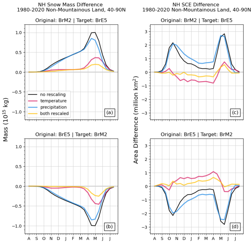
355 Fig. 5 (a, b) NH snow mass and (c, d) snow cover extent differences for MERRA-2 and ERA5 calculated as original minus target . Each panel shows the difference between the original and target snow mass climatologies (black) and the coloured lines represent the datasets generated by adjusting temperature (pink), precipitation (blue), or both (yellow) to the target dataset's climatology.
