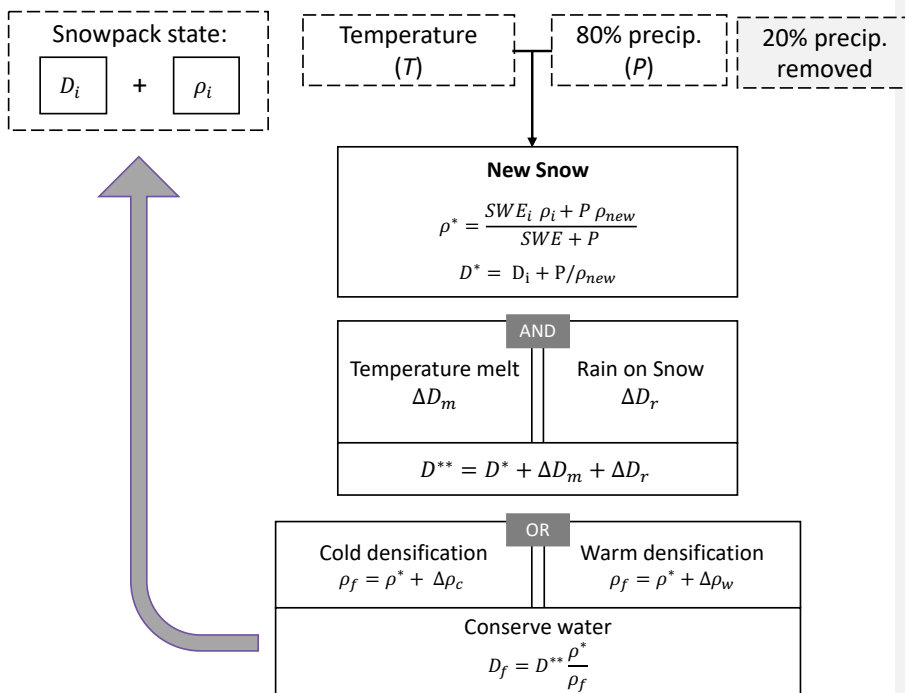
110 Fig. 1 Conceptual overview of the Brown Temperature Index Model (B-TIM). At every time step and location, temperature and precipitation values are used to compute either the density and depth of any new snow or the temperature of any rainfall. The snowpack state (snow depth and density) is affected by rain melt, melting due to air temperature, and one of two densification processes which cause both depth and density variables to evolve.
