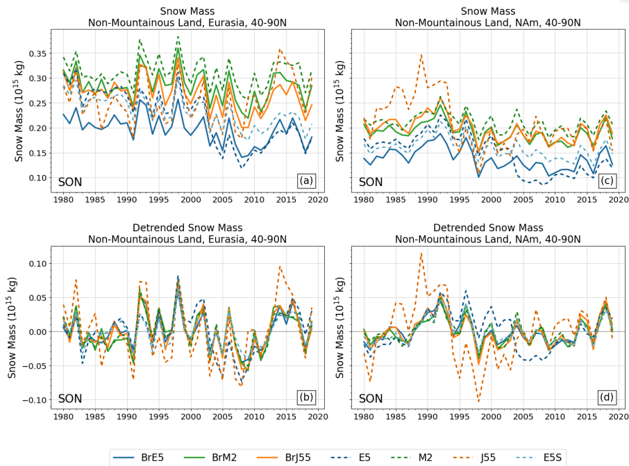
Fig. 6 Time series of total snow mass for SON by continent. Lower row has linear trends removed.
