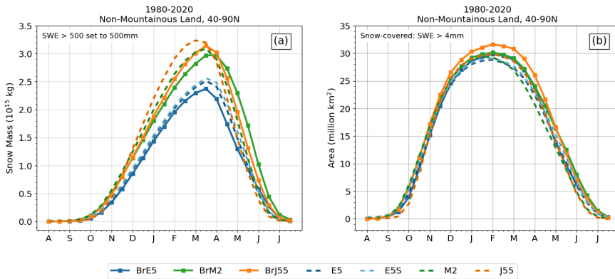
340 Fig. 4 (a) Snow mass climatology over Northern Hemisphere land, with grid cells exceeding 500 mm capped at 500 mm. 341 (b) Snow-covered area climatology, calculated using areas of grid cells with more than 4 mm SWE.
