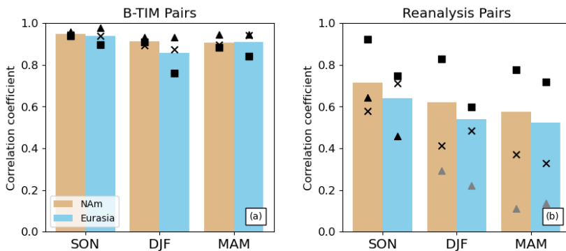
440 Fig. 8 (a) Correlation coefficients for B-TIM dataset pairs. Individual values are shown with black points, and the mean is represented by the height of the bar to summarize the group. Similar information is shown in Fig. 8 (b) for the reanalysis dataset pairs. The ERA5 and JRA-55 pair is represented by the triangle, ERA5 and MERRA-2 by the square, and JRA-55 and MERRA-2 with the x.
