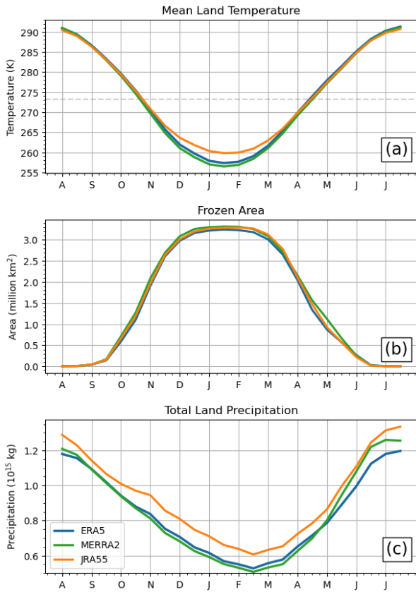
Fig. 2 Climatologies of mean temperature, frozen area, and total precipitation over Northern Hemisphere land areas, excluding mountains , computed twice monthly using 14-day windows centred on the 1 st and 15 th of each month.
