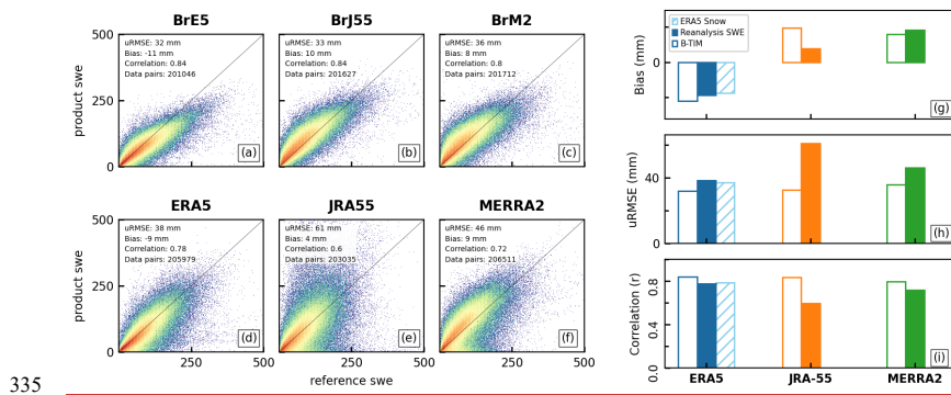
335 Fig. 3 SWE product validation against snow course and gamma SWE measurements. Figs. 3a-f consist of scatterplots showing all valid data pairs (snow course, product) from November to March over 1980-2018. Summary statistics, including the bias, unbiased root mean squared error (uRMSE), and correlation, are included in the legend and are summarized in Figs. 3g-i.
