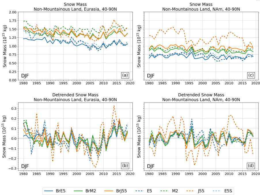
435 Fig. 7 Time series of total snow mass for DJF by continent. Lower row has linear trends removed.
