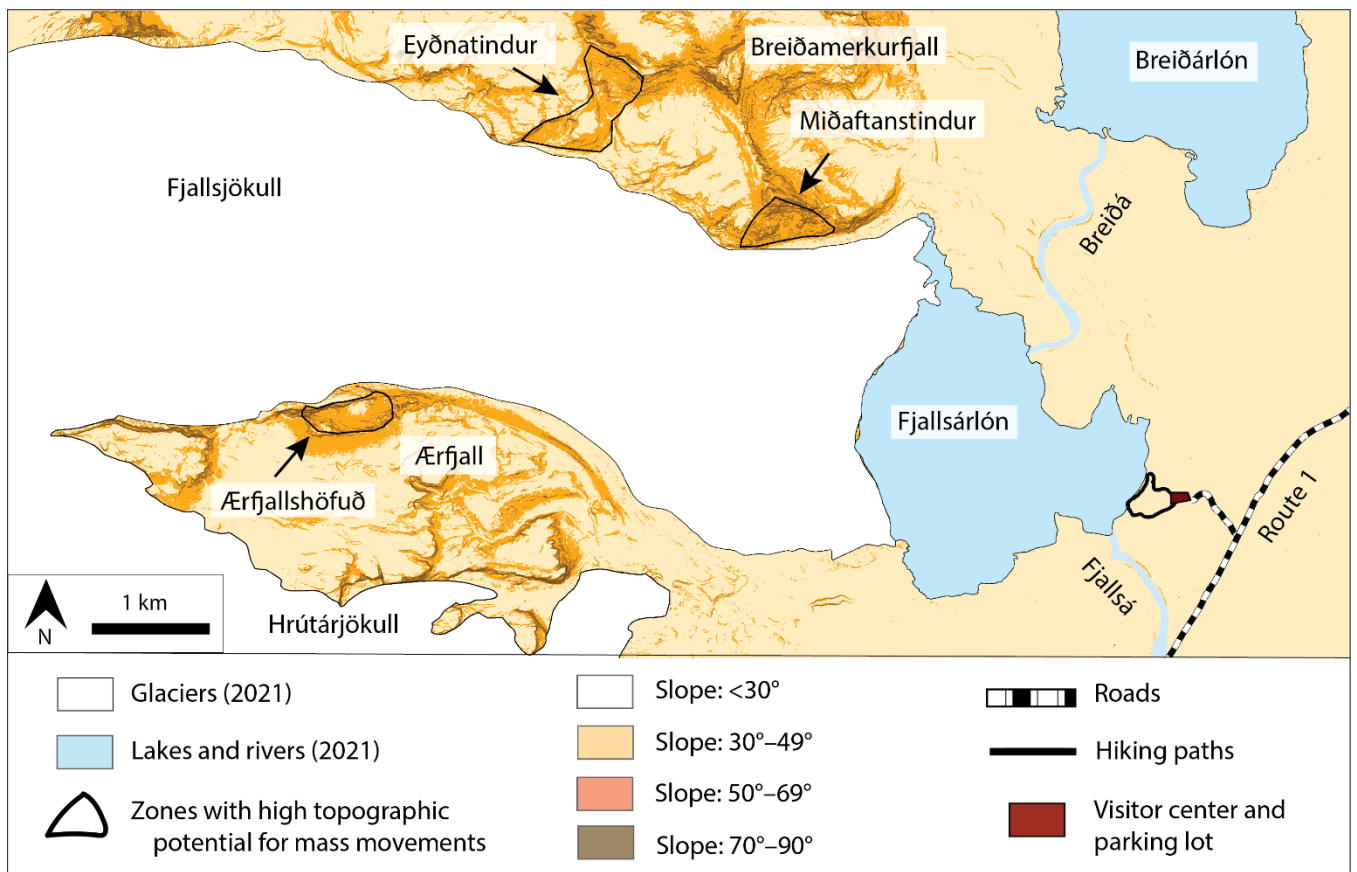
Figure 6. Slope angles on subaerial terrain in study area based on 2021 glacier and lake extent. Delineated zones show areas in valley walls above Fjallsjökull with slope angles >30^\circ and vertical relief >200 m, indicating high topographic potential to source large mass movements. ÍslandsDEM basemap with slope shading in ArcGIS Pro (Landmælingar Íslands, 2021).
