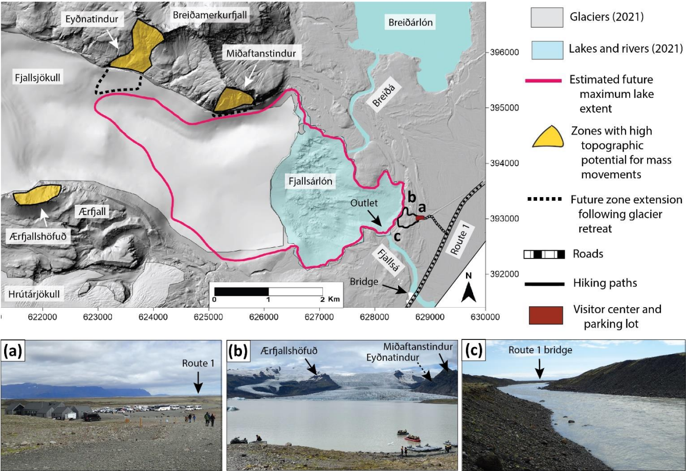
540 Figure 8. Map illustrating potential societal and landscape impacts of mass movement-triggered displacement waves or GLOFs in Fjallsárlón. Bed DEM basemap with ISN93 coordinate system. Photos (a)–(c) correspond to locations marked on the map: (a) View looking northeast towards the visitor center, parking lot, and Route 1. (b) View looking west towards Fjallsjökull showing hiking trails and boat launches along the lakeshore, with high topographic potential zones marked. (c) View looking southeast along the Fjallsá outlet towards the Route 1 bridge.
