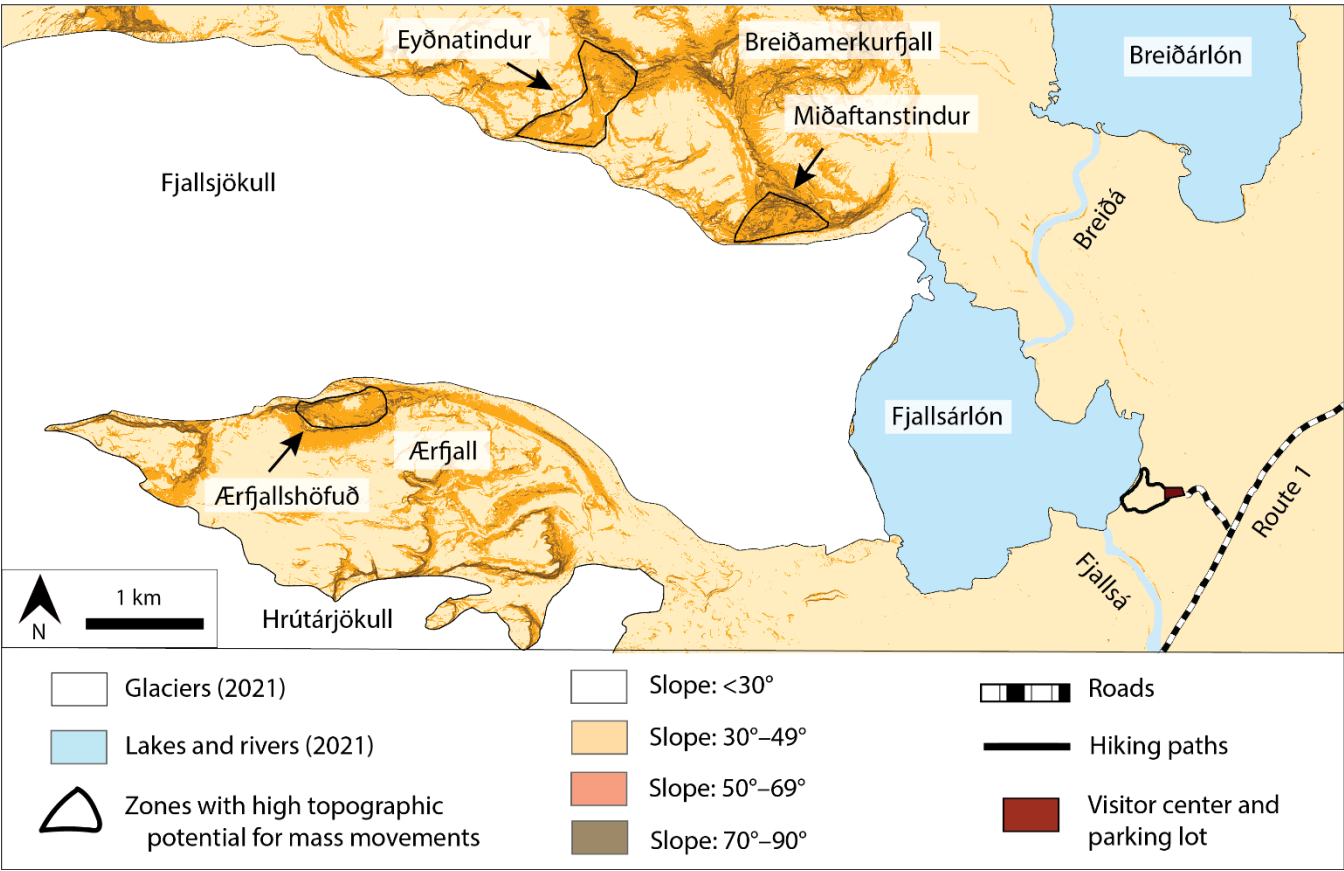
Figure 6. Slope angles on subaerial terrain in study area based on 2021 glacier and lake extent. Delineated zones show areas in valley walls above Fjallsjökull with slope angles >30° and vertical relief >200 m, indicating high topographic potential to source large mass movements. ÍslandsDEM basemap with slope shading in ArcGIS Pro (Landmælingar Íslands, 2021).
