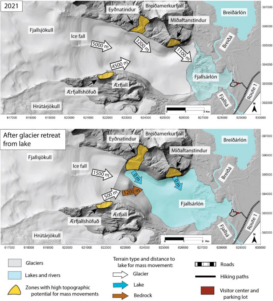
465 Figure 7. Scenarios of mass movements entering Fjallsárlón based on glacier and lake positions in 2021 and at the estimated maximum lake extent after Fjallsjökull has retreated completely from the lake. Bed DEM basemap with ISN93 coordinate system.
