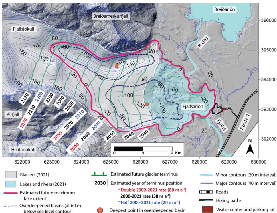
Figure 4. Bed DEM showing overdeepened basins and estimated future development of Fjallsarlón extents and Fjallsjökull terminus positions from 2030–2120 for three terminus retreat rates, assuming linear rates and 2020 lake surface elevation (5 m a.s.l.). Bed DEM uses ISN93 coordinate system.
