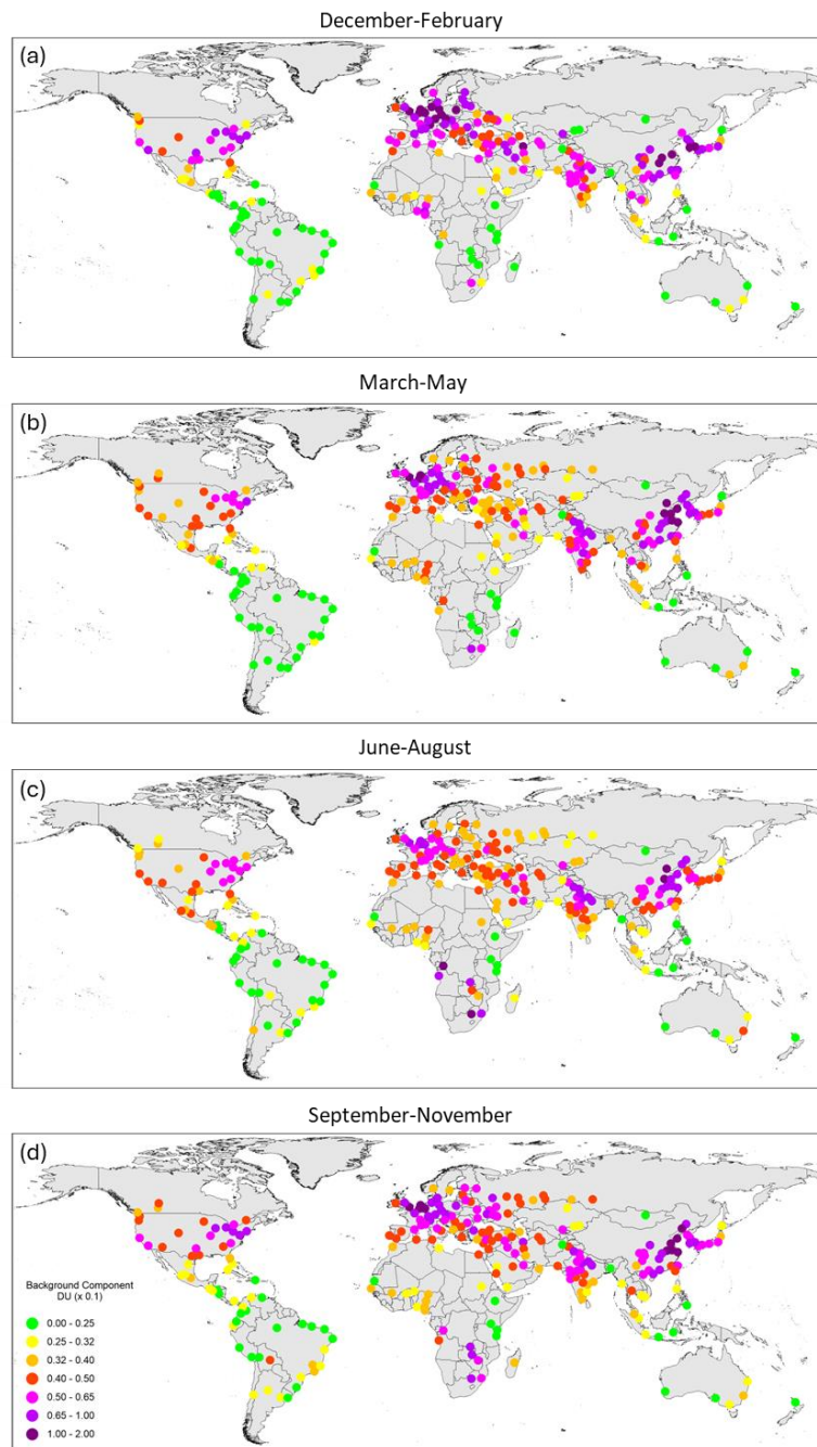
Figure 2. The mean \text{NO}_2 background component in tenths of a Donson Unit DU ( \times 0.1 ) for individual cities for (a) December-February, (b) March-May, (c) June-August, and (d) September-November. The background component represents the mean tropospheric \text{NO}_2 VCD when a direct contribution from urban and industrial emissions is removed.
