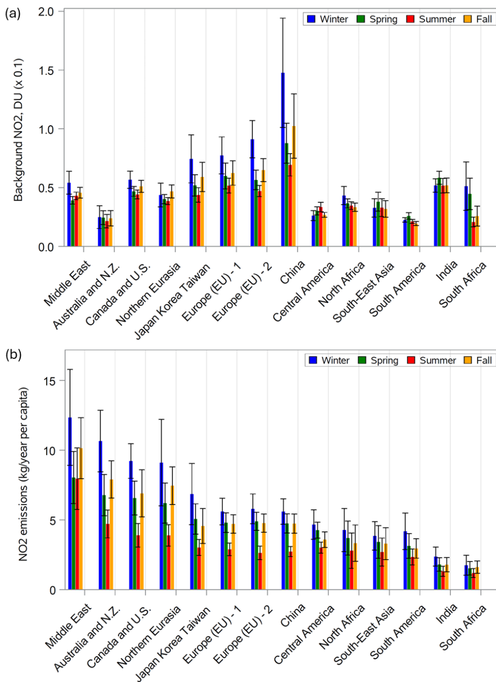
Figure 3. (a) The mean background component in tenths of a Donson Unit for 14 regions for four seasons. Mean values for each region were calculated as a mean of the values from all areas for that region. (b) The mean values of urban NO x emissions per capita reported at NO 2 emissions per capita for the same regions. The uncertainty ( \sigma ) was calculated as a standard error of
