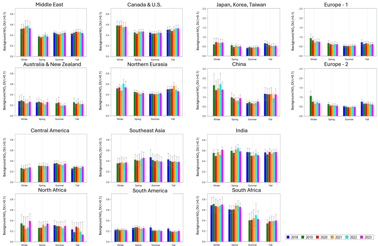
Figure 9. The regional mean background component in tenths of a Donson Unit ( \text{DU} (\times 0.1) ), 2018-2023 for individual seasons.
