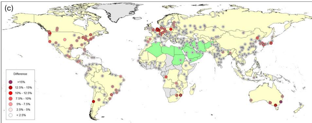
Figure 6. The percentage difference between background components on Monday-Thursday and those on (a) Friday, (b) Saturday, and (c) Sunday. Cities where the difference is below 3-sigma level are marked by large gray dots and between 3- and 5-sigma level by small gray dots. Countries where Sunday is a rest day are in yellow, countries where Friday is a rest day are in green.
