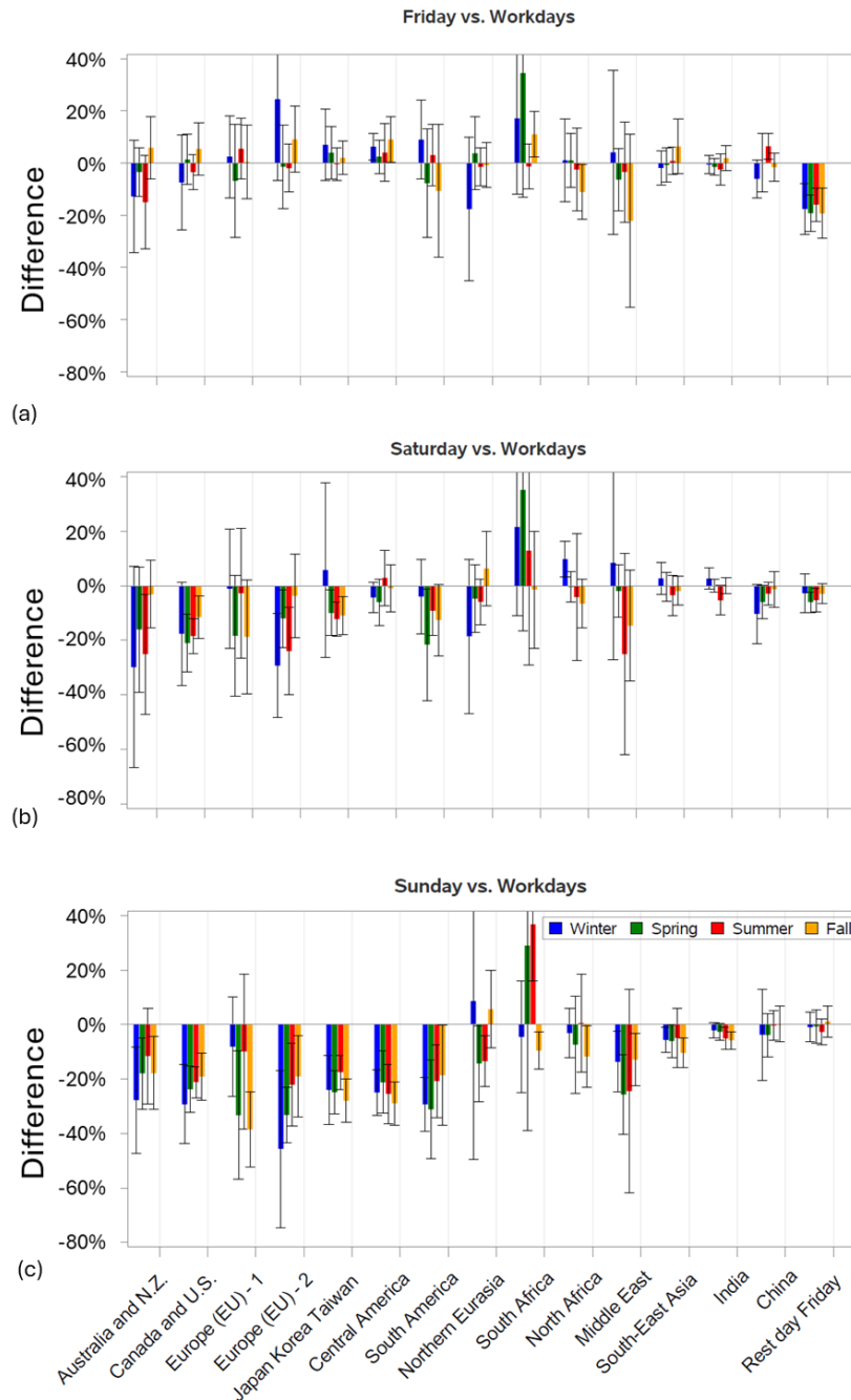
Figure CB1. The percentage difference between industrial components on Monday-Thursday and those on (a) Friday, (b) Saturday, and (c) Sunday for different regions in different seasons. The uncertainty ( \sigma ) was calculated as a standard error of the mean. The error bars represent 2\sigma intervals.
