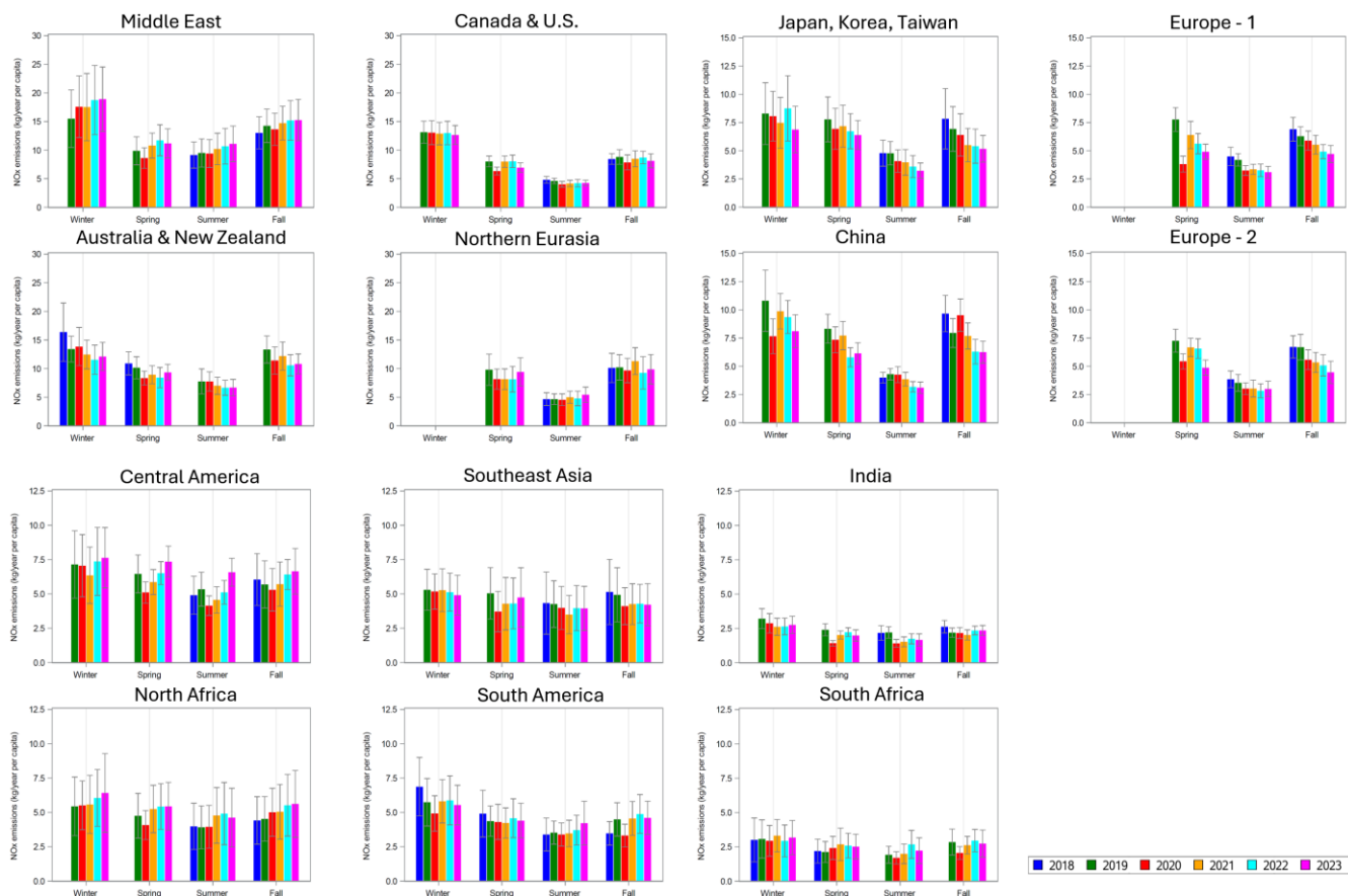
Figure A2. Similar to Fig. 10, but for NO x emissions. The regional mean urban NO x emissions in kt y -1 per capita by region, 2018-2023 for individual seasons estimated using Model 12 . The error bars represent 2σ intervals.
