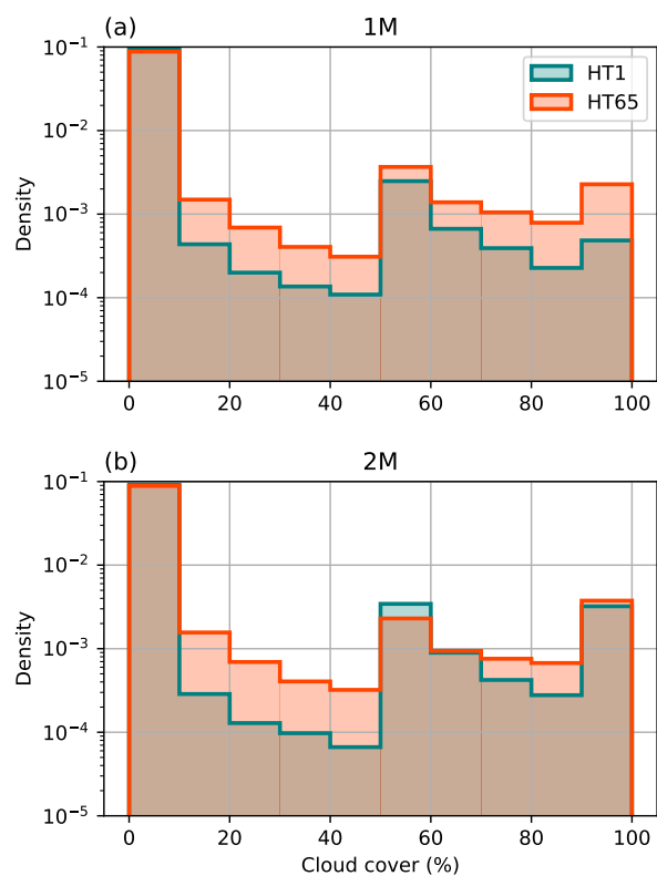
Figure A1. Probability density figures for the cloud cover (%) of HT1 (teal) and HT65 (red) with 1M (a) and 2M (b) over all five minute model output time steps and all height levels, where the cloud was present. The domain and time period included in this analysis is the same as in Fig. 3. The bin width is set to 10%.
