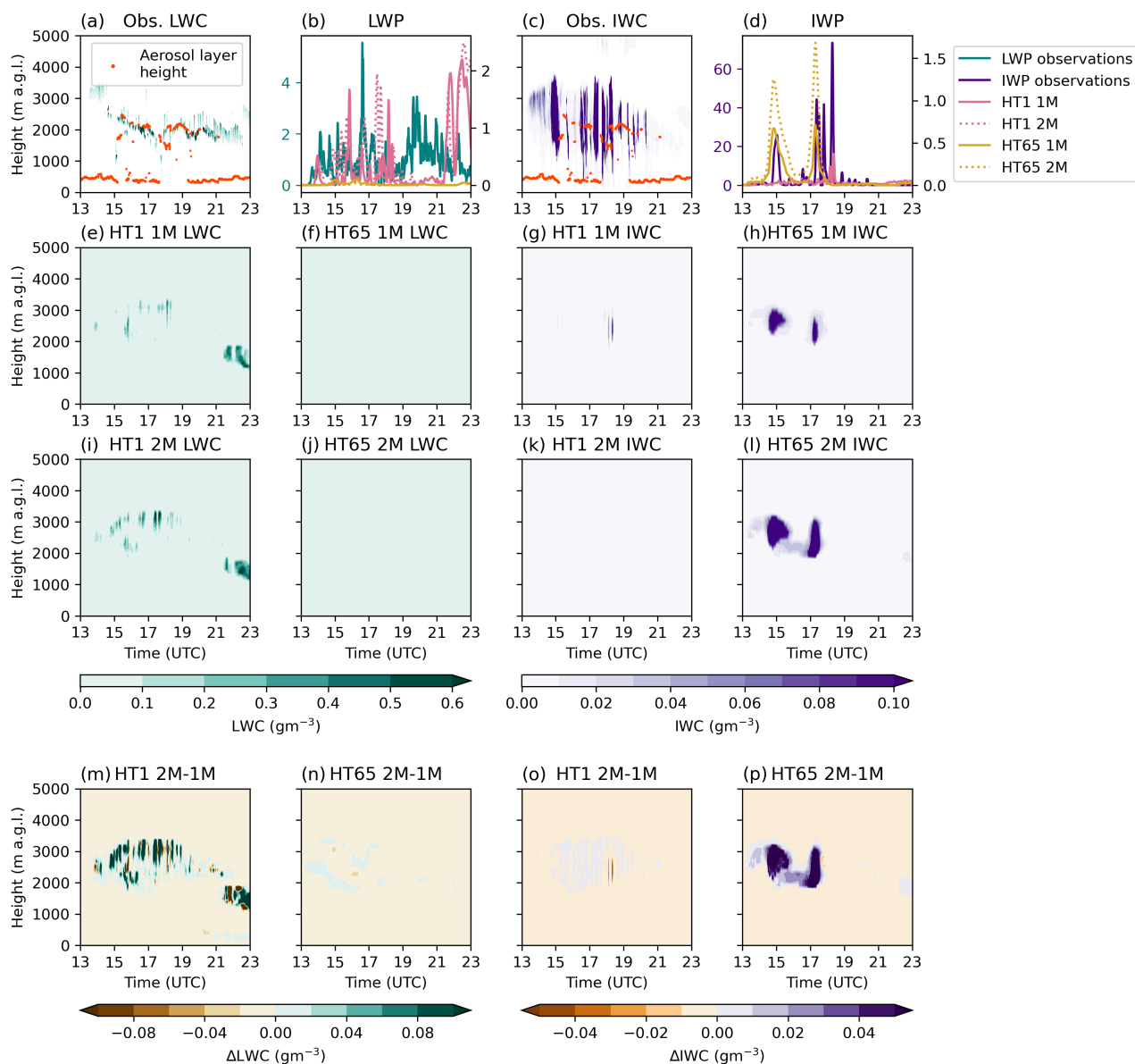
Figure 5. Overview of cloud characteristics for case study 31 Jan 2023. (a) and (c) show the liquid water content (LWC ( \text{g m}^{-3} )) and ice water content (IWC ( \text{g m}^{-3} )) based on the algorithm by Cloudnet with the aerosol layer height (orange dots) serving as a proxy for the boundary layer height. (e)-(l) show the model responses for both LWC and IWC for both resolutions (HT1 and HT65) and both bulk microphysics schemes (1M and 2M). (b) and (d) show the observed (left y-axis) and the simulated (right y-axis) LWP and IWP, respectively.
