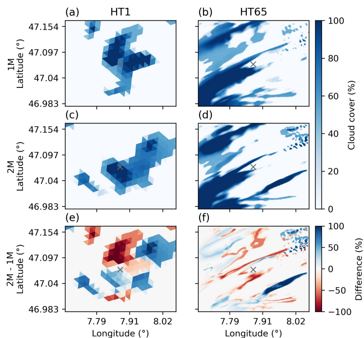
Figure 2. Comparison of fractional cloud cover (%) at \sim 2'500 m AGL for the case study on 20 Mar 2022 at 05:50 UTC (closest time step to the allsky camera snapshot in Fig. 1f) for HT1 (a, c, e) and HT65 (b, d, f) in 1M (first row) and 2M (second row) configuration, and their difference (2M - 1M, last row). "x" marks the CLOUDLAB field site. The domain of HT1 was zoomed in to show the same extent as the HT65 does.
