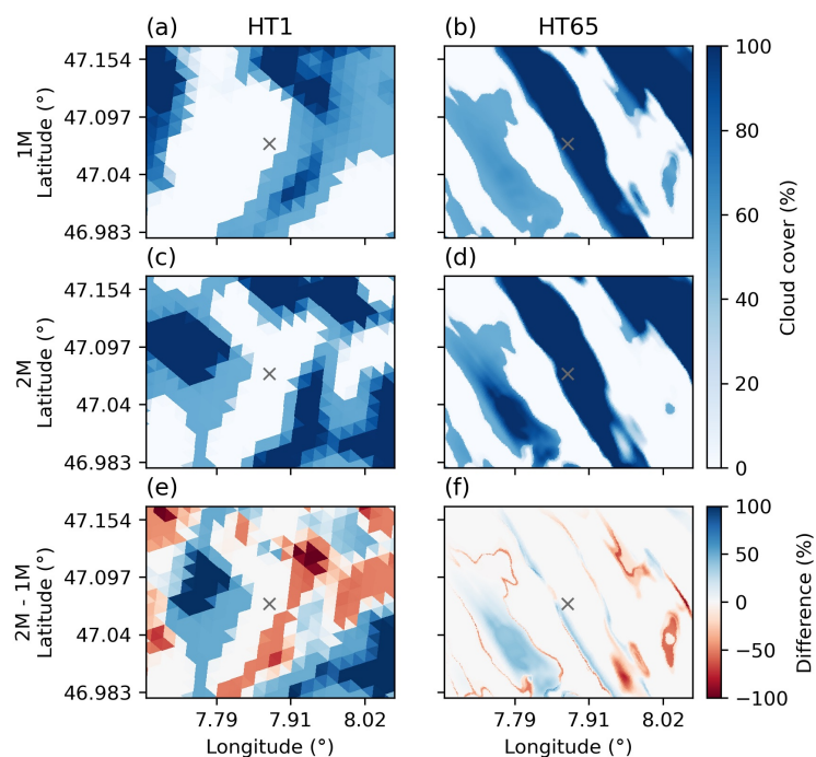
Figure 4. Comparison of fractional cloud cover (%) at \sim 2500 m AGL for the case study on 31 Jan 2023 at 15:30 UTC (closest time step to allsky camera snapshot in Fig. 1g) for HT1 (a, c, e) and HT65 (b, d, f) in 1M (first row) and 2M (second row) configuration, and their difference (2M - 1M, last row). "x" marks the CLOUDLAB field site. The domain of HT1 was zoomed in to show the same area as the HT65 does.
