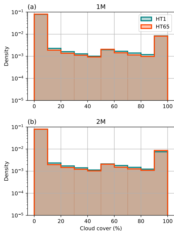
Figure B4. Probability density figures for the cloud cover (%) of HT1 (teal) and HT65 (red) with 1M (a) and 2M (b) over all five minute model output time steps and all height levels, where the cloud was present. The domain and time period included in this analysis is the same as in Fig. 8. The bin width is set to 10%.
