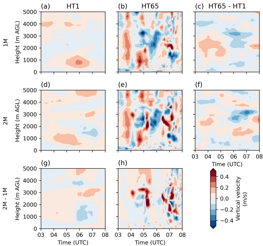
Figure A3. Hovmöller diagrams for vertical velocity ( \text{m s}^{-1} ) averaged over 10 min for HT1 and HT65 with 1M and 2M, respectively, for 20 Mar 2022. Last column shows the differences between the resolutions (HT65 - HT1), where HT65 was averaged over a running mean of 10 s to have the same time frequency as HT1. The last row shows the differences between 2M - 1M for both HT1 and HT65.
