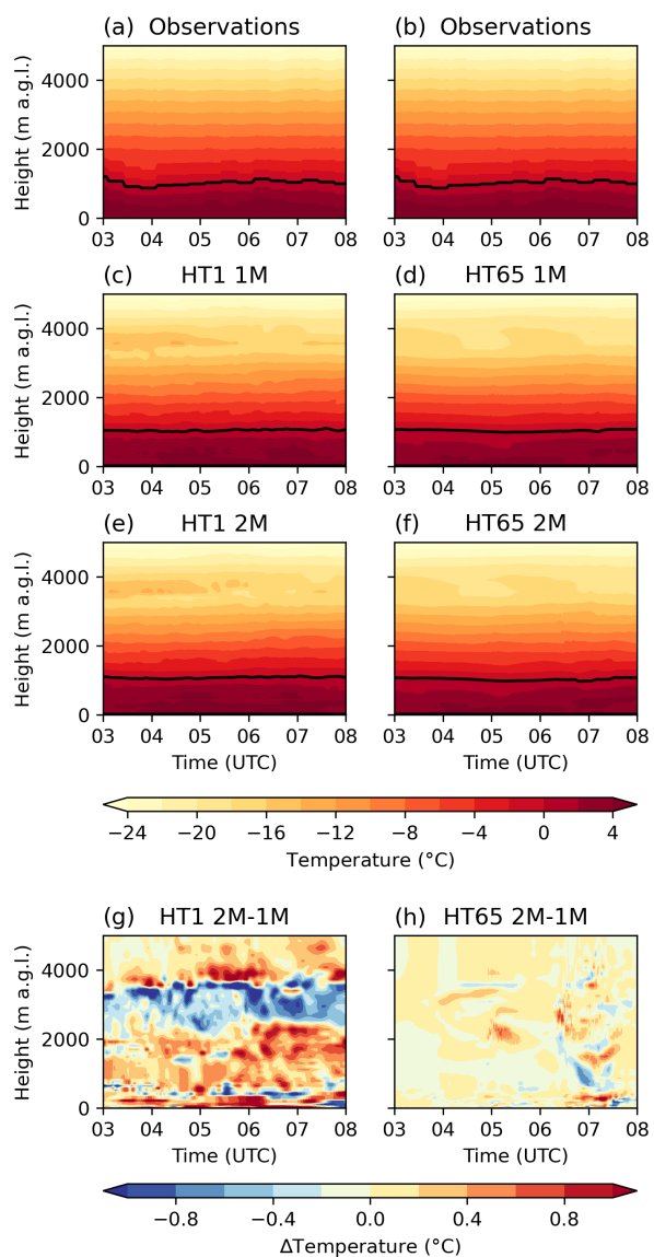
Figure A2. Case study 20 Mar 022: Hovmöller diagrams for temperature ( ^{\circ}\text{C} ) measured by a microwave radiometer (a, b) and simulated by the model for both resolutions (HT1 and HT65) and both cloud microphysics schemes (1M and 2M) (c-f). The black line indicates the 0^{\circ}\text{C} isotherm (black line). The last row (g, h) shows the differences between 2M and 1M for each resolution.
