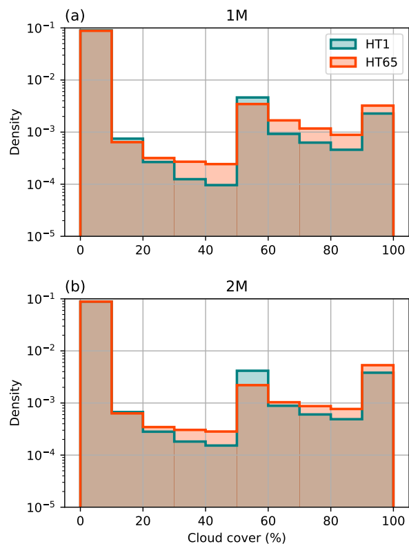
Figure A4. Probability density figures for the cloud cover (%) of HT1 (teal) and HT65 (red) with 1M (a) and 2M (b) over all five minute model output time steps and all height levels, where the cloud was present. The domain and time period included in this analysis is the same as in Fig. 5. The bin width is set to 10%.
