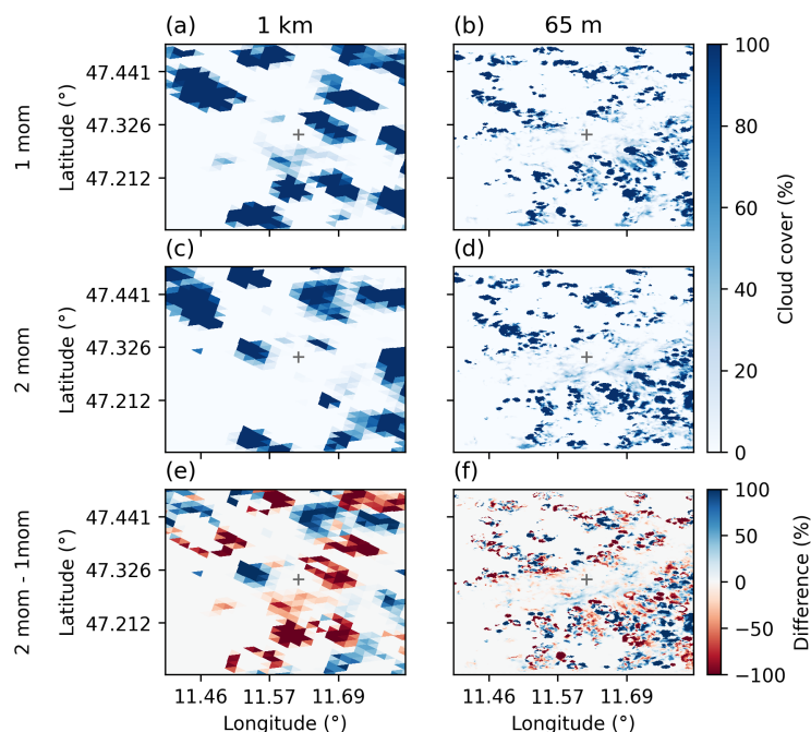
Figure 8. Comparison of cloud cover extent (%) at \sim 4000 m a.g. for the case study on 14 August, 2019 at 09:00 UTC (closest time step to Allsky camera snapshot in Fig. 1h) for CT1 (a, c, e) and CT65 (b, d, f) in 1M (first row) and 2M (second row) configuration, and their difference (2M - 1M, last row). "+" marks the CROSSINN field site. The domain of HT1 was zoomed in to show the same area as the HT65 does.
