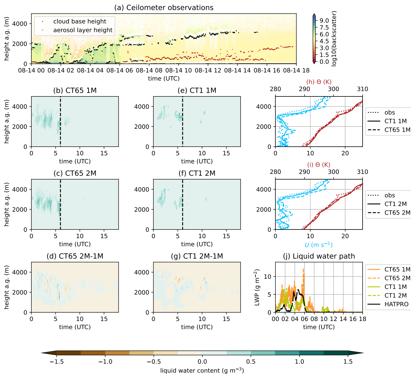
Figure 9. Aug 14, 2019, Inn Valley floor: (a) Ceilometer observations showing cloud backscatter (colors) with cloud base height (black dots) and aerosol layer height (red dots) determined by the instrument. Panels (b)–(g) Time series of model output of liquid water content from simulations CT65 1M (b, c) and CT1 1M (e, f) with 1M (b, e) and 2M (c, f), respectively. Panels (d) and (g) show the difference between the 2M and 1M schemes. The colorbar is valid for all panels showing LWC. Panels h–i) Vertical profiles of potential temperature (red) and horizontal wind speed (blue) of radiosonde observations (dots), CT1 (full lines), and CT65 (dashed lines) from 15:00 UTC. j) Liquid water path observations from HATPRO (black), and LWP model output from the respective simulations (colors).
