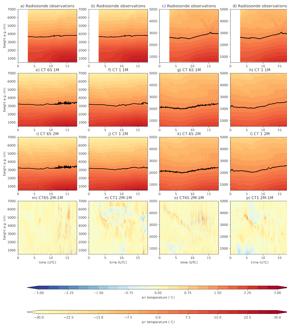
Figure B1. Time evolution of vertical profiles of the air temperature from radiosonde observations (panels (a)-(d)), and model output from the different horizontal resolutions and microphysics schemes ((f)-(l)), and their differences (panels (m)-(p)) from the two CT case studies at the valley floor, respectively. The black lines denotes the 0 °C line.
