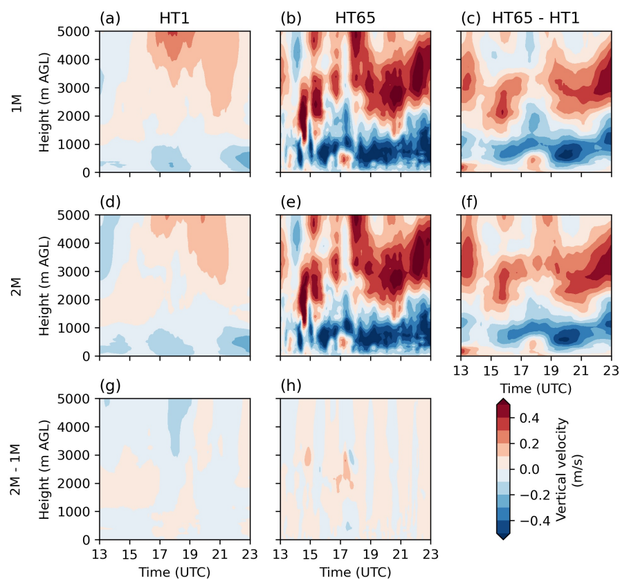
Figure A6. Hovmöller diagrams for vertical velocity ( \text{ms}^{-1} ) averaged over 10 min for HT1 and HT65 with 1M and 2M, respectively, for 31 Jan 2023. Last column shows the differences between the resolutions (HT65 - HT1), where HT65 was averaged over a running mean of 10 s to have the same time frequency as HT1. The last row shows the differences between 2M - 1M for both HT1 and HT65.
