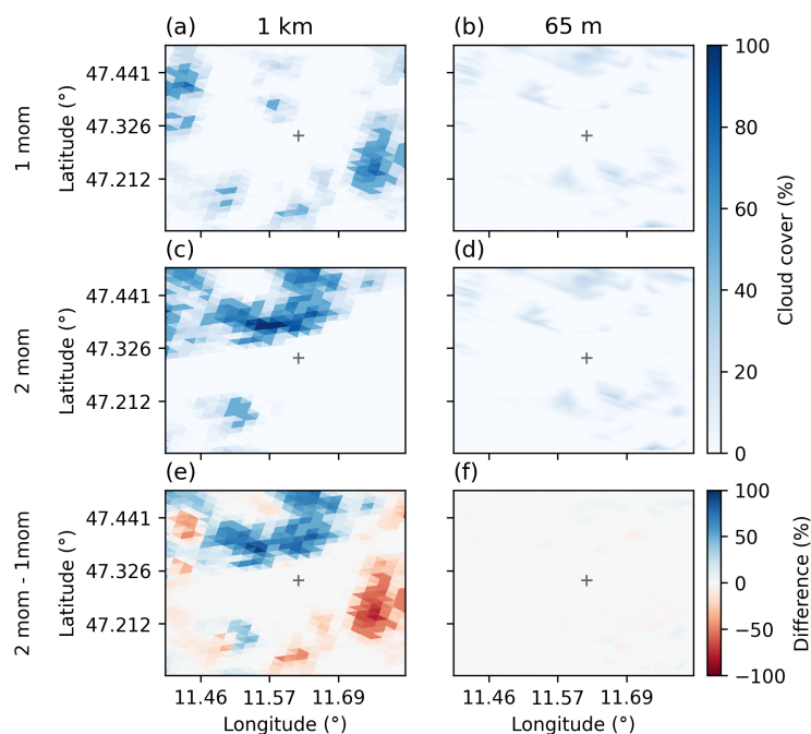
Figure 6. Comparison of cloud cover extent (%) at \sim 4'000 m AGL for the case study on 05 August, 2019 at 09:00 UTC (closest time step to Allsky camera snapshot in Fig. 1h) for CT1 (a, c, e) and HT65 (b, d, f) in 1M (first row) and 2M (second row) configuration, and their difference (2M - 1M, last row). "+" marks the CROSSINN field site. The domain of CT1 was zoomed in to show the same area as the HT65 does.
