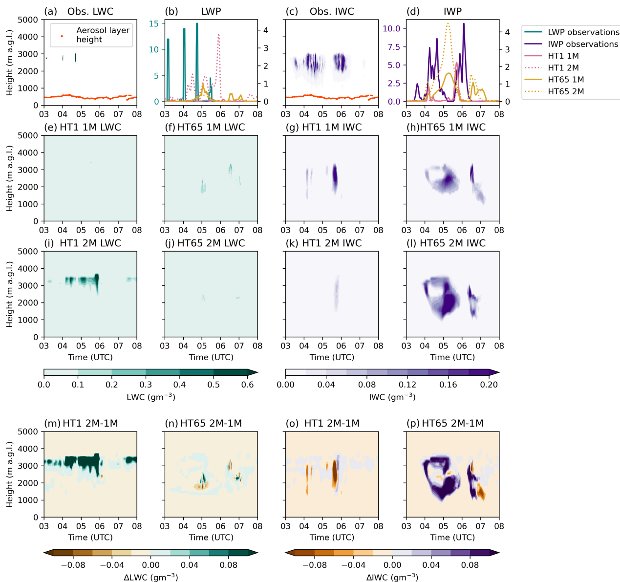
Figure 3. Overview of cloud characteristics for case study 20 Mar 2022. (a) and (c) show the liquid water content (LWC ( \text{g m}^{-3} )) and ice water content (IWC ( \text{g m}^{-3} )) based on the algorithm by Cloudnet with the aerosol layer height (orange dots) serving as a proxy for the boundary layer height. (e)–(l) show the model responses for both LWC and IWC for both resolutions (HT1 and HT65) and both bulk microphysics schemes (1M and 2M). (b) and (d) show the observed (left y-axis) and the simulated (right y-axis) LWP and IWP, respectively.
