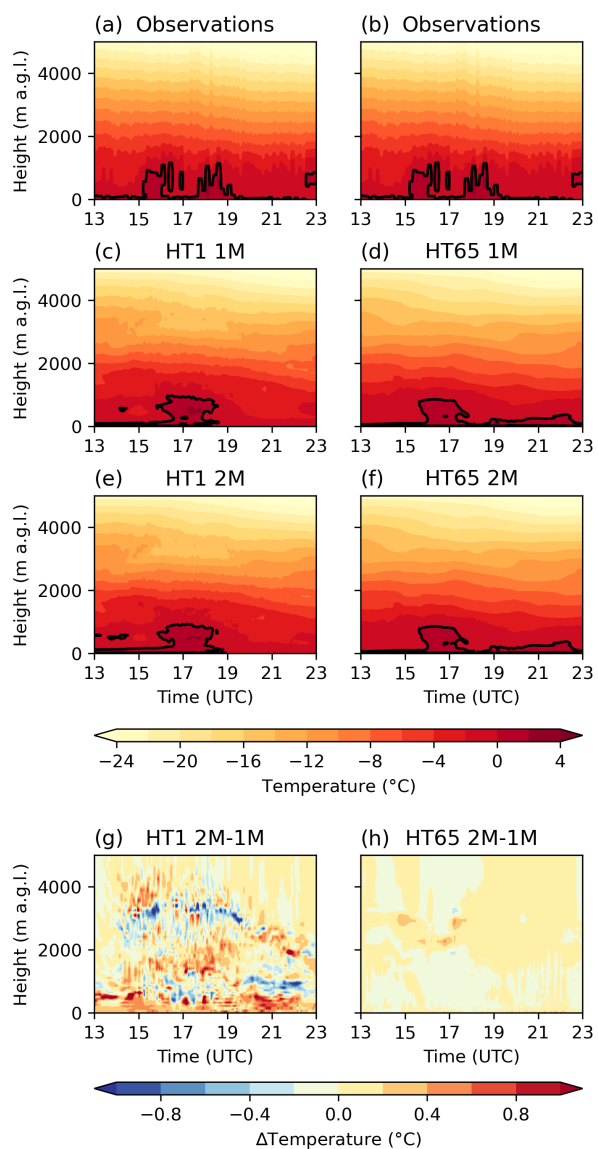
Figure A5. Case study 31 Jan 2023: Hovmöller diagrams for temperature ( ^{\circ}\text{C} ) measured by a microwave radiometer (a, b) and simulated by the model for both resolutions (HT1 and HT65) and both cloud microphysics schemes (1M and 2M) (c-f). The black line indicates the 0^{\circ}\text{C} isotherm (black line). The last row (g, h) shows the differences between 2M and 1M for each resolution.
