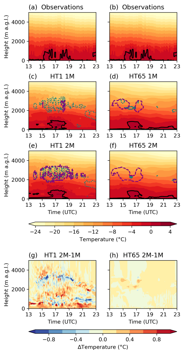
Figure B4. Case study 31 Jan 2023: Hovmöller diagrams for temperature ( ^{\circ}\text{C} ) measured by a microwave radiometer ( a , b ) and simulated by the model for both resolutions (HT1 and HT65) and both cloud microphysics schemes (1M and 2M) ( c-f ). The black line indicates the 0^{\circ}\text{C} isotherm (black line). The dashed purple line shows the \text{IWC} = 0.01 \text{ g m}^{-3} , while the dotted teal line shows the \text{LWC} = 0.01 \text{ g m}^{-3} . These serve as an indicator for the position of the cloud. The last row ( g , h ) shows the differences between 2M and 1M for each resolution.
