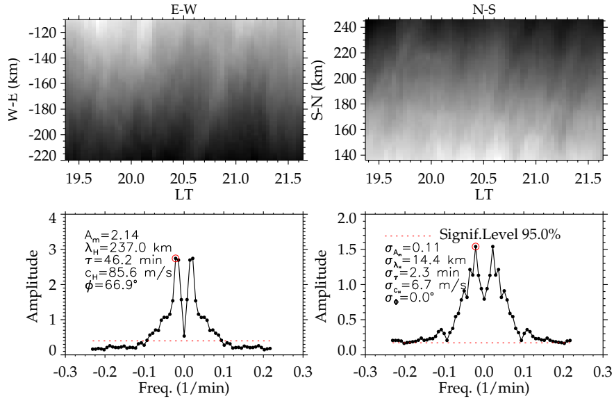
Figure A4. Result of OH emission layer keogram/spectral analysis of Event #02 with period of \tau = 46.20 \pm 02.30 min
