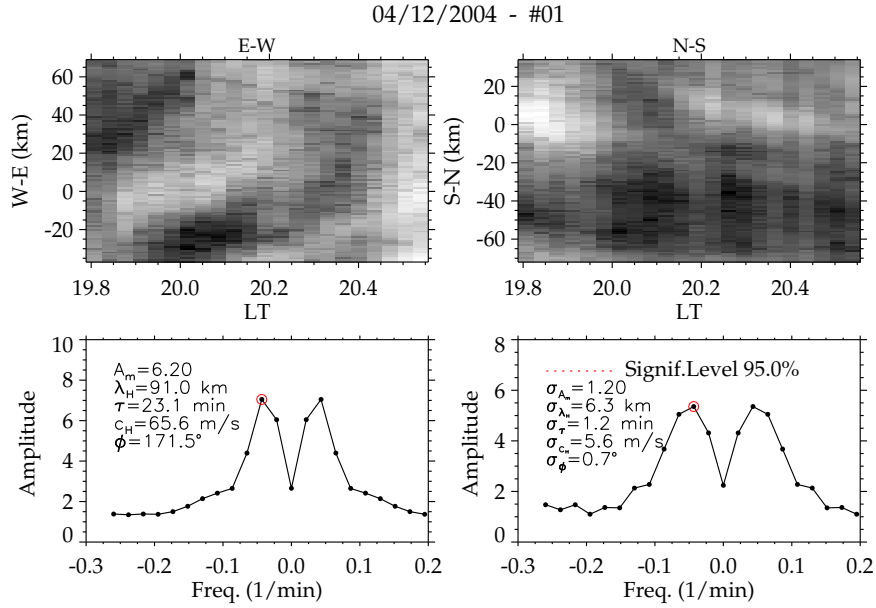
Figure A1. Result of OH emission layer keogram/spectral analysis of Event #01 with period, \tau = 23.10 \pm 01.20 \text{ min} .
