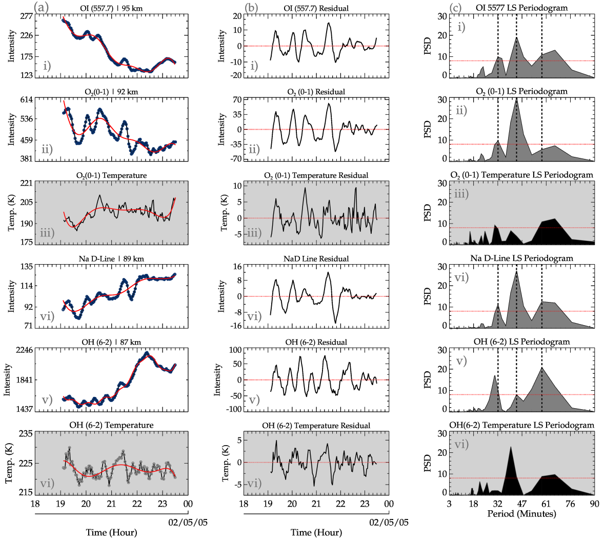
Figure 6. Figure 6 is similar to Figure 5 except for the event of 01/05/2005 between 18:30 and 23:30 UT.
