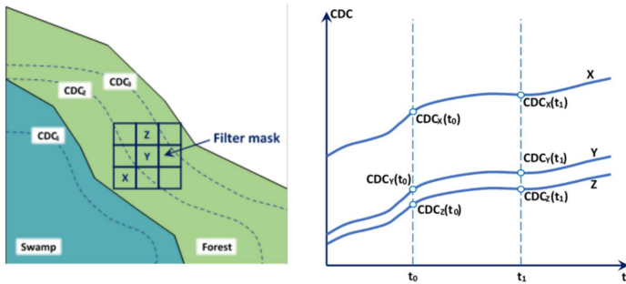
(a) An example of \text{CO}_2 source and sink location (b) An example of synchronous CDC changes over time
