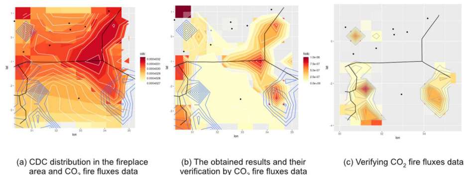
Figure A1: Spatial distributions of the CO 2 parameters and the obtained results of the CO 2 source area detection. A spatial CDC distribution in the area of the fireplace and its boundaries detection with the proposed method
