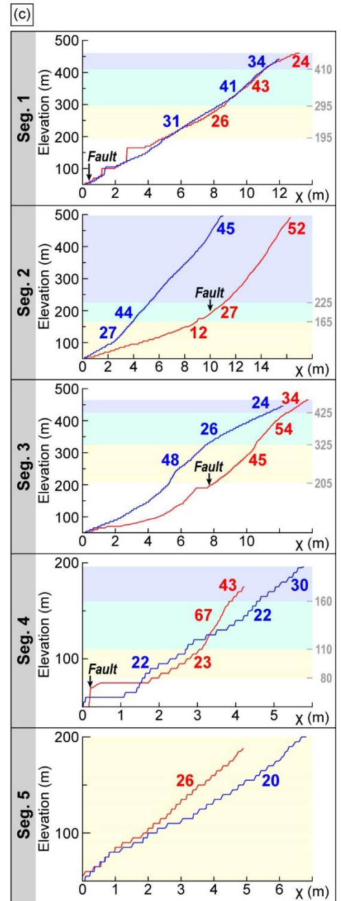
Figure 11: Our proposed segmentation of the UFZ, with values of topographic metrics analysed for each segment. (a) Segmentation of the UFZ proposed in this study. The locations of segment boundaries are the same as those marked in Fig. 7. The segment boundaries are marked with white bars, and the MDD of the TMR is marked with a solid white line. (b) Mean values and 1\sigma standard deviation of topographic metrics within each segment, normalised to the mean value of each index from the western flank. Topographic metrics on the western flank are in red, and those on the eastern flank are in blue. Symbols filled with black represent decoupled \chi indices. We performed Student's t-tests to compare these metrics between the western and eastern flanks. P-values exceeding the threshold of 0.05 (statistical significance of 95 %) are given in bold, which indicate that the mean values of the western- and eastern-flank are not statistically significantly different. (c) \chi -transformed profiles for one western-flank and one eastern-flank channel from each of the segments shown in Fig. 11a. The numbers represent ksn of each reach of channel. The profiles for channels on the western flank are plotted with a red line, and those on the eastern flank are plotted with a blue line.
