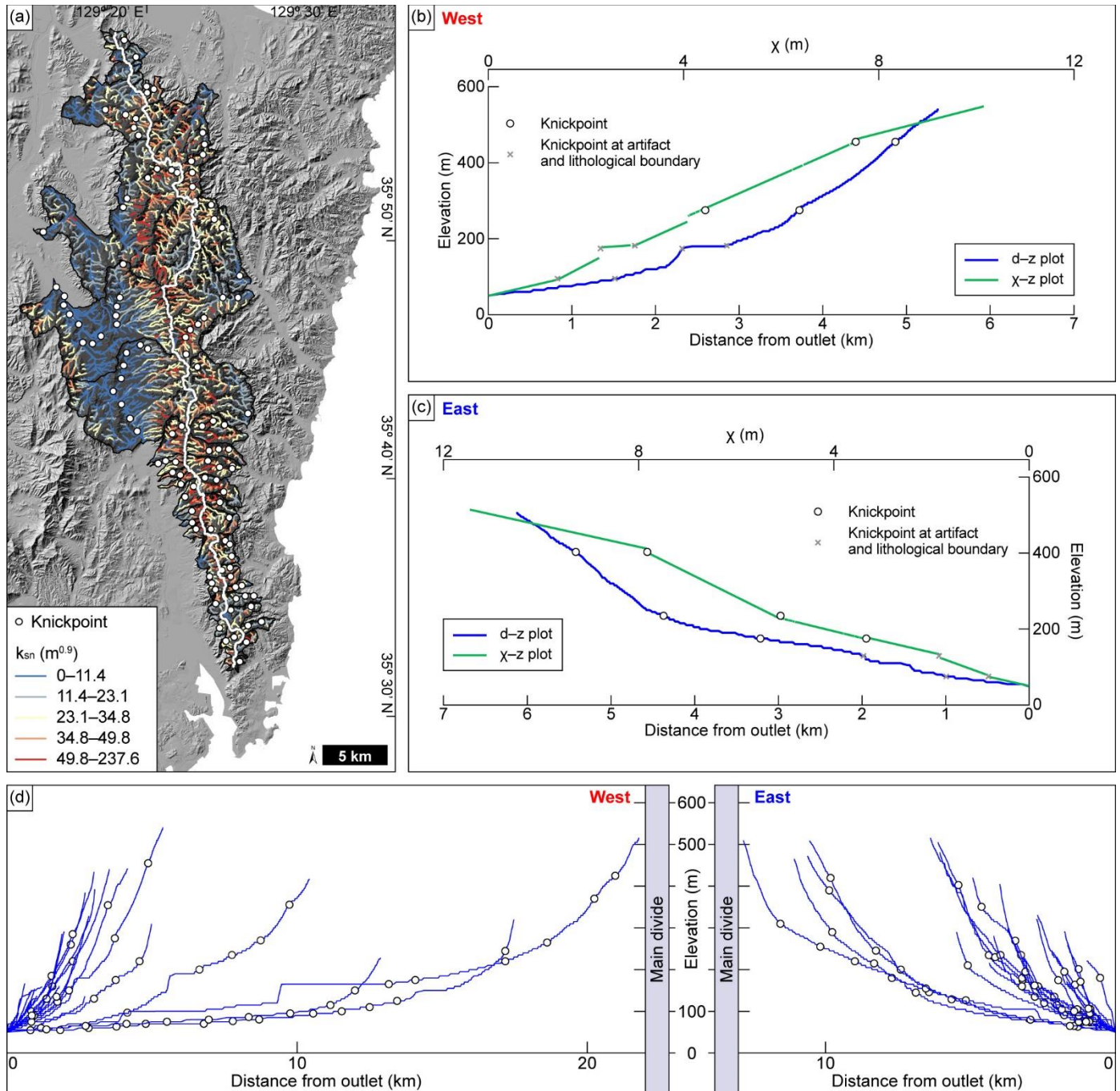
430 Figure 5: (a) Spatial distribution of knickpoints on trunk stream channels and map of normalised steepness index ( k_{sn} ) for the entire study area. A reference concavity index ( \theta_{ref} ) of 0.45 was applied to calculate values of k_{sn} . Knickpoints (white circle) were detected after excluding artefacts and lithological boundaries. (b and c) Plots of d-z (blue) and \chi-z (green) for a stream on each of the western and eastern flanks, respectively, where d is distance from the outlet and z is elevation. Knickpoints detected at artefacts and lithological boundaries are marked with grey crosses. The locations of these channels are marked in Fig. 3b. (d) Longitudinal profiles and knickpoints of all trunk channels in the study area. Knickpoints detected at the artefacts and lithological boundaries are excluded.
