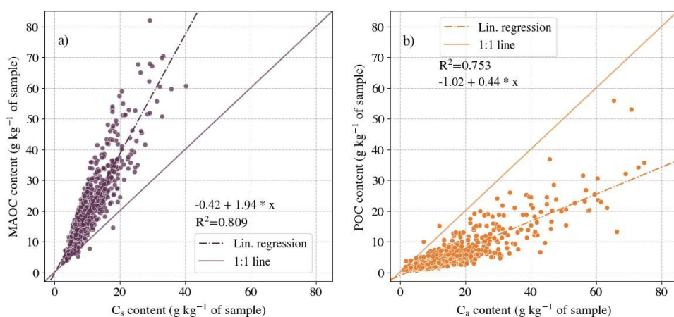
245 Figure 1: Comparison of the quantities of the more stable and more labile fractions for the physical and thermal SOC fractionation schemes, with their correlation coefficient R^2 and linear regression. Panel (a) shows the quantities of MAOC plotted against C_s . Panel (b) shows the quantities of POC plotted against C_a . The dataset is the intersection dataset, i.e. samples for which thermal and physical data are available ( n = 843 ).
