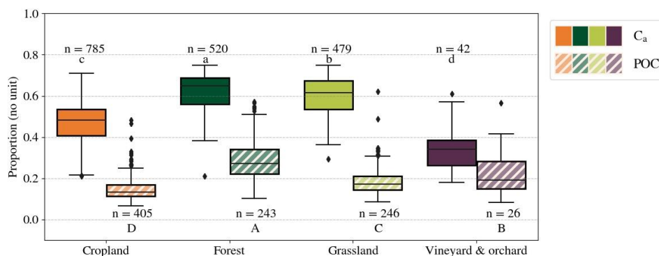
265 Figure 2: Proportion of the C_a and POC fractions depending on the land cover. The black line in each box is the median, the lower and upper edges of the black rectangle are the respective first (Q1) and third (Q3) quartiles, and the lower and upper whiskers are the maximum between the minimum value or the first quartile minus 1.5 times the interquartile range ( \max[\min; Q_1 - 1.5 \times (Q_3 - Q_1)] ) and the minimum between the maximum or the third quartile plus 1.5 times the interquartile range ( \min[\max; Q_3 + 1.5 \times (Q_3 - Q_1)] ), respectively. Different letters indicate significant differences in the distribution of the values for the land covers according to a Kruskal–Wallis test ( p < 0.05 ) and a pairwise Wilcoxon rank sum test ( p < 0.05 ); lowercase letters are used for C_a and uppercase for POC.
