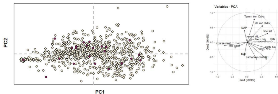
690 Figure A1: Score of the 993 samples on axes 1 and 2 of the principal component analysis on 14 pedoclimatic parameters: clay, fine silt, coarse silt, fine sand and coarse sand contents; pH in water; carbonate content; mean annual temperature and mean annual precipitation; Tamm and Mehra–Jackson iron oxyhydroxide contents; exchangeable calcium, magnesium and potassium ions. Samples with an organic carbon yield between 0.7 and 1.3 are plotted in light yellow, whereas samples with an organic carbon yield <0.7 or >1.3 are plotted in dark red.
