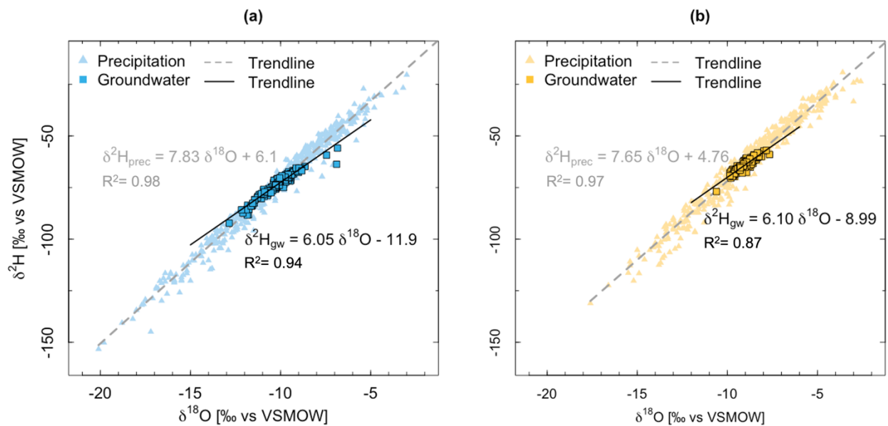
205 Figure 3: Regional Meteoric Water Lines (triangles) and Groundwater Lines (squares) (a) in the southern alpine and (b) northern Main regions.
