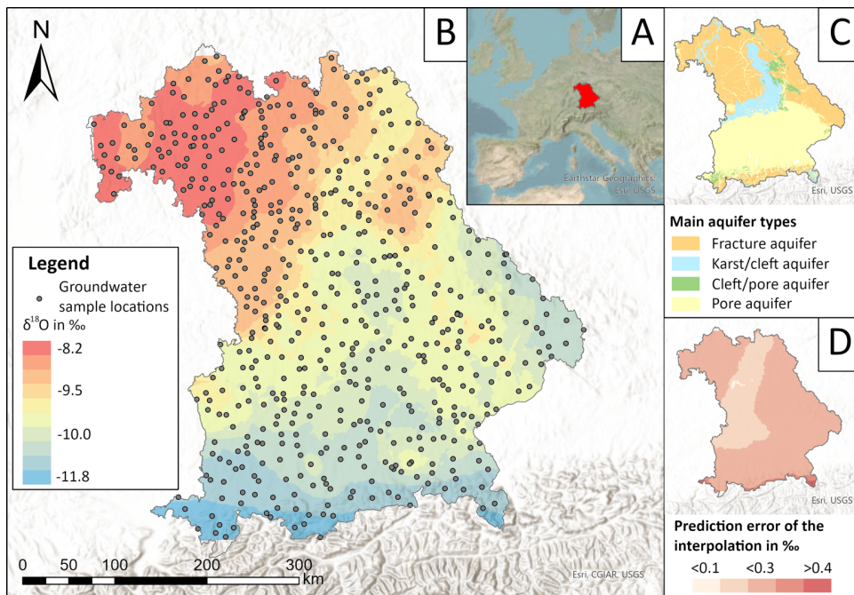
Figure 1: (a) Location of the study area in Europe. groundwater \delta^{18}\text{O} isoscape with sample locations. (b) Groundwater \delta^{18}\text{O} isoscape (obtained with empirical Bayesian Kriging) with sample locations. Location of the study area in Europe. (c) Main hydrogeological units in Bavaria according to the Hydrogeological Map for Germany (HÜK250) provided by the German Federal Institute for Geosciences and Natural Resources (Bundesanstalt für Geowissenschaften und Rohstoffe and Staatlichen Geologischen Dienste, 2019). (d) Standard error of the interpolation prediction in ‰.
