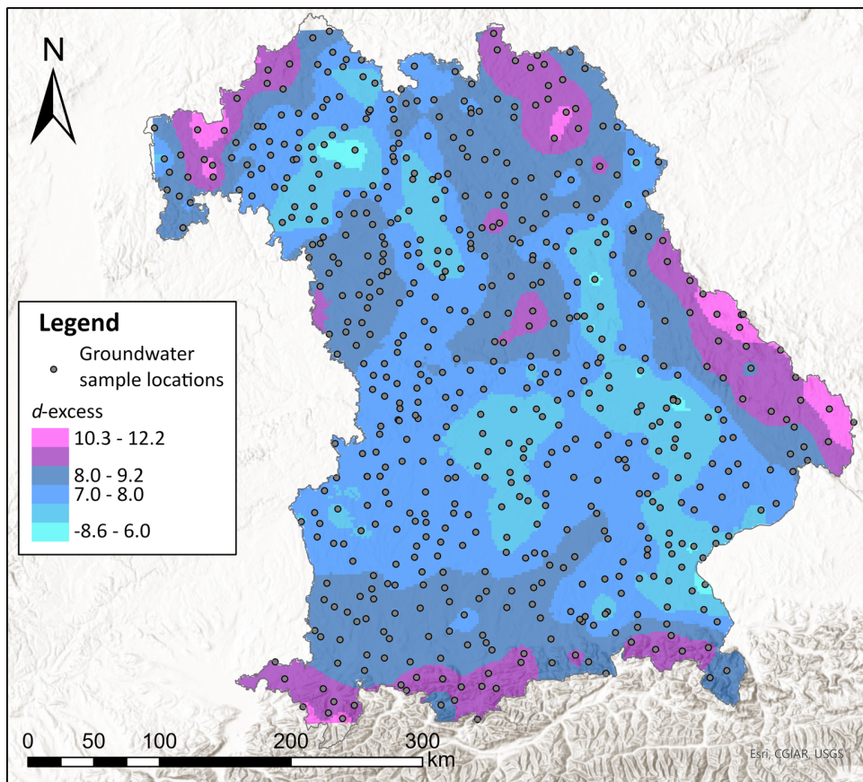
Figure 4: Interpolated d_{\text{-excess}} -values in Bavarian groundwaters (obtained with empirical Bayesian Kriging) with sample locations.
