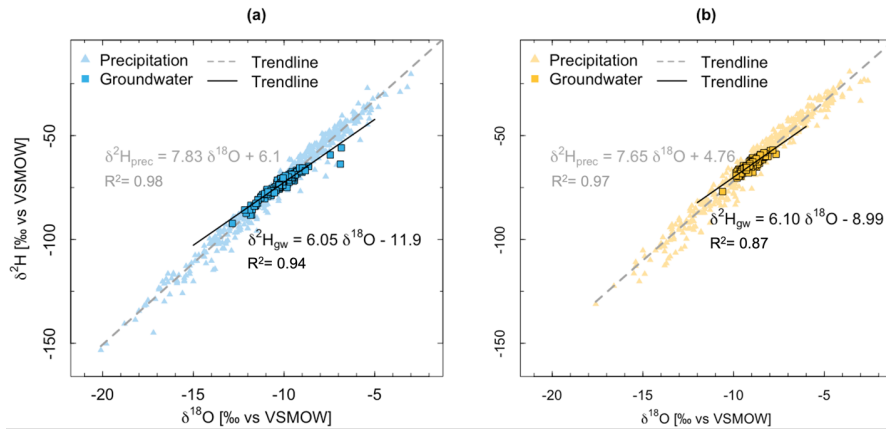
Figure 3: Regional Meteoric Water Lines (triangles) and Groundwater Lines (squares) and precipitation (triangles) (a) in the southern alpine and (b) northern Main regions.
