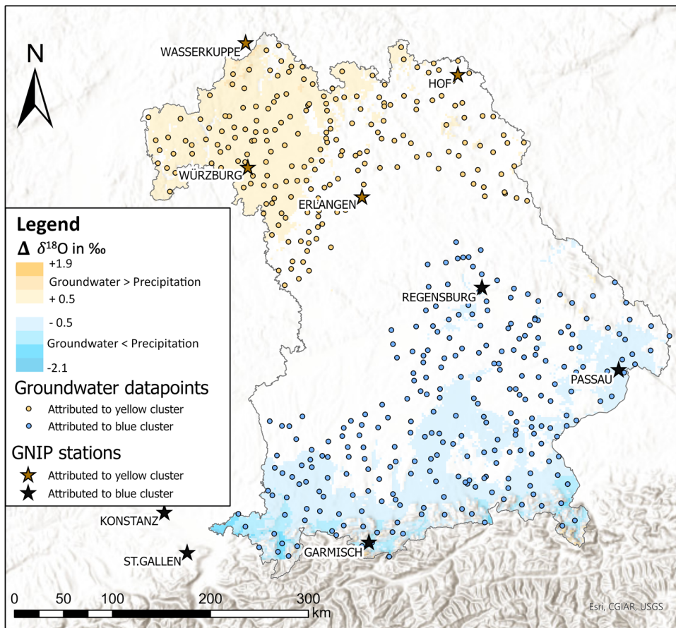
Figure 2: Differences between \delta^{18}\text{O} values groundwater and precipitation isoscapes ( \Delta\delta ). Areas with differences smaller than |0.5 \text{ ‰}| are transparent. The yellow and blue areas mark the clusters with groundwater–precipitation differences >|0.5 \text{ ‰}| . The groundwater sampling points and GNIP stations attributed to one cluster according to Sect. 2.5 are also shown.
