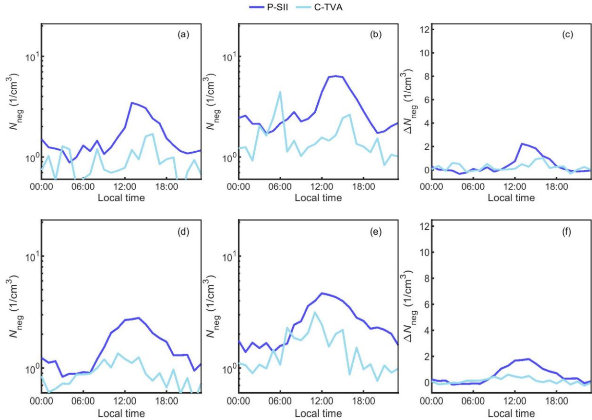
Figure 8. The 50 th percentile (a) and 75 th percentile (b) of negative intermediate ions ( N_{\text{neg}} ) at 350 2.0-2.3 nm at each hour and the daily fluctuations of N_{\text{neg}} (c) for the peatland and coastal area in spring (MAM) and the corresponding 50 th percentile, 75 th percentile, and normalized concentration for median values in summer (JJA), (d), (e), (f), respectively.
