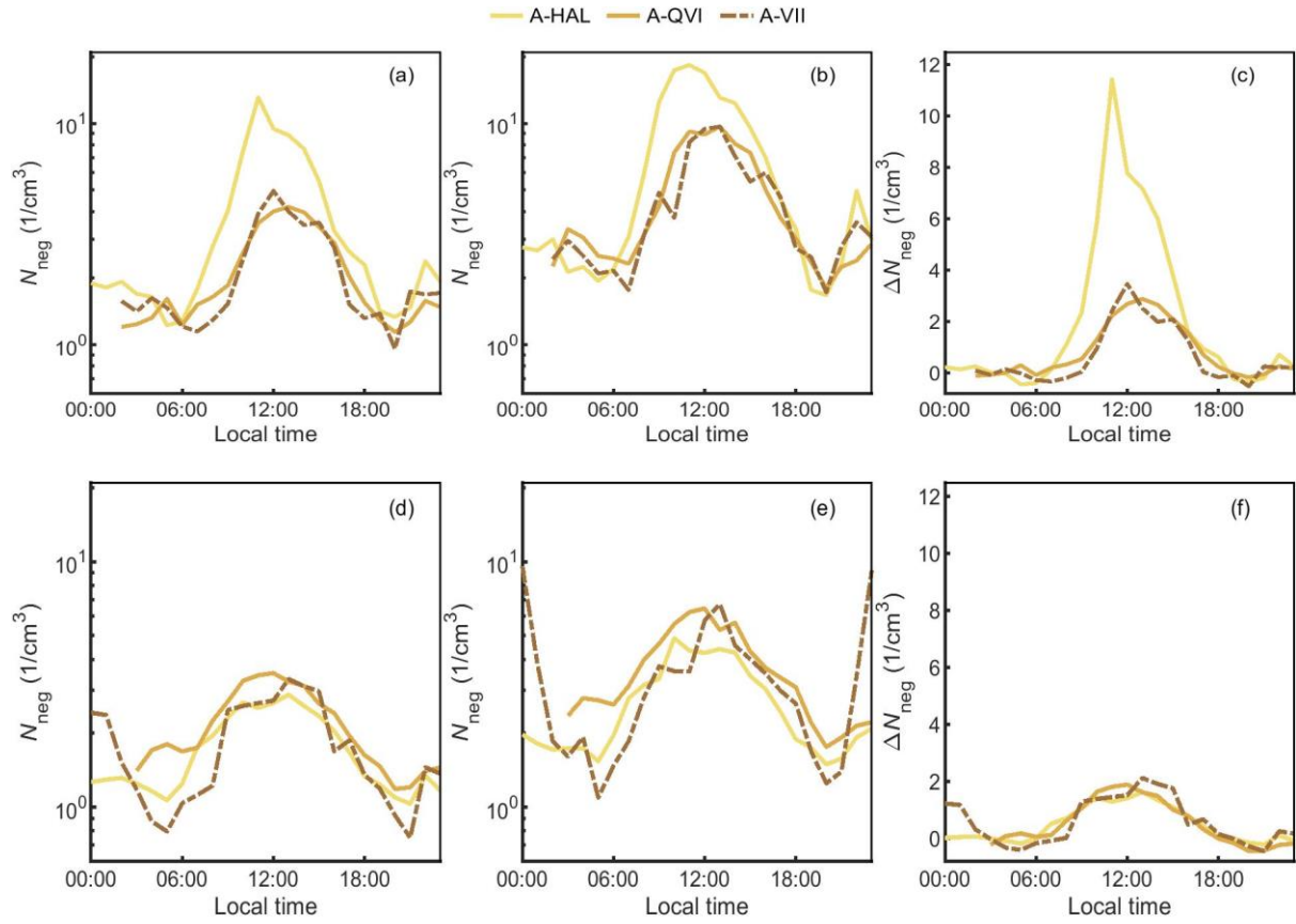
345 Figure 7. The 50 th (a) and 75 th percentile (b) of negative intermediate ions ( N_{\text{neg}} ) at 2.0-2.3 nm at each hour and the daily fluctuations of N_{\text{neg}} (c) for the agricultural fields in spring (MAM) and the corresponding 50 th percentile, 75 th percentile and normalized concentration for median values, (d), (e), (f), in summer (JJA), respectively.
