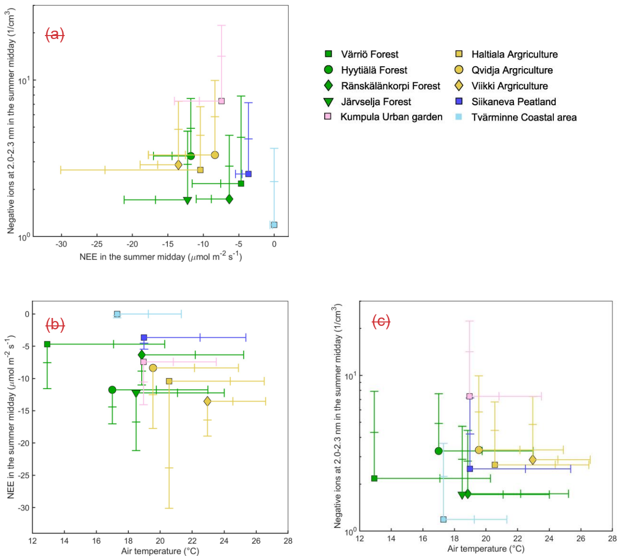
Figure 9. Comparison between the median NEE, median negative intermediate ions at 2.0-2.3 nm, and median air temperature at midday in summer between the sites. The error bars are the 10 th and 25 th percentile for NEE, the 75 th and 90 th percentile for the negative intermediate ions, and the 75 th and 90 th percentile for the air temperature at each site.
