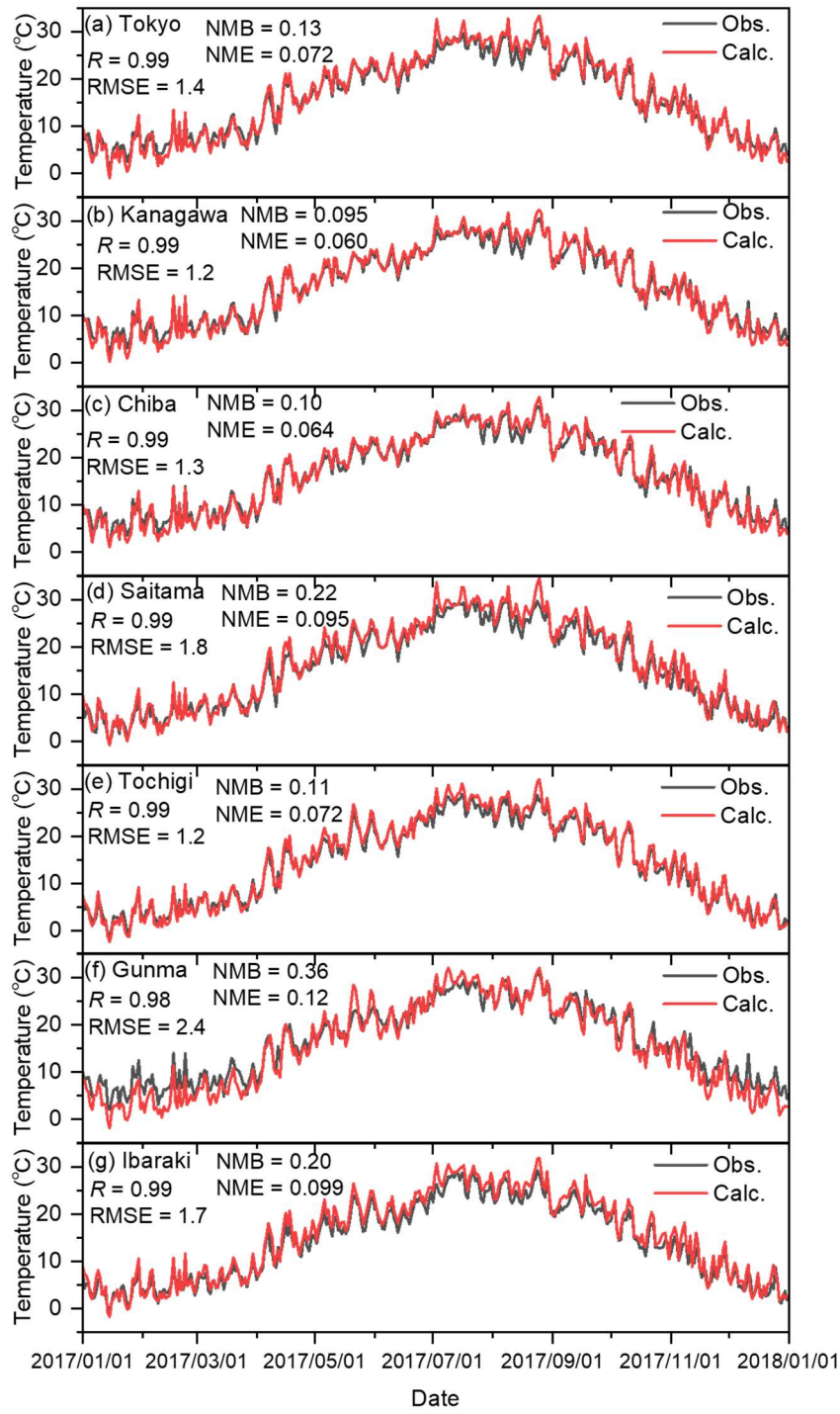
Figure C1: Comparison of observed (Obs.) and calculated (Calc.) daily averaged ground-temperatures in (a) Tokyo, (b) Kanagawa, (c) Chiba, (d) Saitama, (e) Tochigi, (f) Gunma, and (g) Ibaraki.
