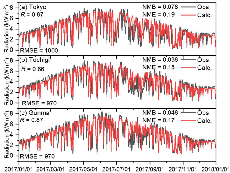
660 Figure C4: Comparison of observed (Obs.) and calculated (Calc.) daily total solar radiation in (a) Tokyo, (b) Tochigi, and (c) Gunma.
