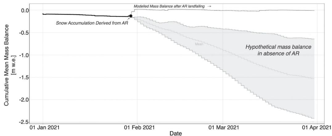
Figure 8. Hypothetical glacier mass balance scenarios for the 2020/21 hydrological year without occurrence of the summer- January-2021 AR event . The graph shows a zoom for the period January to March 2021. The uncertainty range corresponds to 1\sigma .
