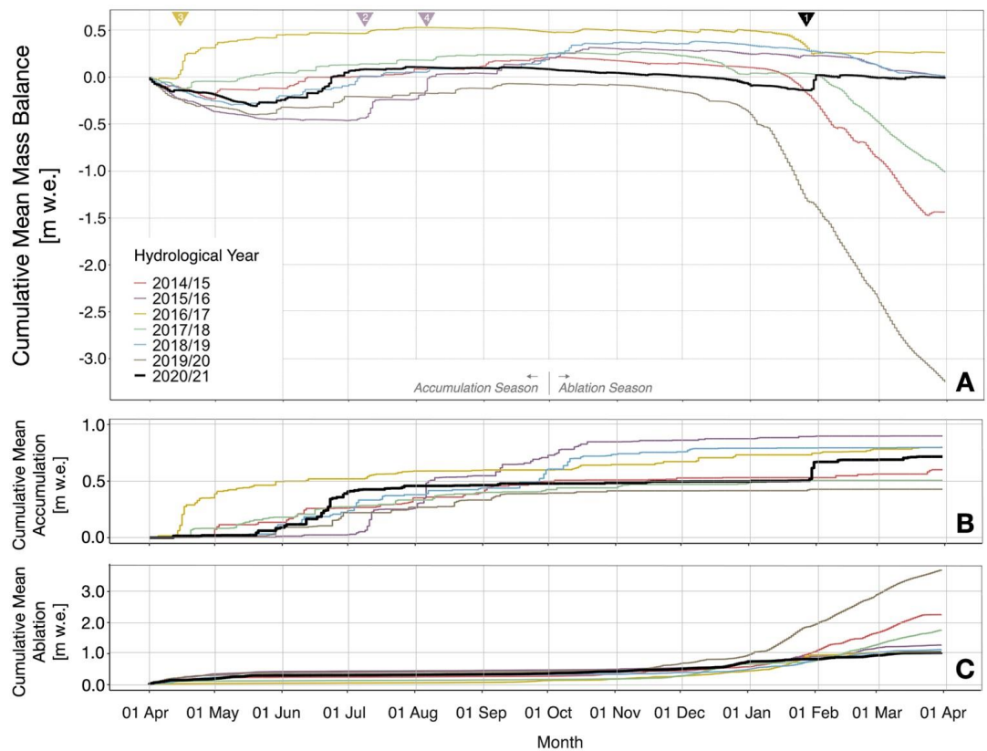
375 Figure 7. a) Cumulative spatial mean mass balance, b) cumulative spatial mean accumulation, and c) cumulative spatial mean ablation of the Olivares Alfa Glacier for seven hydrological years (from 2014/15 to 2020/2021). Triangles at the top are AR events mentioned in the text with their respective categories. Note that vertical axis scales are different
