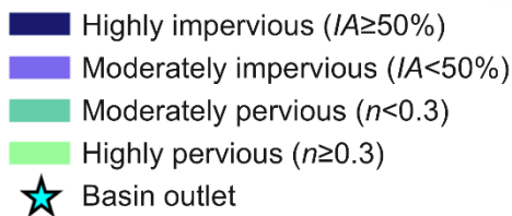
Figure 6. Case-study basins from the EPAE, MO, and VA homogenous regions in the TIA-HCIU plane, considering a) HCIU ( n ) and b) HCIU ( CN ), respectively. Seven specific basins (c–i) are used as examples to visualize the sensitivity of HCIU to different spatial arrangements of LULC patches, even for basins with similar TIA ; a simplified, four-category LULC classification is adopted, as indicated in the legend.
