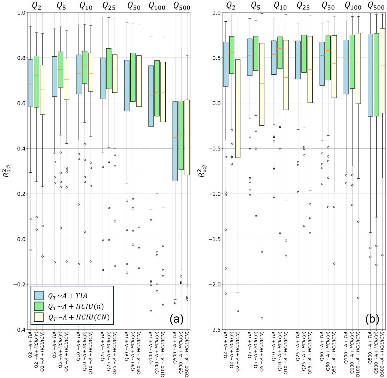
615 Figure 8. Boxplots of test errors for 1) the benchmark Q_T \sim A + TIA , 2) Q_T \sim A + HCIU(n) , and 3) Q_T \sim A + HCIU(CN) models, when they are fitted and blind-tested on distinct basin subsets, for the a) EPAE and b) MO homogenous regions, respectively (see this same plots for VA in Appendix D). For each boxplot, filled bars represent error values between the first and the third quartiles, the upper (lower) whisker extends from the third (first) quartile by adding (subtracting) 1.5 times the interquartile range, and any outliers beyond the whiskers are marked as circles.
