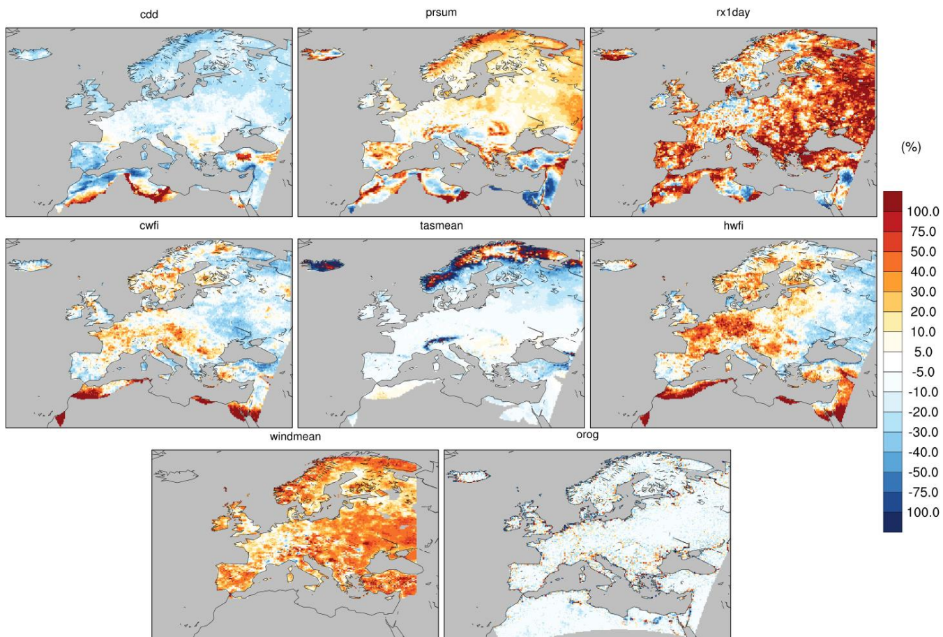
Figure 1: Percentage bias for climate indices from the 310-year Ens6 (see Table 3) compared to E-OBS dataset (1980-2010).
