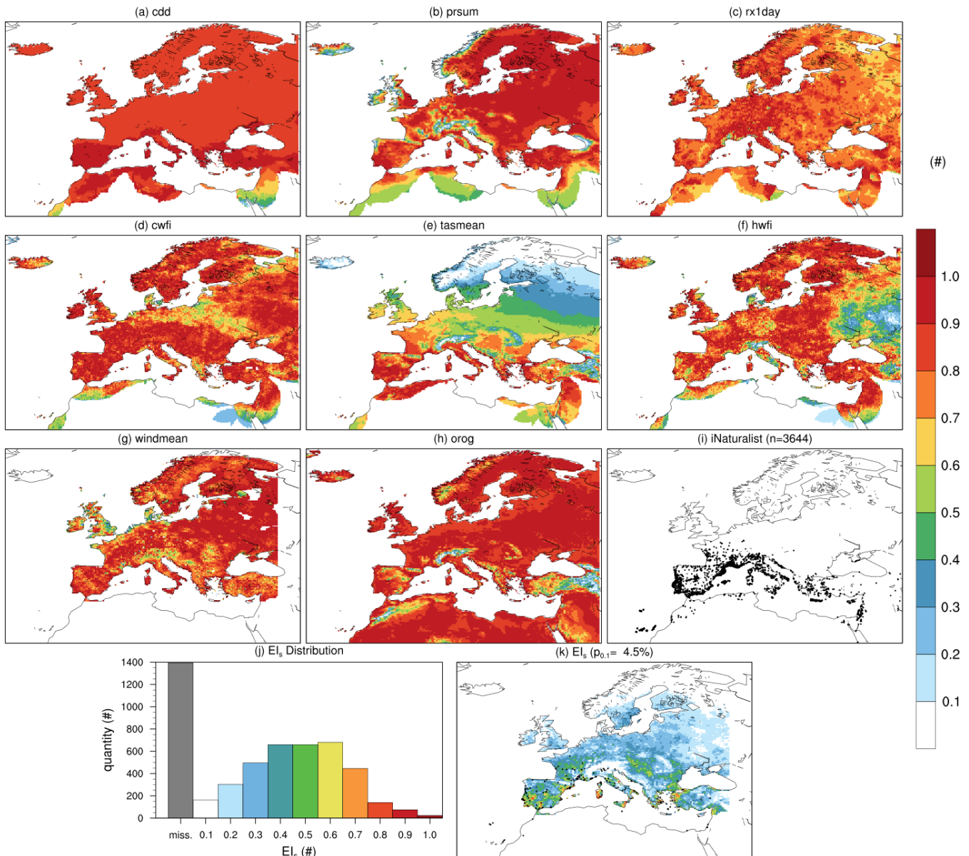
275 Figure 3: The EIs product and components for Spilostethus pandurus according to the 1980-2010 E-OBS dataset. (a-h) The climate indices expressed in terms of affinity to Spilostethus pandurus . (i) The observation points (iNaturalist) and quantity, n , applied. (j) The distribution of EI_s values, including the number of points from the original dataset that could not be applied (“miss.”). (k) The spatial distribution of EI_s , including the points less than 0.1 (quantified with percentage p_{0.1} ).
