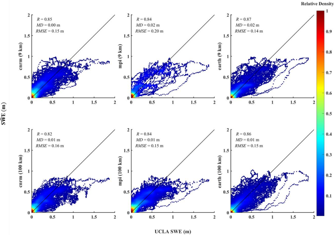
Fig.6. A density scatter plot in California from 2005 to 2010 compares in-situ data locations (Table 3) from UCLA SWE images to the downscaled SWE (S \hat{W}E ) values. The solid black line represents the 1:1 line. The displayed metrics include the correlation coefficient (R), mean difference (MD), and Root-Mean-Squared Error (RMSE). Only data with SWE values greater than 10 mm are included in the comparison.
