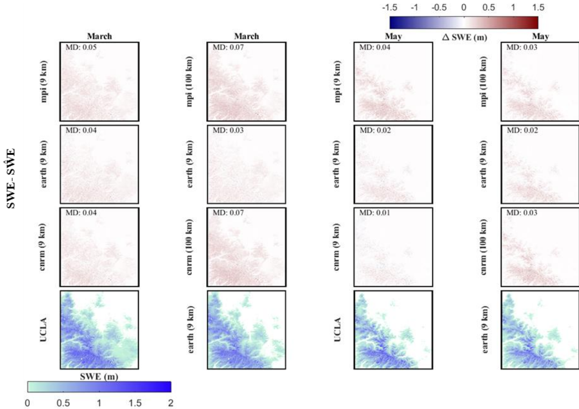
Fig. 9. Spatial assessment of the downscaling. The first three rows represent the mean difference between UCLA SWE and downscaled SWE ( SWE - \hat{SWE} ) over California throughout the 6-year testing period (2005-2010) for two months (March and May). The last row represents the averaged reference SWE (UCLA SWE) or averaged downscaled SWE ( \hat{SWE} ) throughout the 6-year testing period (2005-2010) for two different months (March and May). The evaluation metric includes Mean Difference (MD).
