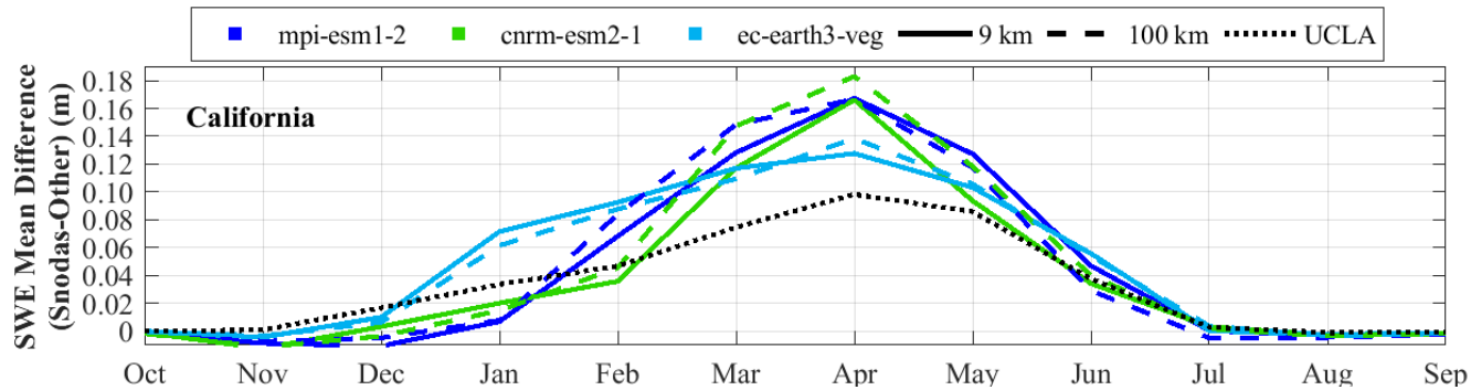
Fig. 10. The average mean difference of SWE over California for the 6-year testing period (2005-2010) compares UCLA SWE (black dotted line) and downscaled SWE ( \hat{SWE} ) data (blue and green lines) against SNODAS. The \hat{SWE} data, derived from different climate models, are represented by distinct colors: light blue for 'ec-earth3-veg', green for 'cnrm-esm2-1', and dark blue for 'mpi-esm1-2'. Solid lines indicate estimates at a 9 km resolution, while dashed lines correspond to a 100 km resolution, distinguishing the spatial resolutions of the climate data.
