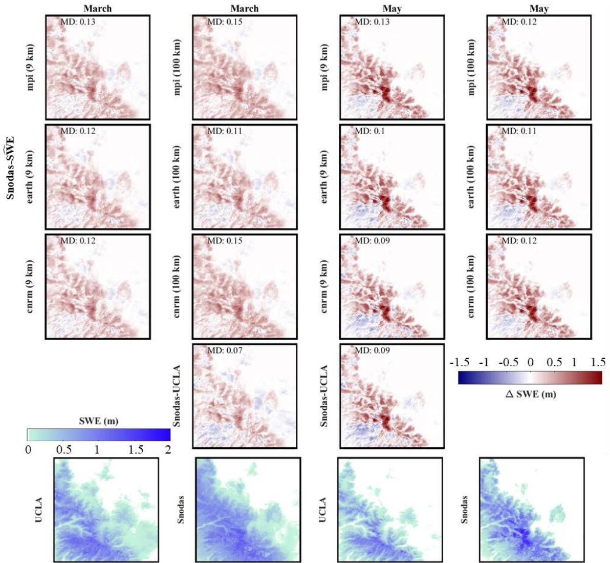
Fig. 11. Comparison with SNODAS data. The first four rows present the average difference between SNODAS and downscaled SWE (SWE) or UCLA SWE (SNODAS-SWE or SNODAS-UCLA) over California for March and May during the 6-year testing period (2005-2010). The last row compares the average UCLA SWE or SNODAS SWE over California for March and May during the same 6-year testing period (2005-2010). The evaluation metric includes Mean Difference (MD).
