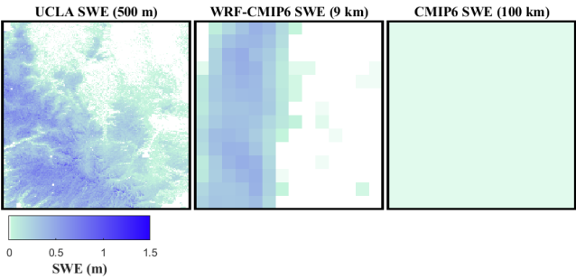
Fig. 4. Comparative illustration of SWE images highlighting the effect of spatial resolution on accuracy. Displayed from left to right are the UCLA SWE, WRF-CMIP6, and CMIP6 images captured over the California region (Fig. 3 (b), lon: -120 to -119, lat: 38 to 39) on January 8, 1995. Distinct variations between these images underscore the influence of scaling on image accuracy. Among the available models with resolutions of both 9 km and 100 km, we have selected three models for testing our methodology (Table 1Table 4). These models have been utilized in other studies (Thrasher et al., 2022; Kouki et al., 2022); Although our methodology is not limited to these models, they were selected merely as examples. Hereafter, we will refer to them as 'cnrm-esm2-1', 'ec-earth3-veg', and 'mpi-esm1-2'.
