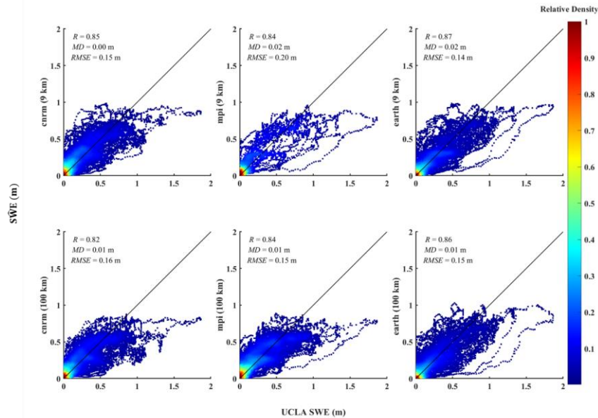
Fig.6. A density scatter plot in California from 2005 to 2010 compares in-situ data locations (Table 3 Table 3) from UCLA SWE images to the downscaled SWE ( \hat{SWE} ) values. The solid black line represents the 1:1 line. The displayed metrics include the correlation coefficient ( R ), mean difference ( MD ), and Root-Mean-Squared Error ( RMSE ). Only data with SWE values greater than 10 mm are included in the comparison.
