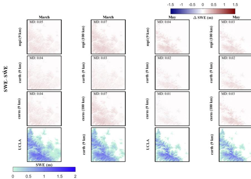
Fig. 9. Spatial assessment of the downscaling. The first three rows represent the mean difference between UCLA SWE and downscaled SWE (SWE- SWE) over California throughout the 6-year testing period (2005-2010) for two months (March and May). The last row represents the averaged reference SWE (UCLA SWE) or averaged downscaled SWE (SWE) throughout the 6-year testing period (2005-2010) for two different months (March and May). The evaluation metric includes Mean Difference (MD).
