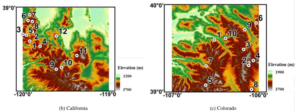
Fig. 3. a) Map of elevation (in meters) across the Western United States, highlighting two regions of interest (red squares). b) Map of elevation and locations of in-situ sites in the Sierra Nevada, California .c) Map of elevation and locations of in-situ sites in the Upper Colorado River Basin, Colorado.
