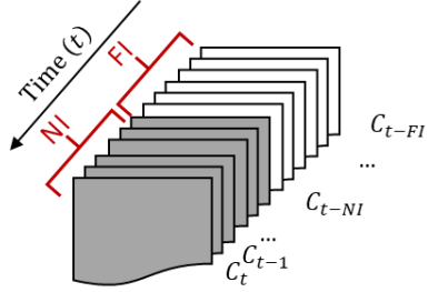
Fig. 1. Illustration of the definition of Near (shown in gray) and Far (shown in white) daily intervals for climate variables, highlighting the Far Temporal Interval (FI) and Near Temporal Interval (NI) of Climate Data at a Specific Time ( C_t ).
