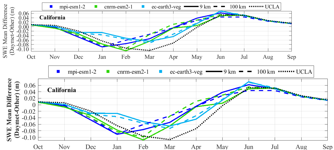
Fig.-12. Same as Fig. 910, but for comparison against the Daymet data.
