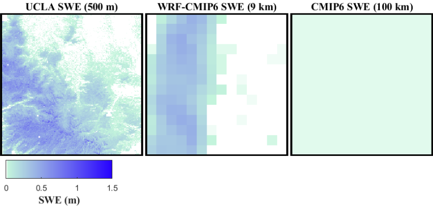
Fig. 4 . Comparative illustration of SWE images highlighting the effect of spatial resolution on accuracy. Displayed from left to right are the UCLA SWE, WRF-CMIP6, and CMIP6 images captured over the California region (Fig. 23 (b), lon: -120 to -119 , lat: 38 to 39) on January 8, 1995. The Distinct variations between these images underscore the influence of scaling on image accuracy.
