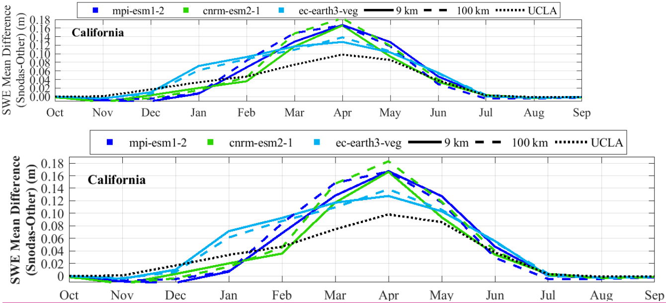
Fig. 10. The average mean difference of SWE over California for the 6-year testing period (2005-2010) compares UCLA SWE (black dotted line) and downscaled SWE (SWE) data (blue and green lines) against SNODAS. The SWE data, derived from various different climate estimators/models, are identified in the legend represented by their names and associated distinct colors: light blue for 'ec-earth3-veg', green for 'cnrm-esm2-1', and dark blue for 'mpi-esm1-2'. Within each color group, line styles distinguish the spatial resolutions of the climate data: Solid lines indicate climate estimators estimates at a 9 km resolution, while dashed lines represent climate estimators at correspond to a 100 km resolution, distinguishing the spatial resolutions of the climate data.
