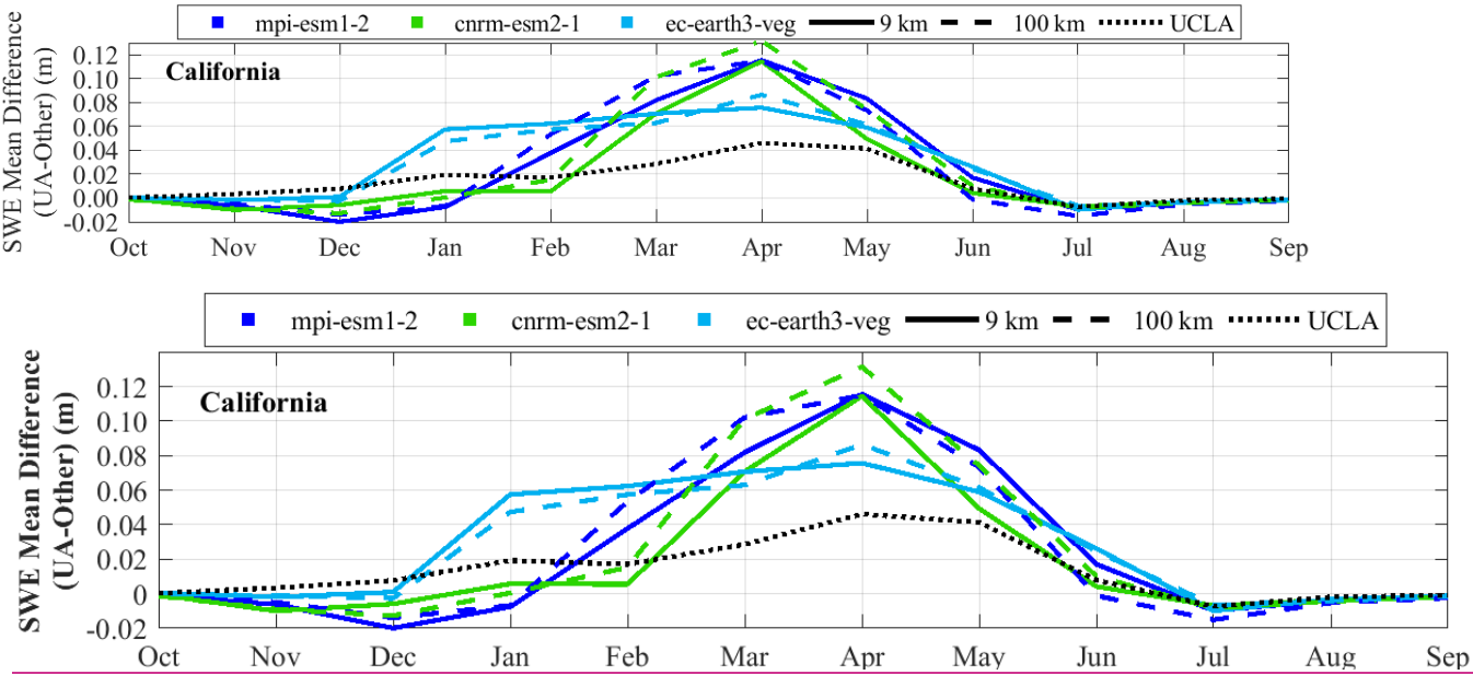
Fig. -14. Same as Fig. 910, but for comparison against the University of Arizona (UA) data.
