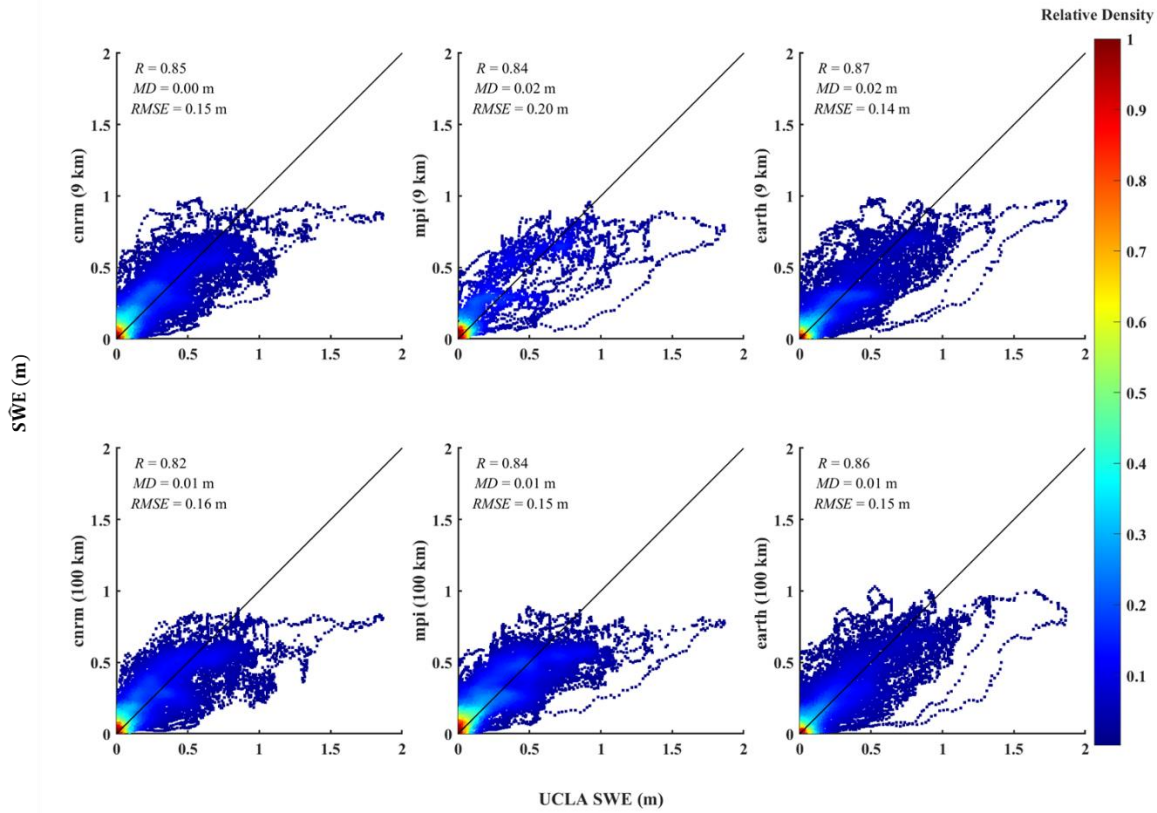
Fig. 6. A density scatter plot in California from 2005 to 2010 compares in-situ data locations (Table 3) from UCLA SWE images to the downscaled SWE ( \hat{SWE} ) values. The solid black line represents the 1:1 line. The displayed metrics include the correlation coefficient ( R ), mean difference ( MD ), and Root-Mean-Squared Error ( RMSE ). Only data with SWE values greater than 4 mm are included in the comparison.
