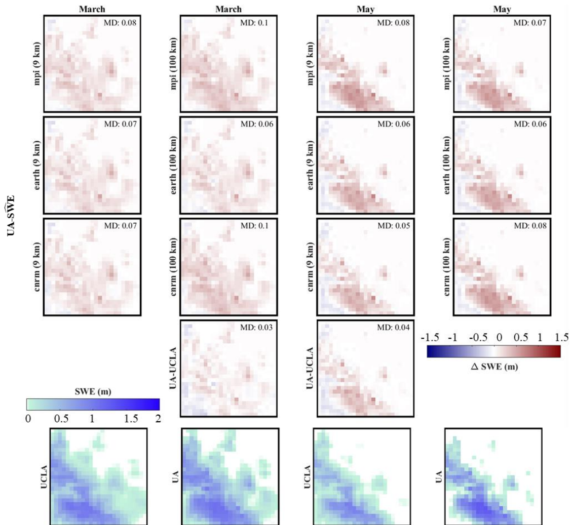
Fig. 15. Same as Fig. 4011, but for comparison against the University of Arizona (UA) data.
