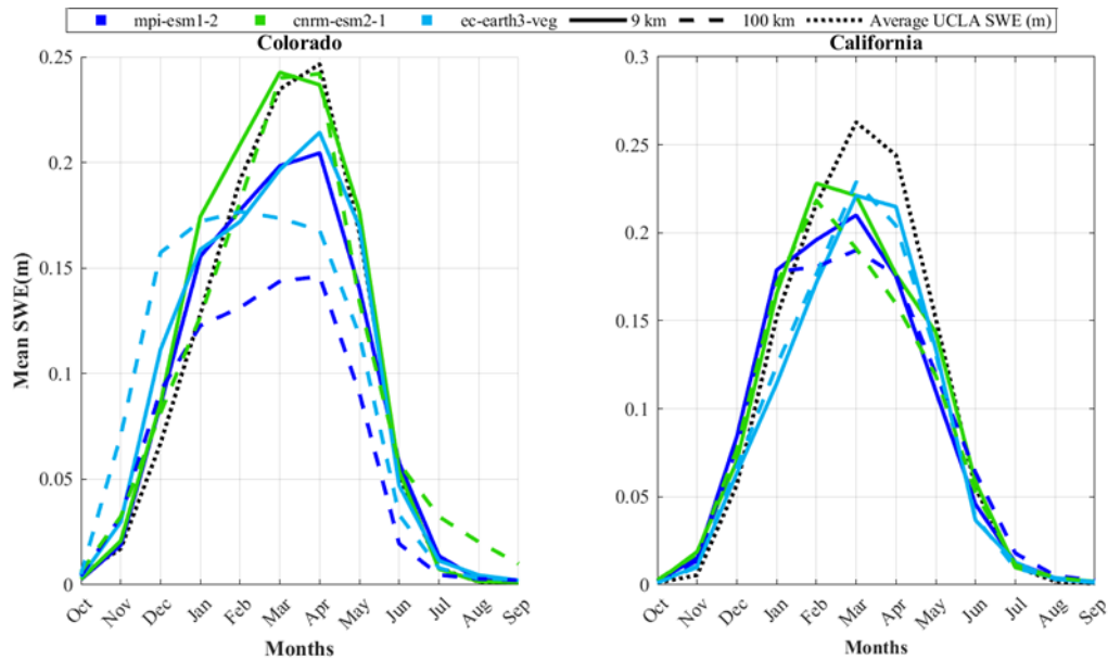
Fig. 7. The average of the UCLA SWE (black dotted line, reference) and the downscaled SWEs (SWE; blue and green lines) for each area over the six-year period from 2005 to 2010. For each area, the three climate models used in the downscaling are represented by a unique color: light blue for 'ec-earth3-veg', green for 'cnrm-esm2-1', and dark blue for 'mpi-esm1-2'. Within each color group, line styles indicate the spatial resolution of the climate data: solid lines correspond to results based on a 9 km climate estimators resolution, and dashed lines represent results based on a 100 km climate estimators resolution. The dotted black line represents the average UCLA SWE, which is the reference.
