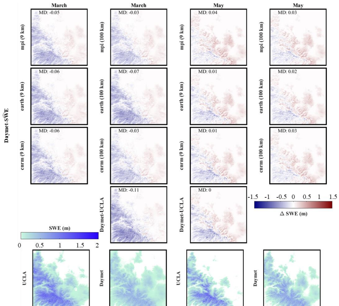
Fig. -13. Same as Fig. 4011, but for comparison against the Daymet data.
