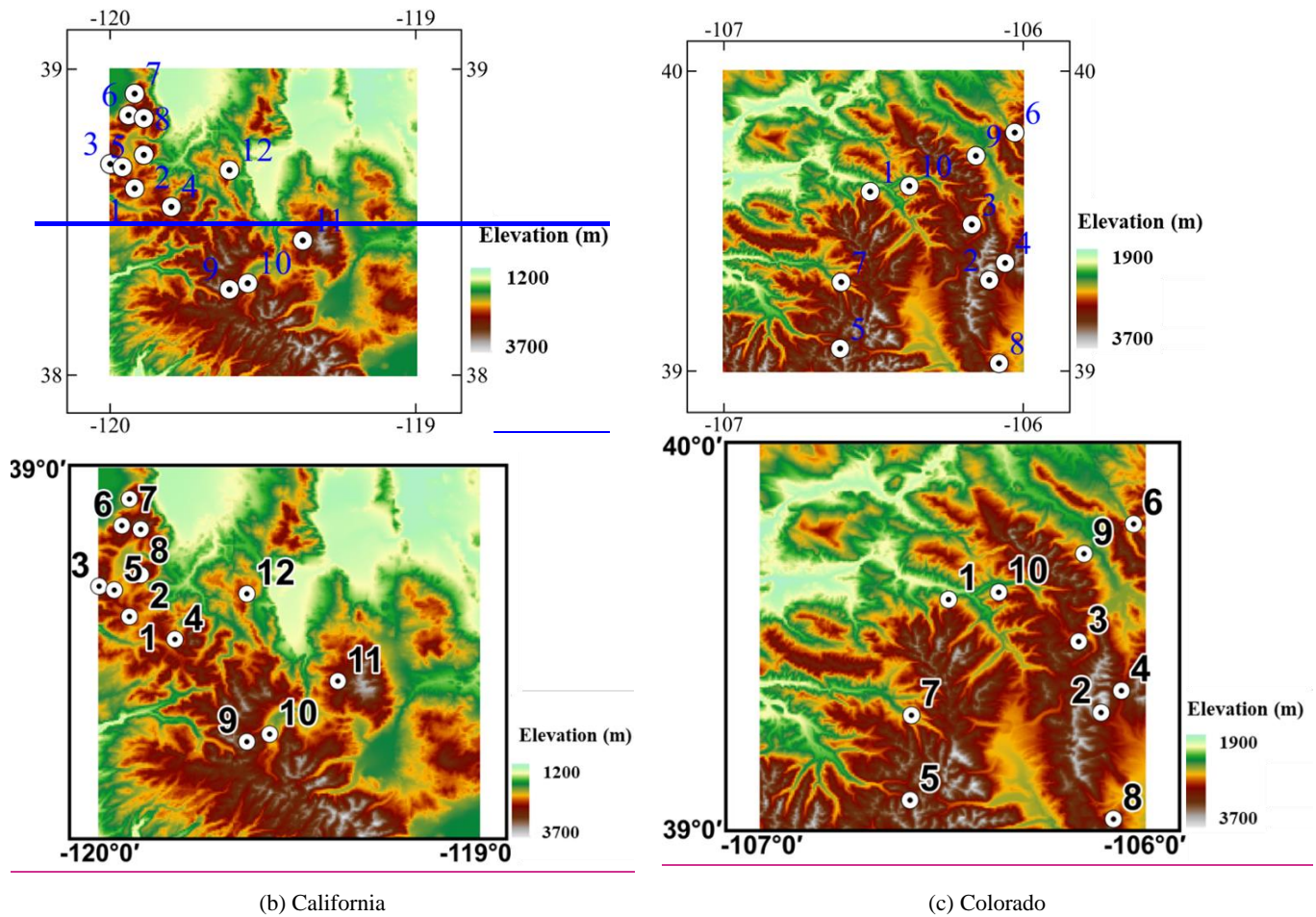
Fig. 3. a) Map of elevation (in meters) across the Western United States, highlighting two regions of interest (red squares). b) Map of elevation and locations of in-situ sites in the Sierra Nevada, California. c) Map of elevation and locations of in-situ sites in the Upper Colorado River Basin, Colorado.
